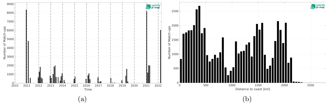
Figure 1: Number of match-ups between TSG (Polarstern) and SMOS SSS L2 v700 (ESA) SSS as a function of time (a) and as function of the distance to coast (b) over the Roaring Forties and Furious Fifties Pi-MEP region and for the full satellite product period.
