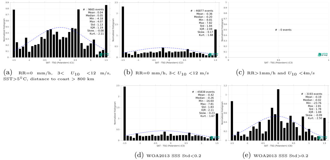
Figure 13: Normalized histogram of \Delta SSS (SMOS SSS L2 v700 (ESA) - TSG (Polarstern)) for 5 different subdatasets corresponding to: RR=0 mm/h, 3 < U_{10} < 12 m/s, SST > 5°C, distance to coast > 800 km (a), RR=0 mm/h, 3 < U_{10} < 12 m/s (b), RR > 1mm/h and U_{10} < 4 m/s (c), WOA2013 SSS Std < 0.2 (d), WOA2013 SSS Std > 0.2 (e).
