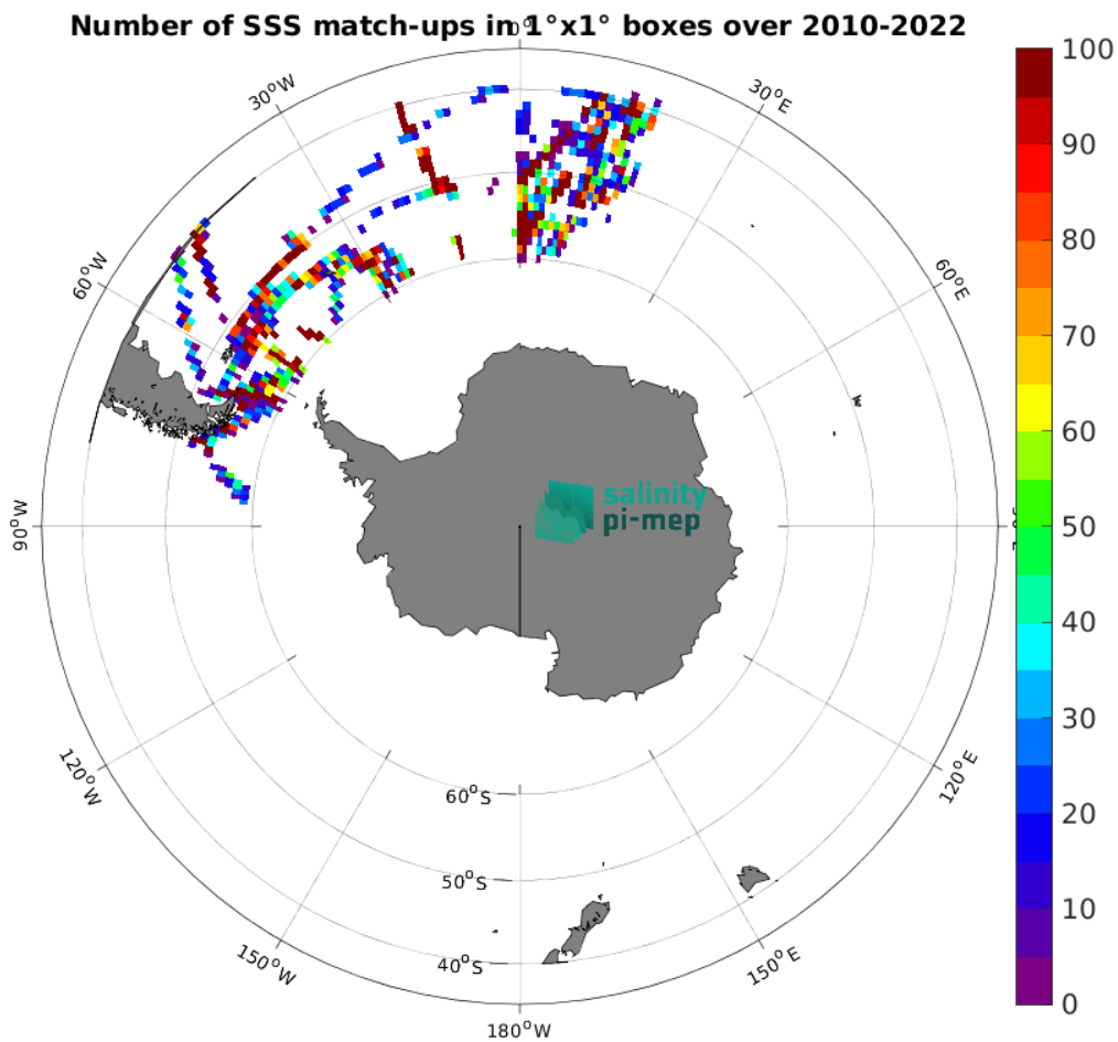
Figure 4: Number of SSS match-ups between TSG (Polarstern) SSS and the SMOS SSS L2 v700 (ESA) SSS product for the Roaring Forties and Furious Fifties Pi-MEP region over 1^\circ \times 1^\circ boxes and for the full satellite product period.
