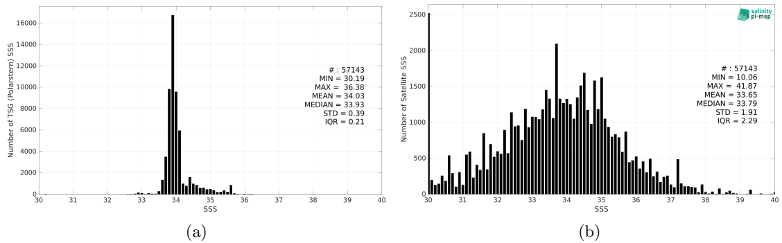
Figure 2: Histograms of SSS from TSG (Polarstern) (a) and SMOS SSS L2 v700 (ESA) (b) considering all match-up pairs per bins of 0.1 over the Roaring Forties and Furious Fifties Pi-MEP region and for the full satellite product period.
