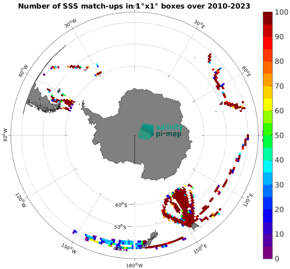
Figure 5: Number of SSS match-ups between TSG (LEGOS-DM) SSS and the SMOS SSS L2 v700 (ESA) SSS product for the Roaring Forties and Furious Fifties Pi-MEP region over 1^\circ \times 1^\circ boxes and for the full satellite product period.
