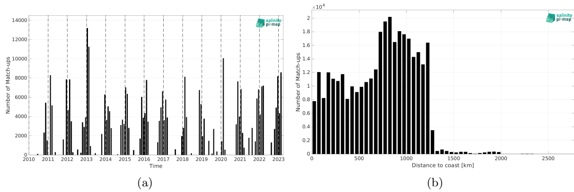
Figure 2: Number of match-ups between TSG (LEGOS-DM) and SMOS SSS L2 v700 (ESA) SSS as a function of time (a) and as function of the distance to coast (b) over the Roaring Forties and Furious Fifties Pi-MEP region and for the full satellite product period.
