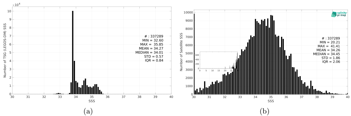
Figure 3: Histograms of SSS from TSG (LEGOS-DM) (a) and SMOS SSS L2 v700 (ESA) (b) considering all match-up pairs per bins of 0.1 over the Roaring Forties and Furious Fifties Pi-MEP region and for the full satellite product period.
