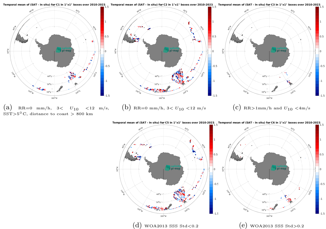
Figure 14: Temporal mean gridded over spatial boxes of size 1^\circ \times 1^\circ of \Delta SSS (SMOS SSS L2 v700 (ESA) - TSG (LEGOS-DM)) for 5 different subdatasets corresponding to: RR=0 mm/h, 3 < U_{10} < 12 m/s, SST > 5°C, distance to coast > 800 km (a), RR=0 mm/h, 3 < U_{10} < 12 m/s (b), RR > 1mm/h and U_{10} < 4 m/s (c), WOA2013 SSS Std < 0.2 (d), WOA2013 SSS Std > 0.2 (e).
