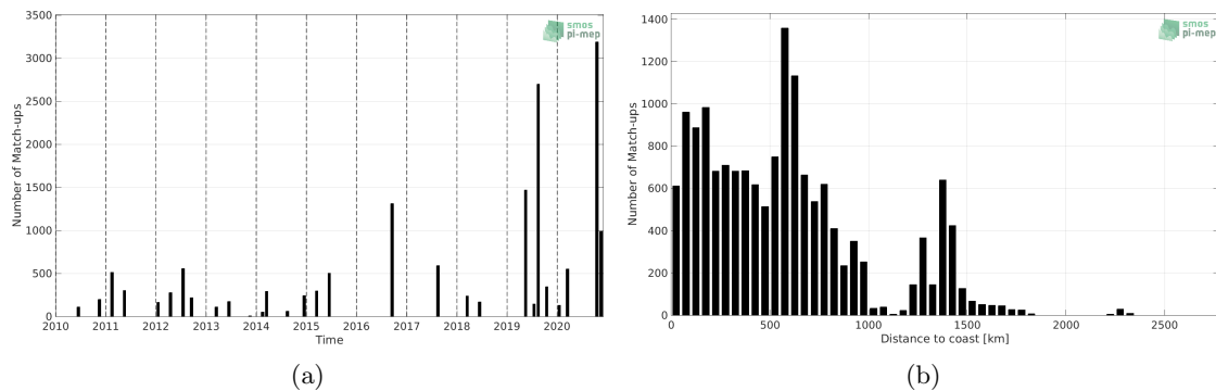
Figure 1: Number of match-ups between TSG (LEGOS-DM) and SMOS SSS L2 v700 (ESA) SSS as a function of time (a) and as function of the distance to coast (b) over the Roaring Forties and Furious Fifties Pi-MEP region and for the full satellite product period.
