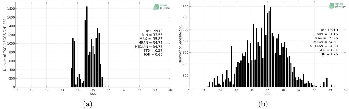
Figure 2: Histograms of SSS from TSG (LEGOS-DM) (a) and SMOS SSS L2 v700 (ESA) (b) considering all match-up pairs per bins of 0.1 over the Roaring Forties and Furious Fifties Pi-MEP region and for the full satellite product period.
