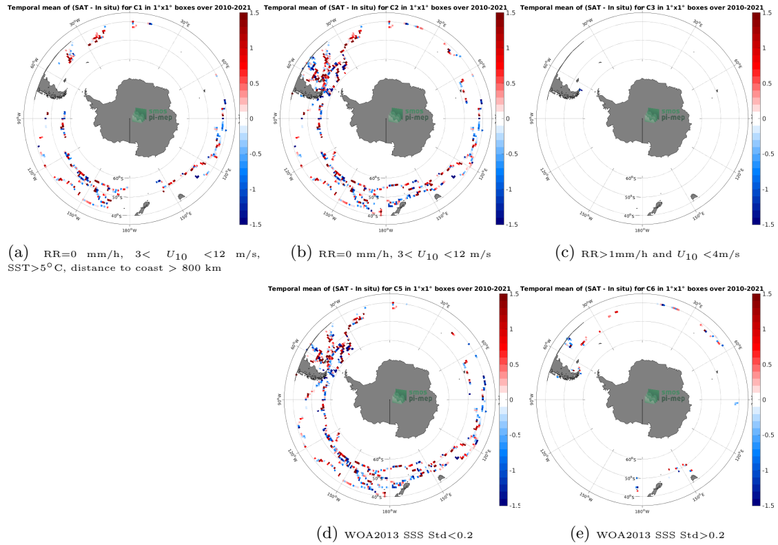
Figure 12: Temporal mean gridded over spatial boxes of size 1^\circ \times 1^\circ of \Delta\text{SSS} (SMOS SSS L2 v700 (ESA) - TSG (GOSUD-Sailing-ship)) for 5 different subdatasets corresponding to: RR=0 mm/h, 3 < U_{10} < 12 m/s, SST > 5^\circ\text{C} , distance to coast > 800 km (a), RR=0 mm/h, 3 < U_{10} < 12 m/s (b), RR > 1 mm/h and U_{10} < 4 m/s (c), WOA2013 SSS Std < 0.2 (d), WOA2013 SSS Std > 0.2 (e).
