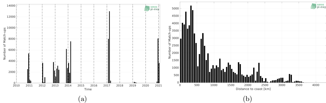
Figure 1: Number of match-ups between TSG (GOSUD-Sailing-ship) and SMOS SSS L2 v700 (ESA) SSS as a function of time (a) and as function of the distance to coast (b) over the Roaring Forties and Furious Fifties Pi-MEP region and for the full satellite product period.
