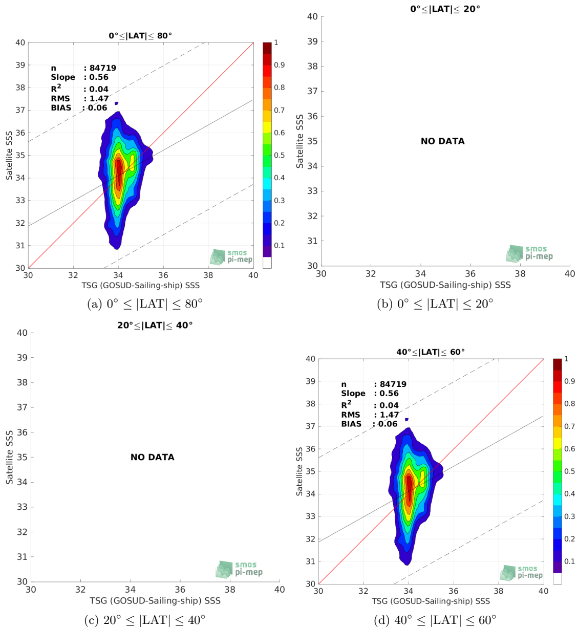
Figure 9: Contour maps of the concentration of SMOS SSS L2 v700 (ESA) SSS (y-axis) versus TSG (GOSUD-Sailing-ship) SSS (x-axis) at match-up pairs for different latitude bands. For each plot, the red line shows x=y . The black thin and dashed lines indicate a linear fit through the data cloud and the \pm 95\% confidence levels, respectively. The number match-up pairs n , the slope and R^2 coefficient of the linear fit, the root mean square (RMS) and the mean bias between satellite and in situ data are indicated for each latitude band in each plot.
