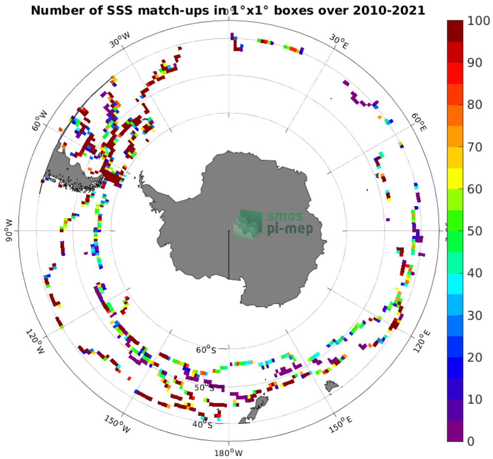
Figure 4: Number of SSS match-ups between TSG (GOSUD-Sailing-ship) SSS and the SMOS SSS L2 v700 (ESA) SSS product for the Roaring Forties and Furious Fifties Pi-MEP region over 1^\circ \times 1^\circ boxes and for the full satellite product period.
