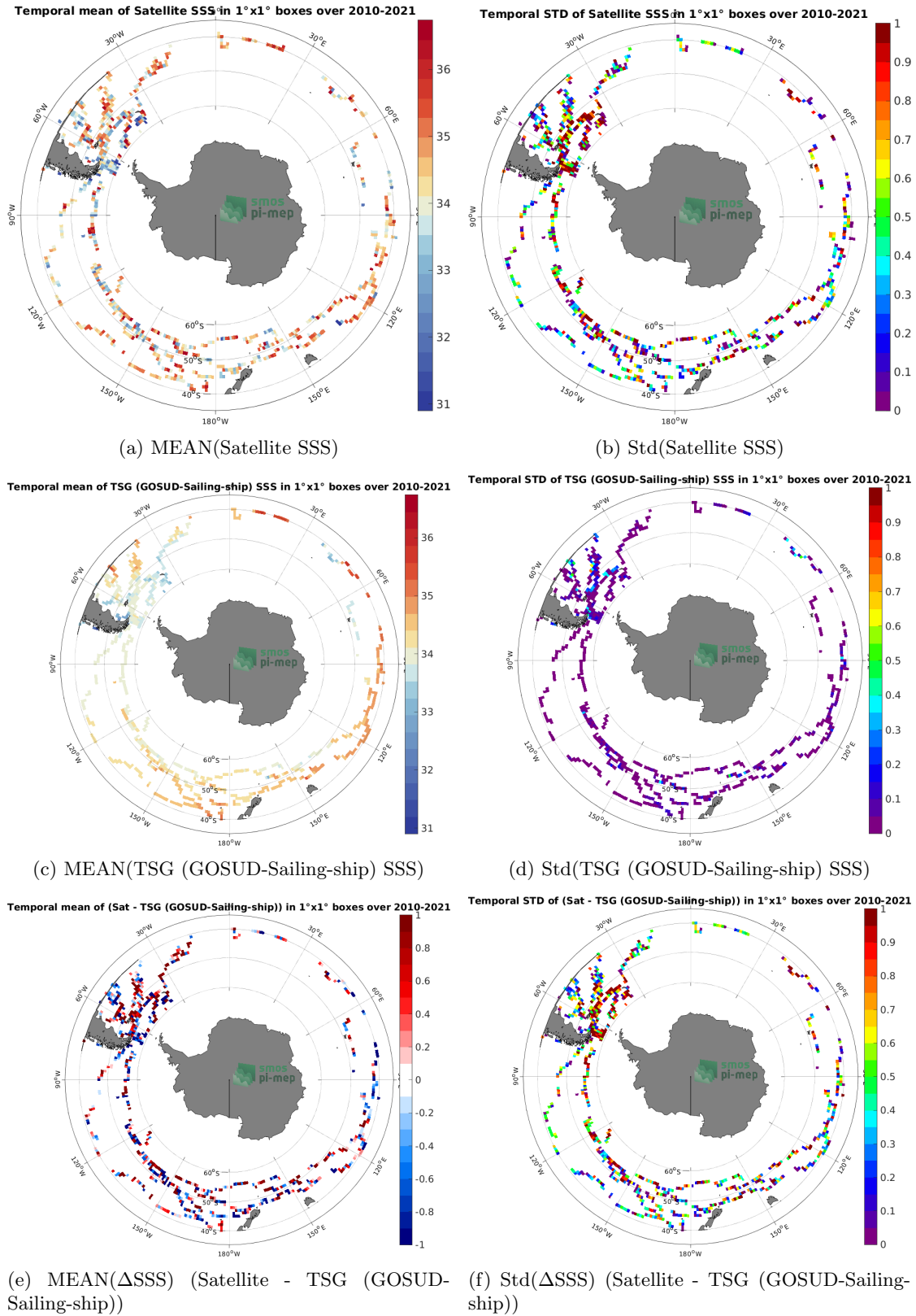
Figure 6: Temporal mean (left) and Std (right) of SSS from SMOS SSS L2 v700 (ESA) (top), TSG (GOSUD-Sailing-ship) (middle), and of \Delta SSS (Satellite - TSG (GOSUD-Sailing-ship)). Only match-up pairs are used to generate these maps.
