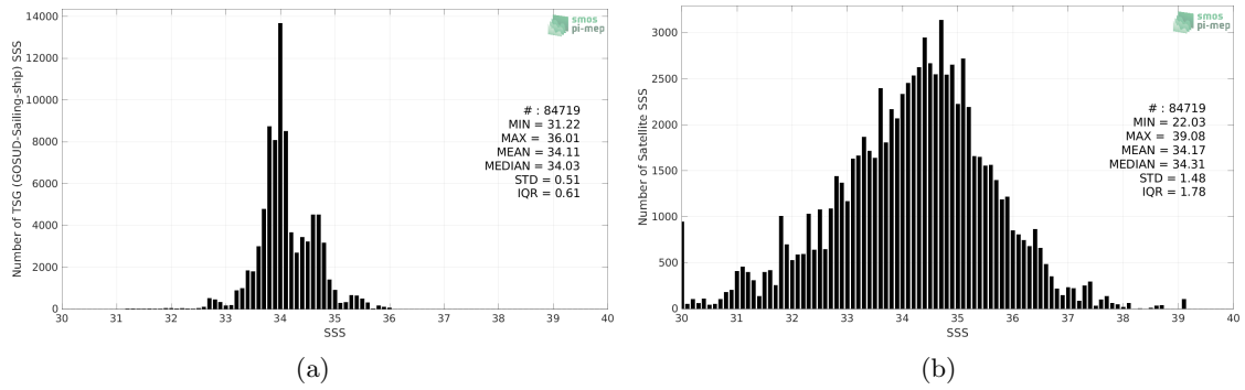
Figure 2: Histograms of SSS from TSG (GOSUD-Sailing-ship) (a) and SMOS SSS L2 v700 (ESA) (b) considering all match-up pairs per bins of 0.1 over the Roaring Forties and Furious Fifties Pi-MEP region and for the full satellite product period.
