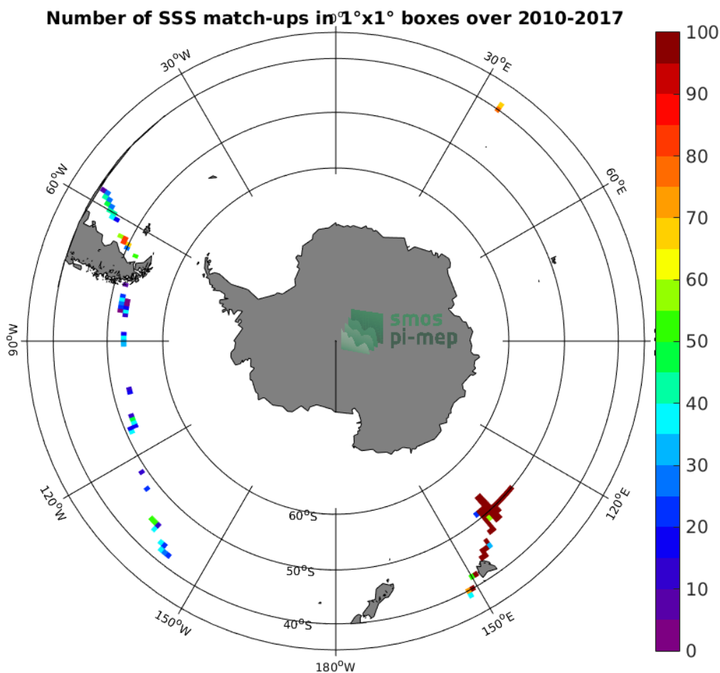
Figure 4: Number of SSS match-ups between TSG (GOSUD-Research-vessel) SSS and the SMOS SSS L2 v700 (ESA) SSS product for the Roaring Forties and Furious Fifties Pi-MEP region over 1^\circ \times 1^\circ boxes and for the full satellite product period.
