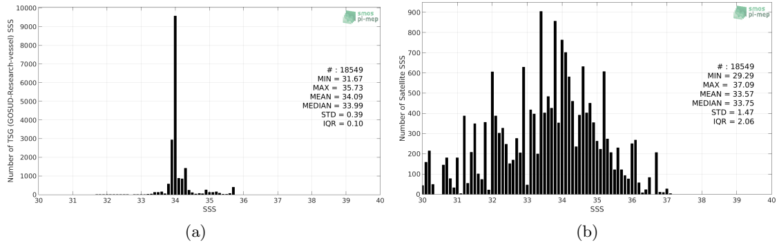
Figure 2: Histograms of SSS from TSG (GOSUD-Research-vessel) (a) and SMOS SSS L2 v700 (ESA) (b) considering all match-up pairs per bins of 0.1 over the Roaring Forties and Furious Fifties Pi-MEP region and for the full satellite product period.
