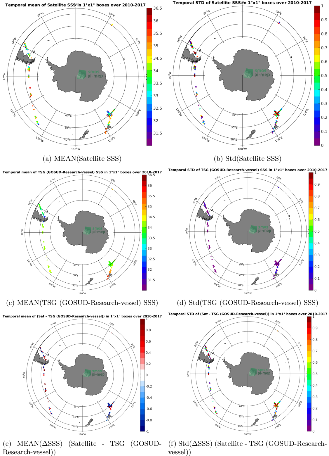
Figure 6: Temporal mean (left) and Std (right) of SSS from SMOS SSS L2 v700 (ESA) (top), TSG (GOSUD-Research-vessel) (middle), and of \Delta SSS (Satellite - TSG (GOSUD-Research-vessel)). Only match-up pairs are used to generate these maps.
