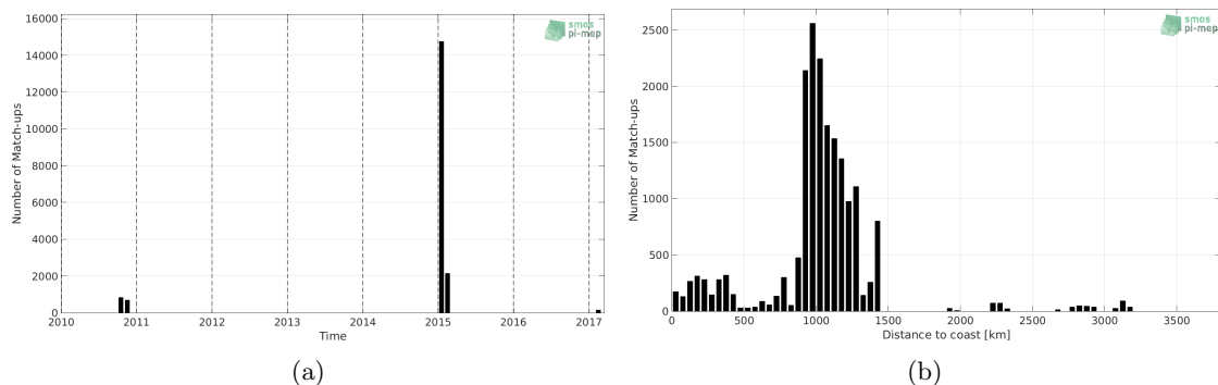
Figure 1: Number of match-ups between TSG (GOSUD-Research-vessel) and SMOS SSS L2 v700 (ESA) SSS as a function of time (a) and as function of the distance to coast (b) over the Roaring Forties and Furious Fifties Pi-MEP region and for the full satellite product period.
