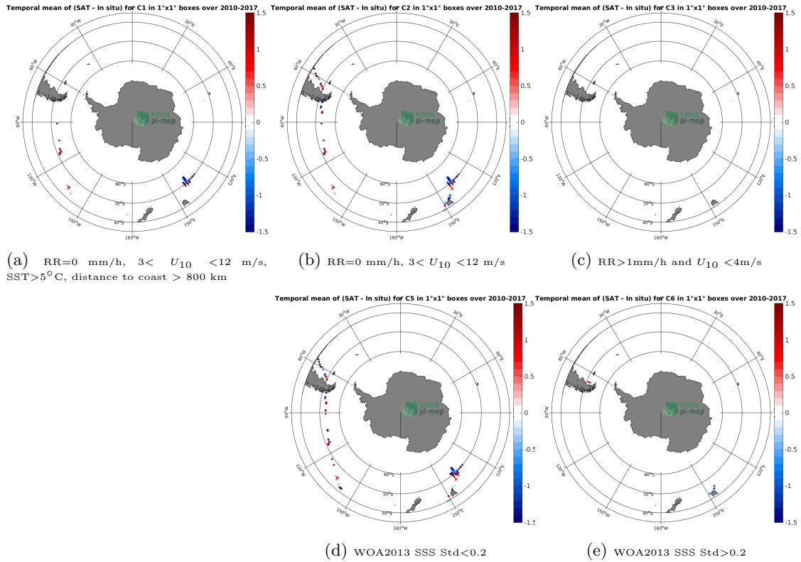
Figure 12: Temporal mean gridded over spatial boxes of size 1°x1° of \Delta SSS (SMOS SSS L2 v700 (ESA) - TSG (GOSUD-Research-vessel)) for 5 different subdatasets corresponding to:RR=0 mm/h, 3 < U_{10} < 12 m/s, SST>5°C, distance to coast > 800 km (a), RR=0 mm/h, 3 < U_{10} < 12 m/s (b), RR>1mm/h and U_{10} < 4 m/s (c), WOA2013 SSS Std<0.2 (d), WOA2013 SSS Std>0.2 (e).
