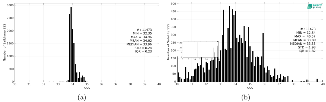
Figure 3: Histograms of SSS from Saildrone (a) and SMOS SSS L2 v700 (ESA) (b) considering all match-up pairs per bins of 0.1 over the Roaring Forties and Furious Fifties Pi-MEP region and for the full satellite product period.
