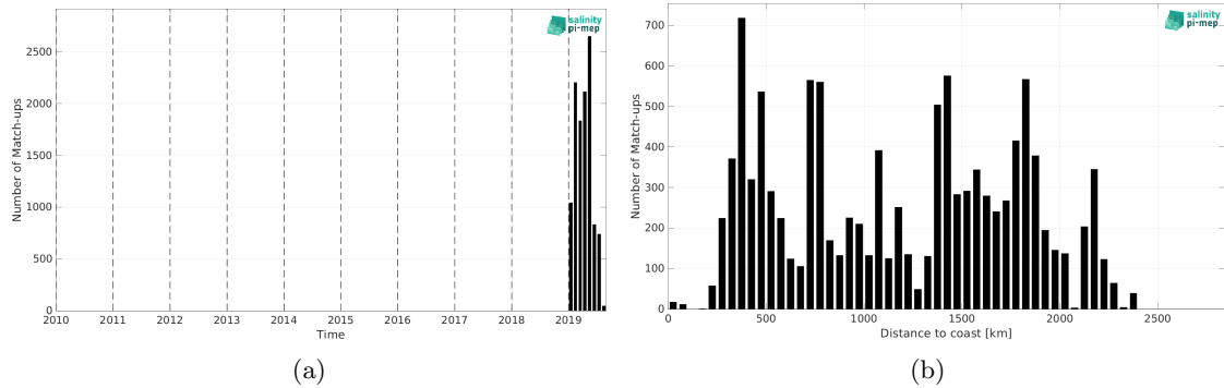
Figure 2: Number of match-ups between Saildrone and SMOS SSS L2 v700 (ESA) SSS as a function of time (a) and as function of the distance to coast (b) over the Roaring Forties and Furious Fifties Pi-MEP region and for the full satellite product period.
