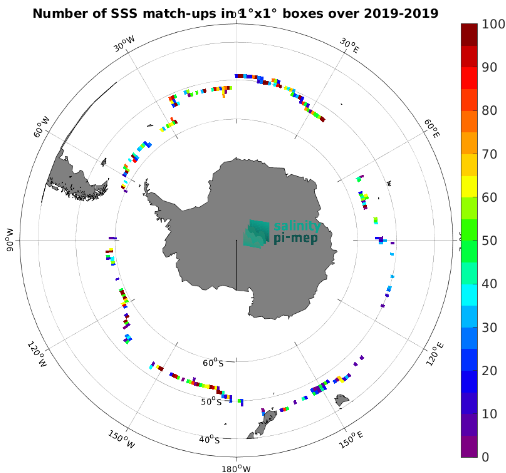
Figure 5: Number of SSS match-ups between Saildrone SSS and the SMOS SSS L2 v700 (ESA) SSS product for the Roaring Forties and Furious Fifties Pi-MEP region over 1^\circ \times 1^\circ boxes and for the full satellite product period.
