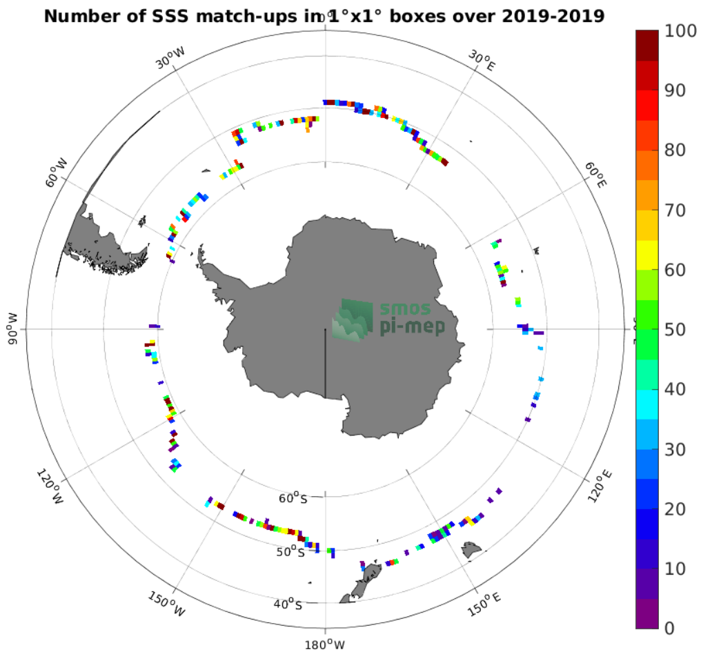
Figure 4: Number of SSS match-ups between Saildrone SSS and the SMOS SSS L2 v700 (ESA) SSS product for the Roaring Forties and Furious Fifties Pi-MEP region over 1^\circ \times 1^\circ boxes and for the full satellite product period.
