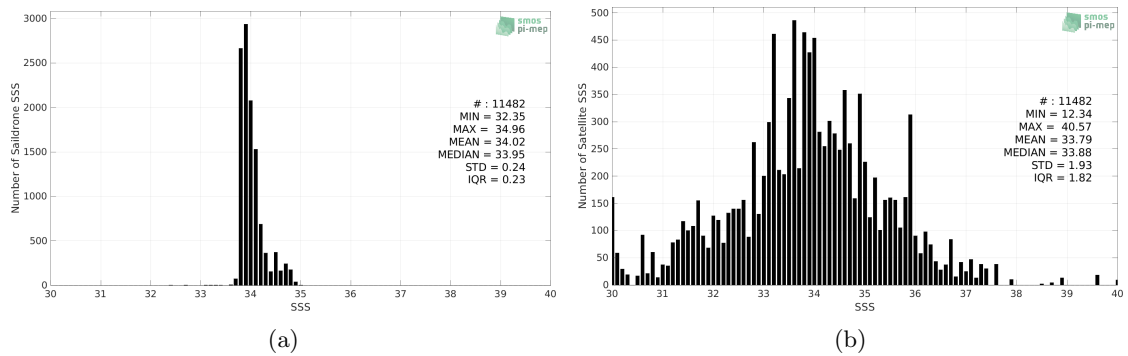
Figure 2: Histograms of SSS from Saildrone (a) and SMOS SSS L2 v700 (ESA) (b) considering all match-up pairs per bins of 0.1 over the Roaring Forties and Furious Fifties Pi-MEP region and for the full satellite product period.
