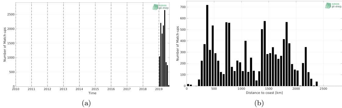
Figure 1: Number of match-ups between Saildrone and SMOS SSS L2 v700 (ESA) SSS as a function of time (a) and as function of the distance to coast (b) over the Roaring Forties and Furious Fifties Pi-MEP region and for the full satellite product period.
