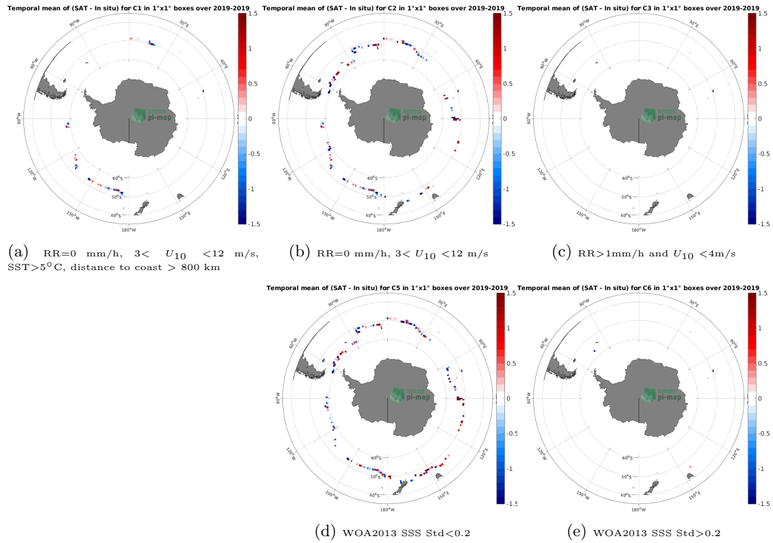
Figure 12: Temporal mean gridded over spatial boxes of size 1^{\circ}\times 1^{\circ} of \Delta\text{SSS} (SMOS SSS L2 v700 (ESA) - Saifrone) for 5 different subdatasets corresponding to: \text{RR}=0 mm/h, 3 < U_{10} < 12 m/s, \text{SST}>5^{\circ}\text{C} , distance to coast > 800 km (a), \text{RR}=0 mm/h, 3 < U_{10} < 12 m/s (b), \text{RR}>1\text{mm/h} and U_{10} < 4\text{m/s} (c), WOA2013 SSS Std < 0.2 (d), WOA2013 SSS Std > 0.2 (e).
