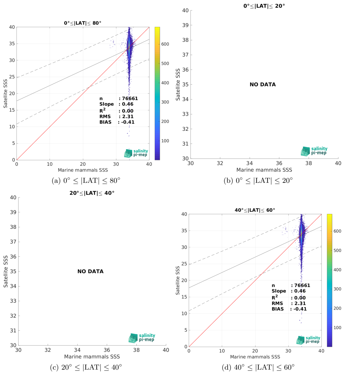
Figure 10: Contour maps of the concentration of SMOS SSS L2 v700 (ESA) SSS (y-axis) versus Marine mammals SSS (x-axis) at match-up pairs for different latitude bands. For each plot, the red line shows x=y . The black thin and dashed lines indicate a linear fit through the data cloud and the \pm 95\% confidence levels, respectively. The number match-up pairs n , the slope and R^2 coefficient of the linear fit, the root mean square (RMS) and the mean bias between satellite and in situ data are indicated for each latitude band in each plots.
