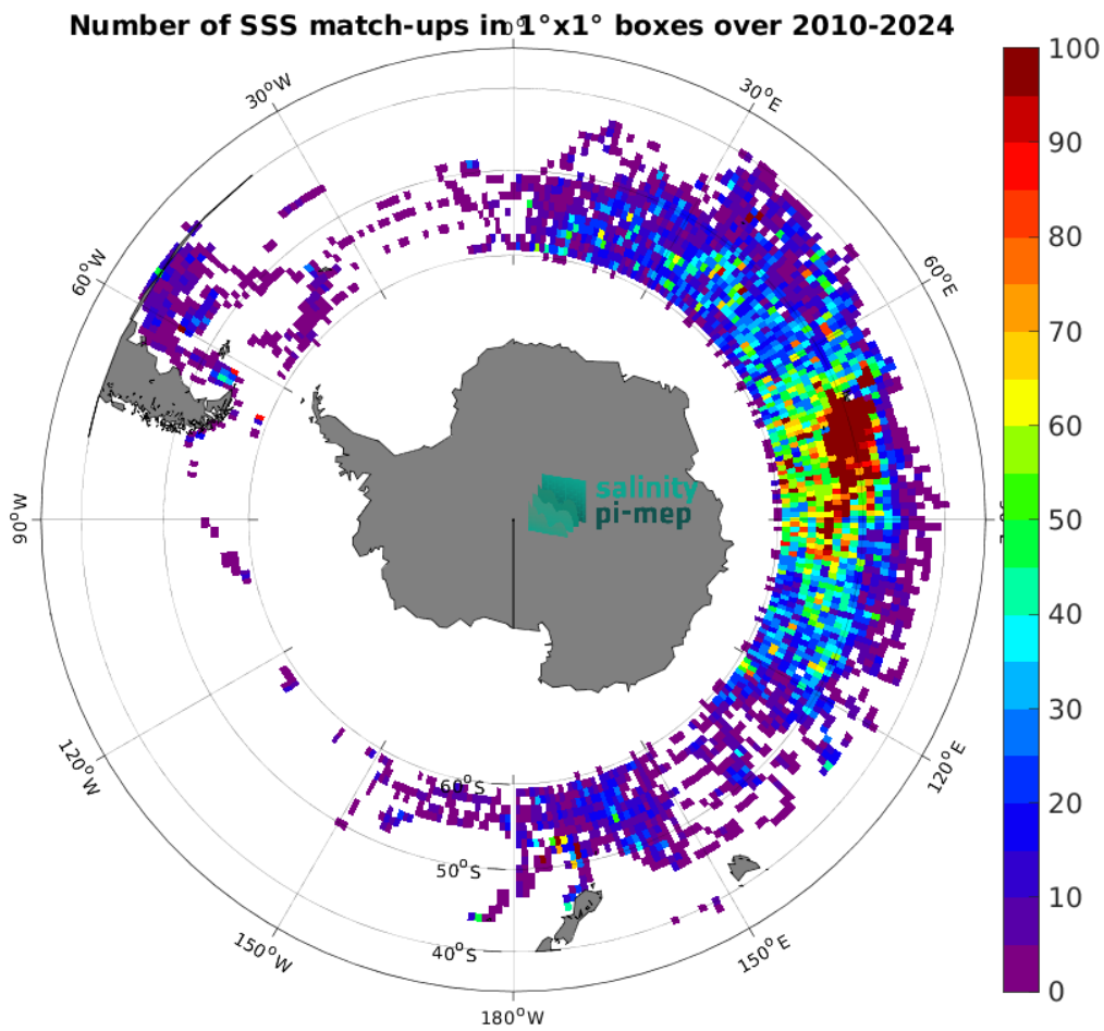
Figure 5: Number of SSS match-ups between Marine mammals SSS and the SMOS SSS L2 v700 (ESA) SSS product for the Roaring Forties and Furious Fifties Pi-MEP region over 1^\circ \times 1^\circ boxes and for the full satellite product period.
