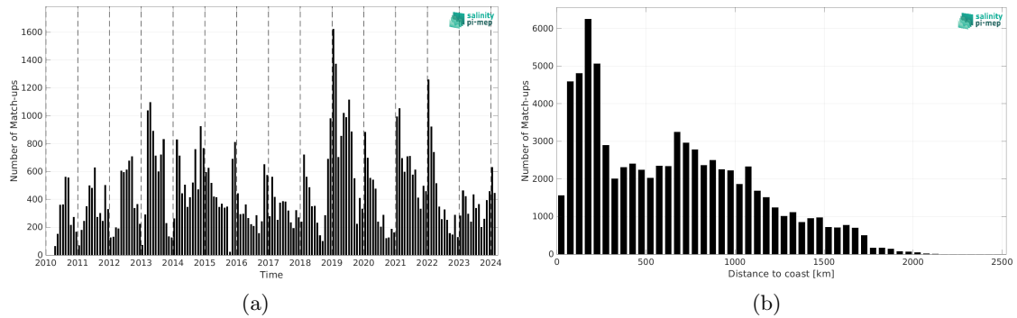
Figure 2: Number of match-ups between Marine mammals and SMOS SSS L2 v700 (ESA) SSS as a function of time (a) and as function of the distance to coast (b) over the Roaring Forties and Furious Fifties Pi-MEP region and for the full satellite product period.
