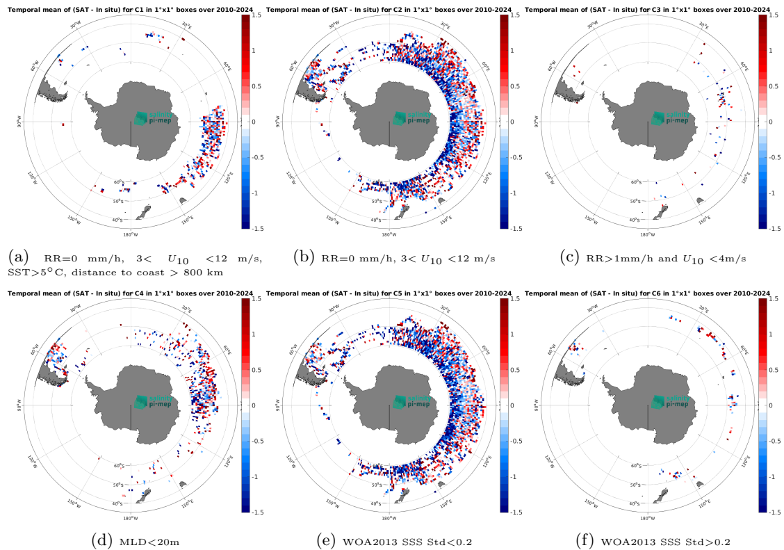
Figure 14: Temporal mean gridded over spatial boxes of size 1^\circ \times 1^\circ of \Delta SSS (SMOS SSS L2 v700 (ESA) - Marine mammals) for 6 different subdatasets corresponding to:RR=0 mm/h, 3 < U_{10} < 12 m/s, SST>5°C, distance to coast > 800 km (a), RR=0 mm/h, 3 < U_{10} < 12 m/s (b), RR>1mm/h and U_{10} < 4 m/s (c),MLD<20m (d),WOA2013 SSS Std<0.2 (e),WOA2013 SSS Std>0.2 (f).
