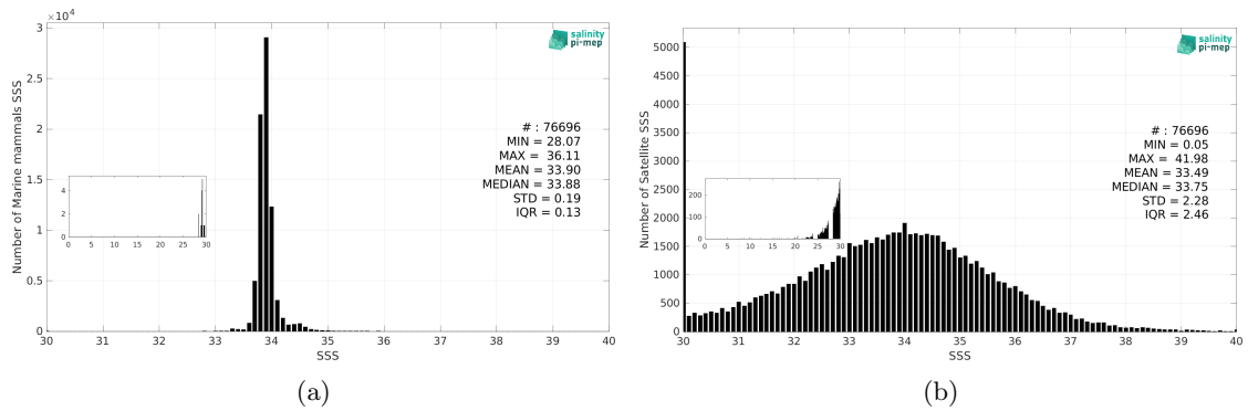
Figure 3: Histograms of SSS from Marine mammals (a) and SMOS SSS L2 v700 (ESA) (b) considering all match-up pairs per bins of 0.1 over the Roaring Forties and Furious Fifties Pi-MEP region and for the full satellite product period.
