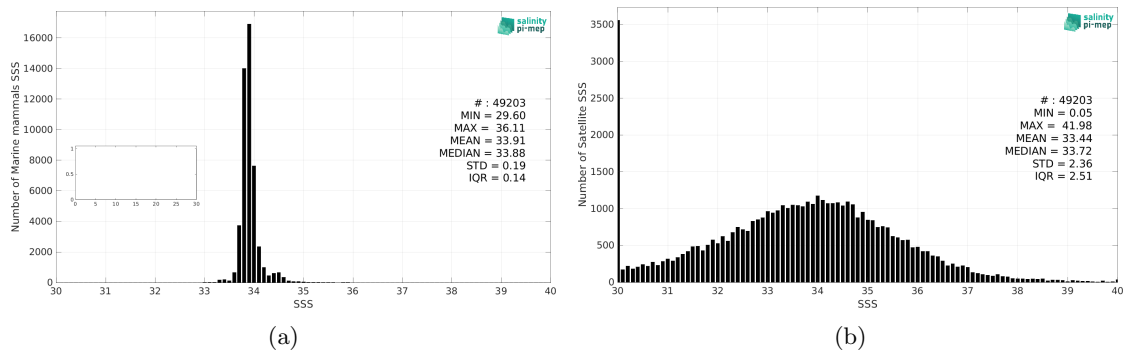
Figure 2: Histograms of SSS from Marine mammals (a) and SMOS SSS L2 v700 (ESA) (b) considering all match-up pairs per bins of 0.1 over the Roaring Forties and Furious Fifties Pi-MEP region and for the full satellite product period.
