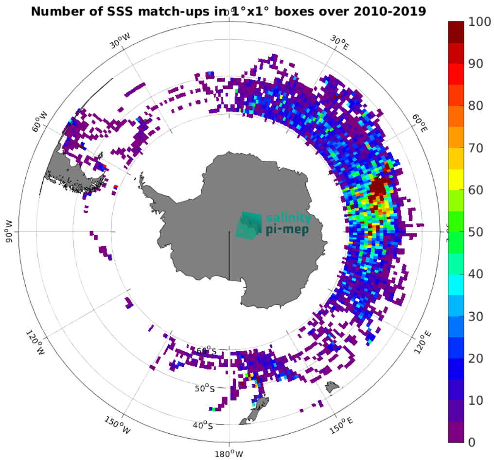
Figure 4: Number of SSS match-ups between Marine mammals SSS and the SMOS SSS L2 v700 (ESA) SSS product for the Roaring Forties and Furious Fifties Pi-MEP region over 1^\circ \times 1^\circ boxes and for the full satellite product period.
