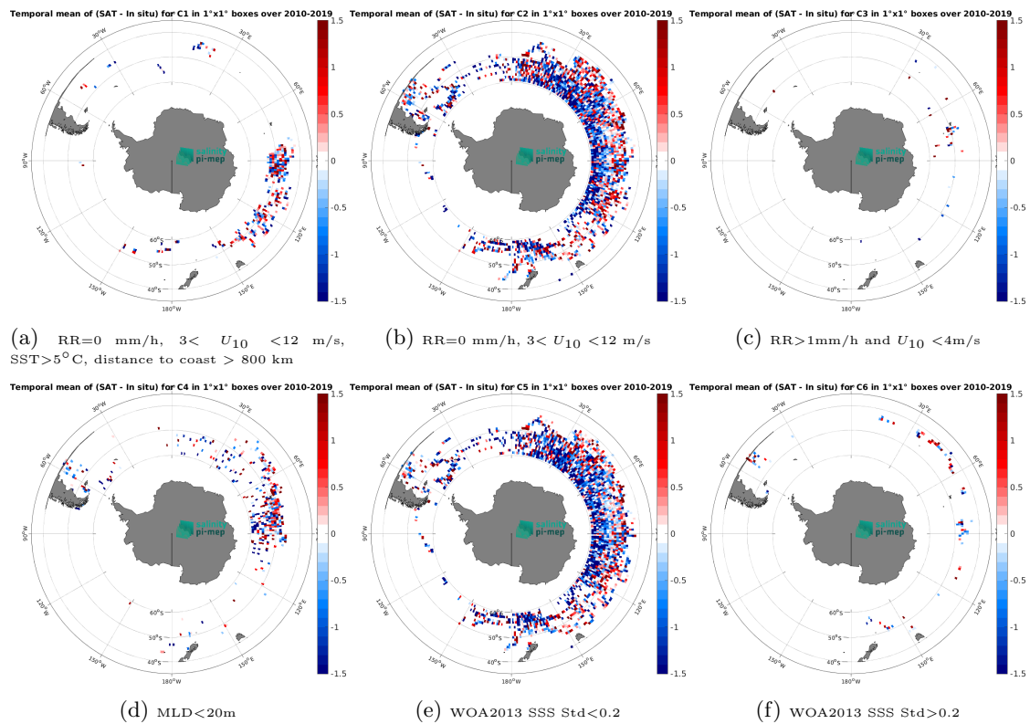
Figure 12: Temporal mean gridded over spatial boxes of size 1^{\circ}\times 1^{\circ} of \Delta\text{SSS} (SMOS SSS L2 v700 (ESA) - Marine mammals) for 6 different subdatasets corresponding to:RR=0 mm/h, 3 < U_{10} < 12 m/s, SST >5^{\circ}\text{C} , distance to coast > 800 km (a), RR=0 mm/h, 3 < U_{10} < 12 m/s (b), RR >1 mm/h and U_{10} < 4 m/s (c),MLD <20 m (d),WOA2013 SSS Std <0.2 (e),WOA2013 SSS Std >0.2 (f).
