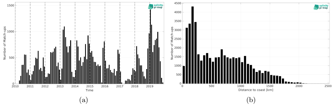
Figure 1: Number of match-ups between Marine mammals and SMOS SSS L2 v700 (ESA) SSS as a function of time (a) and as function of the distance to coast (b) over the Roaring Forties and Furious Fifties Pi-MEP region and for the full satellite product period.
