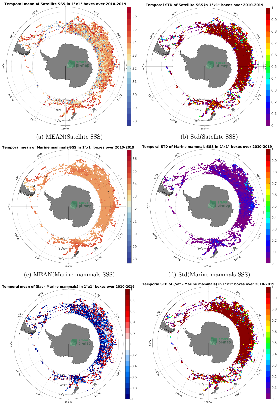
(e) MEAN( \Delta SSS) (Satellite - Marine mammals) 20 (f) Std( \Delta SSS) (Satellite - Marine mammals)
