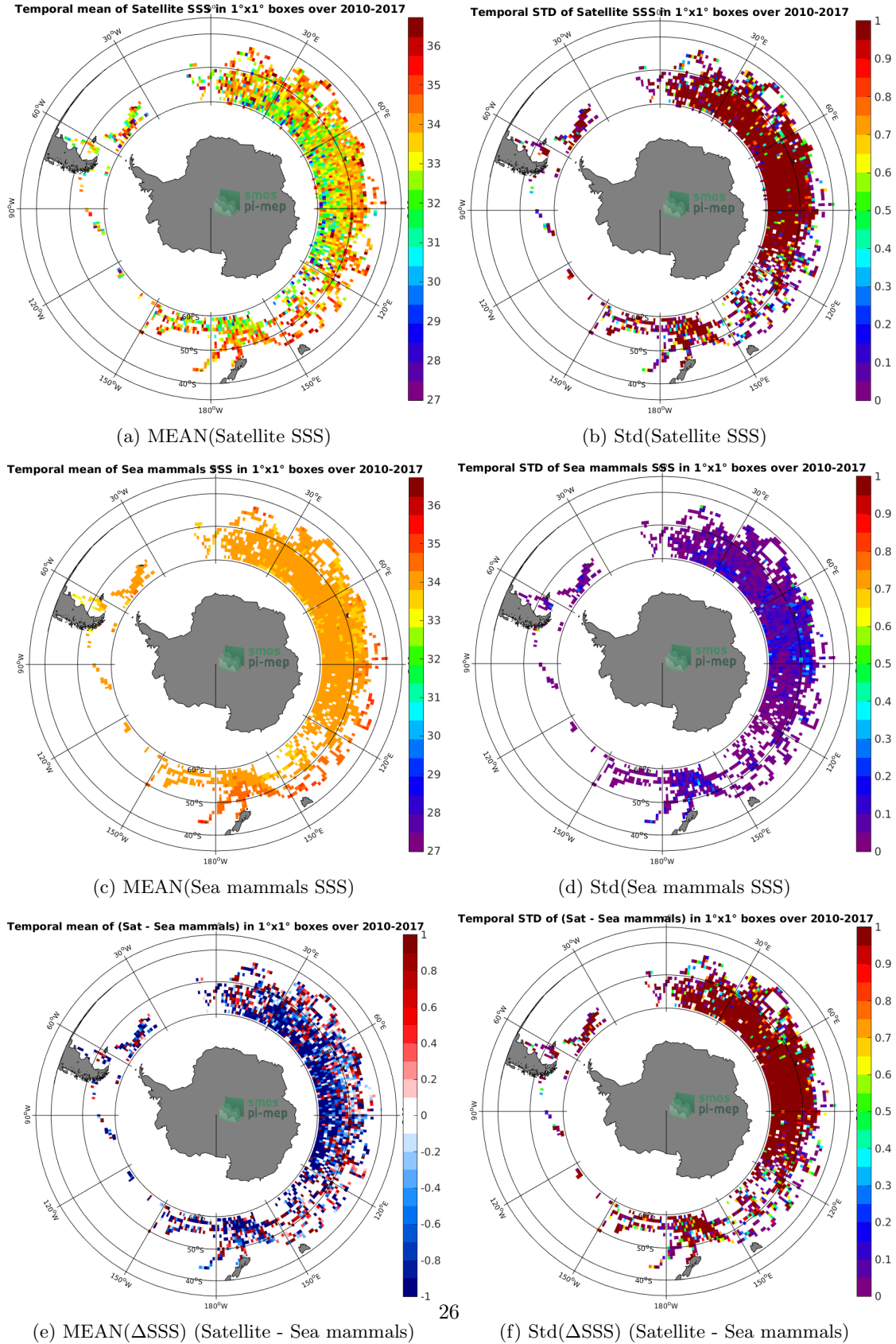
Figure 6: Temporal mean (left) and Std (right) of SSS from SMOS SSS L2 v700 (ESA) (top), Sea mammals (middle), and of \Delta SSS (Satellite - Sea mammals). Only match-up pairs are used to generate these maps.
