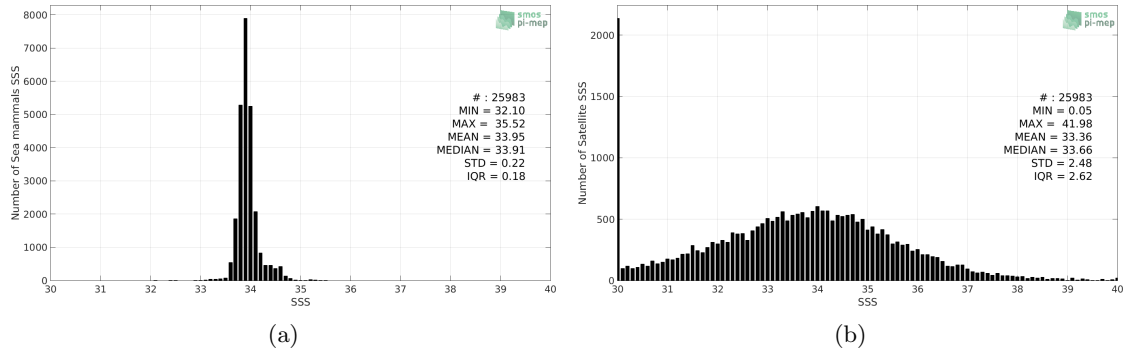
Figure 2: Histograms of SSS from Sea mammals (a) and SMOS SSS L2 v700 (ESA) (b) considering all match-up pairs per bins of 0.1 over the Roaring Forties and Furious Fifties Pi-MEP region and for the full satellite product period.
