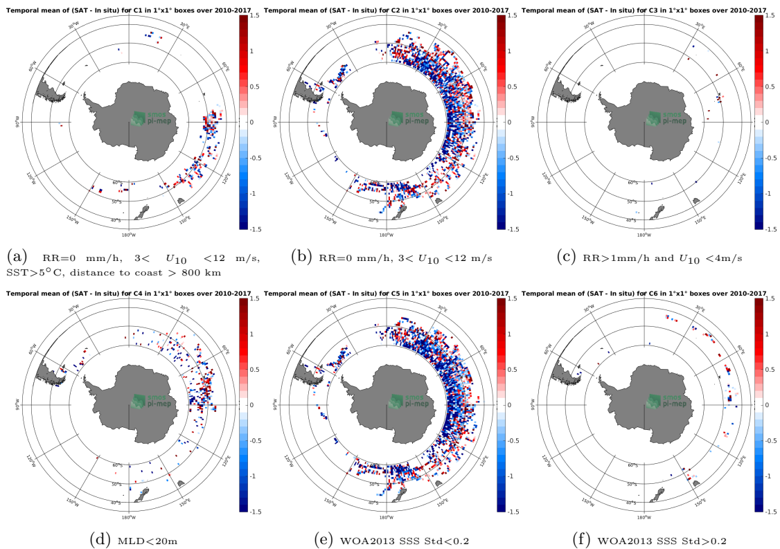
Figure 12: Temporal mean gridded over spatial boxes of size 1^{\circ}\times 1^{\circ} of \Delta\text{SSS} (SMOS SSS L2 v700 (ESA) - Sea mammals) for 6 different subdatasets corresponding to:RR=0 mm/h, 3 < U_{10} < 12 m/s, SST >5^{\circ}\text{C} , distance to coast > 800 km (a), RR=0 mm/h, 3 < U_{10} < 12 m/s (b), RR >1\text{mm/h} and U_{10} < 4\text{m/s} (c),MLD <20\text{m} (d),WOA2013 SSS Std <0.2 (e),WOA2013 SSS Std >0.2 (f).
