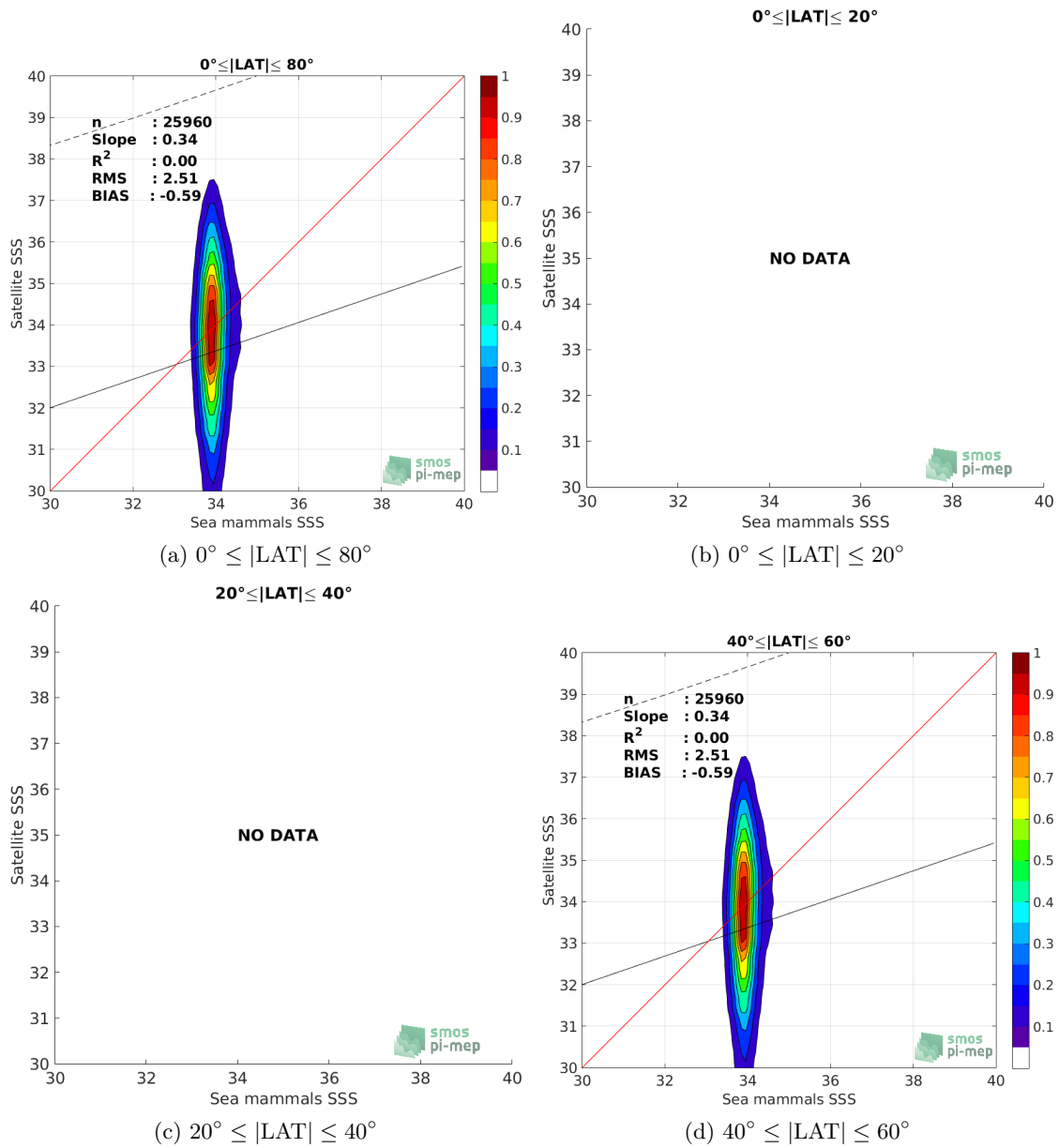
Figure 9: Contour maps of the concentration of SMOS SSS L2 v700 (ESA) SSS (y-axis) versus Sea mammals SSS (x-axis) at match-up pairs for different latitude bands. For each plot, the red line shows x=y . The black thin and dashed lines indicate a linear fit through the data cloud and the \pm 95\% confidence levels, respectively. The number match-up pairs n , the slope and R^2 coefficient of the linear fit, the root mean square (RMS) and the mean bias between satellite and in situ data are indicated for each latitude band in each plots.
