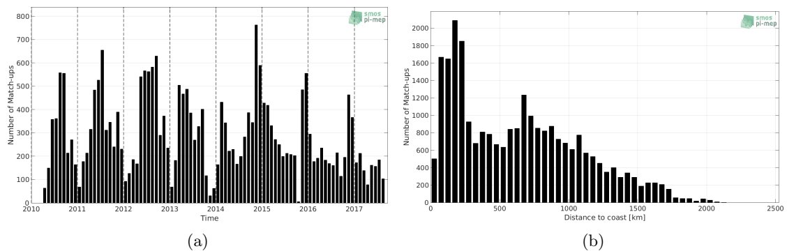
Figure 1: Number of match-ups between Sea mammals and SMOS SSS L2 v700 (ESA) SSS as a function of time (a) and as function of the distance to coast (b) over the Roaring Forties and Furious Fifties Pi-MEP region and for the full satellite product period.
