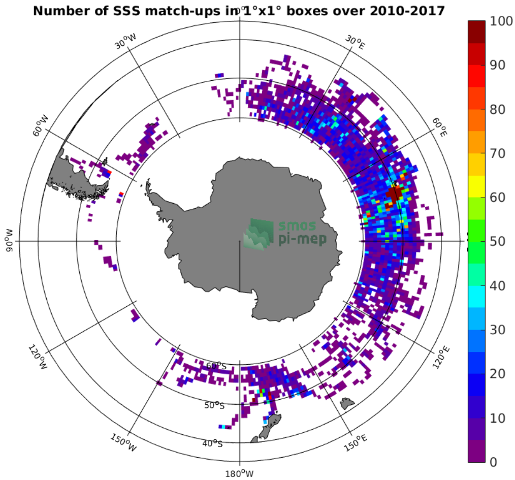
Figure 4: Number of SSS match-ups between Sea mammals SSS and the SMOS SSS L2 v700 (ESA) SSS product for the Roaring Forties and Furious Fifties Pi-MEP region over 1^\circ \times 1^\circ boxes and for the full satellite product period.
