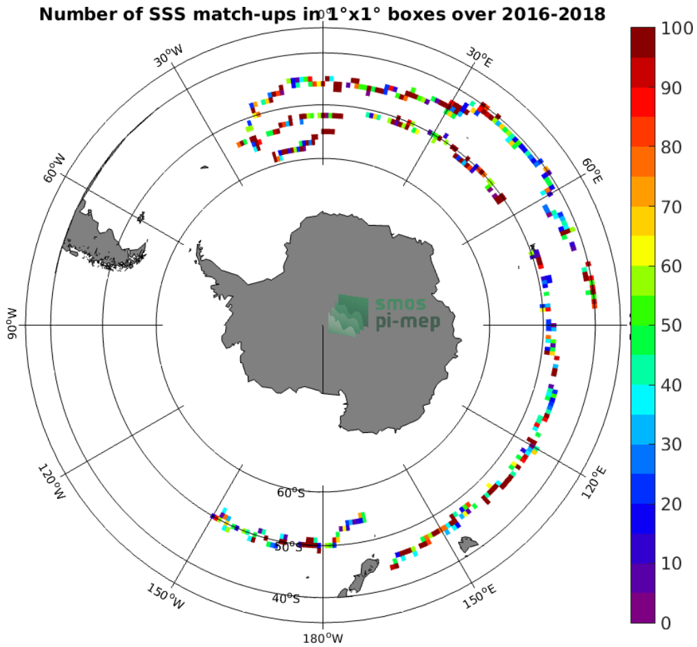
Figure 3: Number of SSS match-ups between Surface drifters SSS and the SMOS SSS L2 v700 (ESA) SSS product for the Roaring Forties and Furious Fifties Pi-MEP region over 1^\circ \times 1^\circ boxes and for the full satellite product period.
