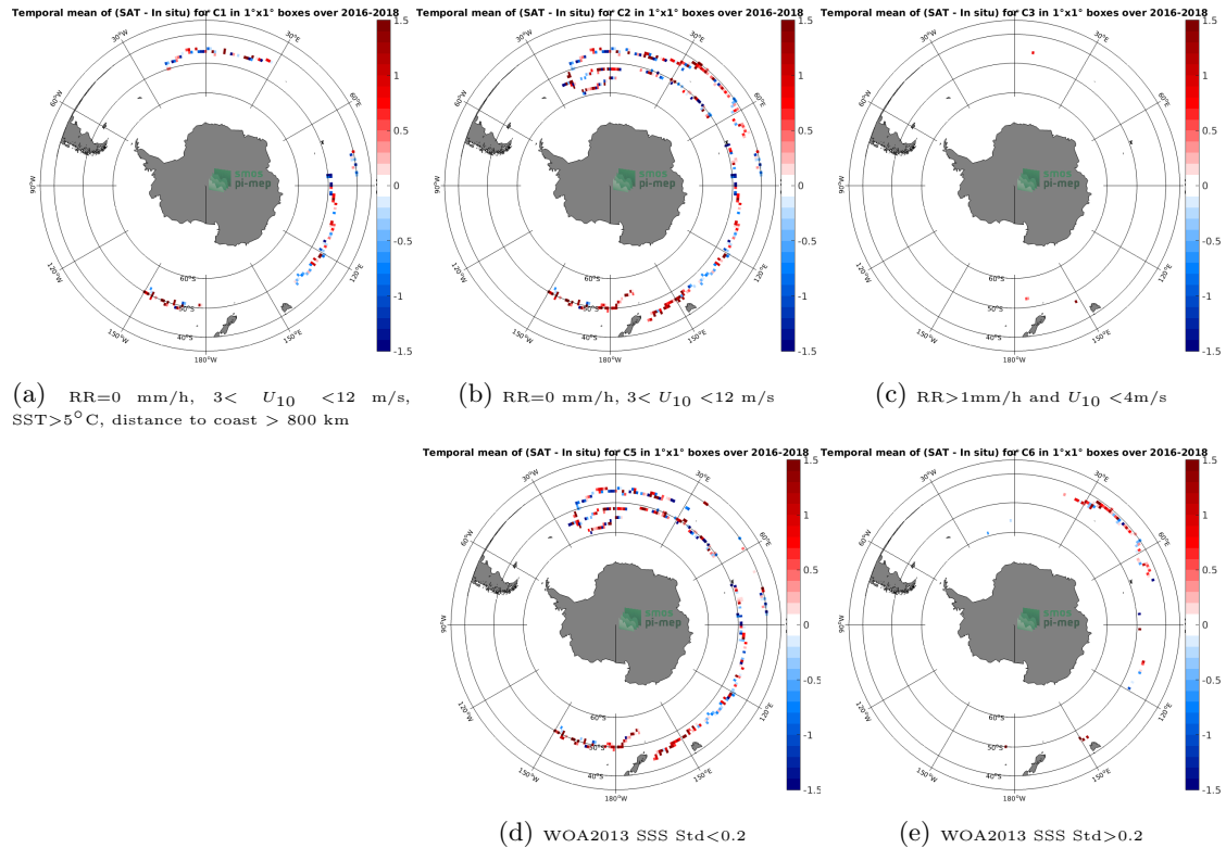
Figure 11: Temporal mean gridded over spatial boxes of size 1^{\circ}\times 1^{\circ} of \Delta\text{SSS} (SMOS SSS L2 v700 (ESA) - Surface drifters) for 5 different subdatasets corresponding to:RR=0 mm/h, 3 < U_{10} < 12 m/s, SST >5^{\circ}\text{C} , distance to coast > 800 km (a), RR=0 mm/h, 3 < U_{10} < 12 m/s (b), RR >1 mm/h and U_{10} < 4 m/s (c), WOA2013 SSS Std <0.2 (d), WOA2013 SSS Std >0.2 (e).
