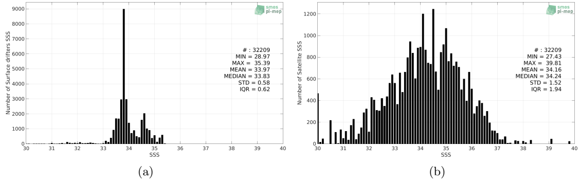
Figure 2: Histograms of SSS from Surface drifters (a) and SMOS SSS L2 v700 (ESA) (b) considering all match-up pairs per bins of 0.1 over the Roaring Forties and Furious Fifties Pi-MEP region and for the full satellite product period.
