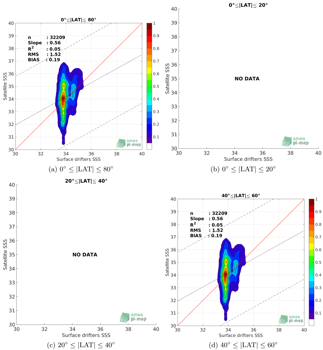
Figure 8: Contour maps of the concentration of SMOS SSS L2 v700 (ESA) SSS (y-axis) versus Surface drifters SSS (x-axis) at match-up pairs for different latitude bands. For each plot, the red line shows x=y . The black thin and dashed lines indicate a linear fit through the data cloud and the \pm 95\% confidence levels, respectively. The number match-up pairs n , the slope and R^2 coefficient of the linear fit, the root mean square (RMS) and the mean bias between satellite and in situ data are indicated for each latitude band in each plots.
