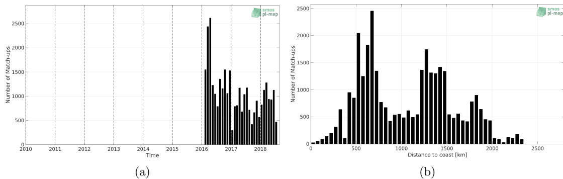
Figure 1: Number of match-ups between Surface drifters and SMOS SSS L2 v700 (ESA) SSS as a function of time (a) and as function of the distance to coast (b) over the Roaring Forties and Furious Fifties Pi-MEP region and for the full satellite product period.
