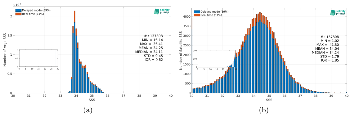
Figure 3: Histograms of SSS from Argo (a) and SMOS SSS L2 v700 (ESA) (b) considering all match-up pairs per bins of 0.1 over the Roaring Forties and Furious Fifties Pi-MEP region and for the full satellite product period.
