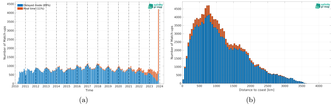
Figure 2: Number of match-ups between Argo and SMOS SSS L2 v700 (ESA) SSS as a function of time (a) and as function of the distance to coast (b) over the Roaring Forties and Furious Fifties Pi-MEP region and for the full satellite product period.
