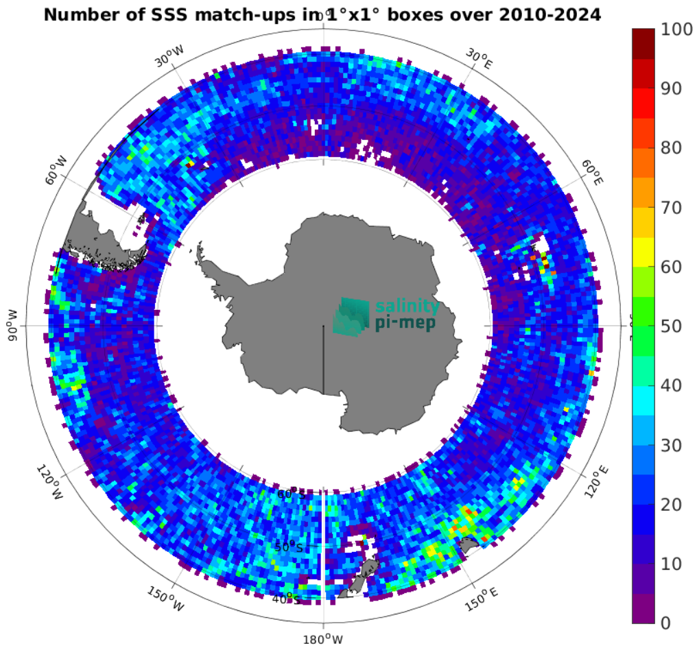
Figure 5: Number of SSS match-ups between Argo SSS and the SMOS SSS L2 v700 (ESA) SSS product for the Roaring Forties and Furious Fifties Pi-MEP region over 1^\circ \times 1^\circ boxes and for the full satellite product period.
