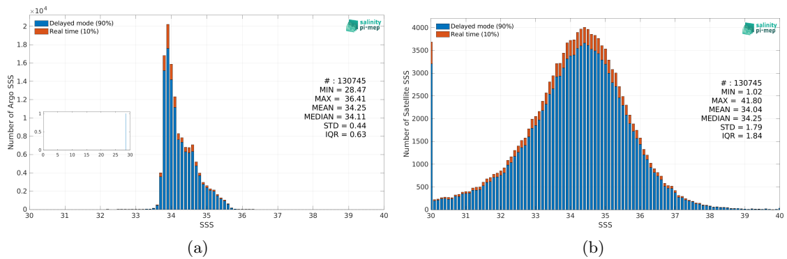
Figure 2: Histograms of SSS from Argo (a) and SMOS SSS L2 v700 (ESA) (b) considering all match-up pairs per bins of 0.1 over the Roaring Forties and Furious Fifties Pi-MEP region and for the full satellite product period.
