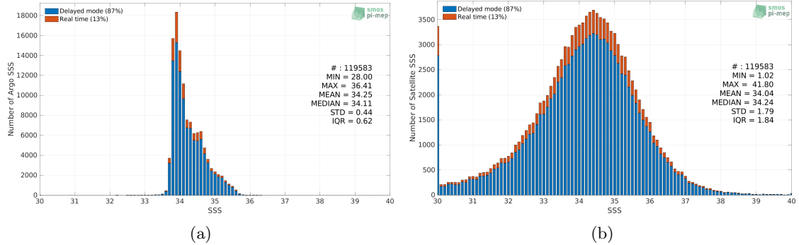
Figure 2: Histograms of SSS from Argo (a) and SMOS SSS L2 v700 (ESA) (b) considering all match-up pairs per bins of 0.1 over the Roaring Forties and Furious Fifties Pi-MEP region and for the full satellite product period.
