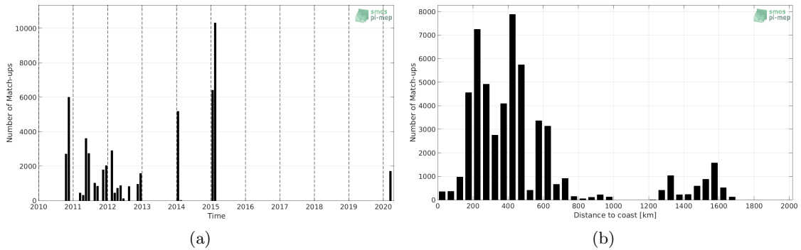
Figure 1: Number of match-ups between TSG (SAMOS) and SMOS SSS L2 v662 (ESA) SSS as a function of time (a) and as function of the distance to coast (b) over the Roaring Forties and Furious Fifties Pi-MEP region and for the full satellite product period.
