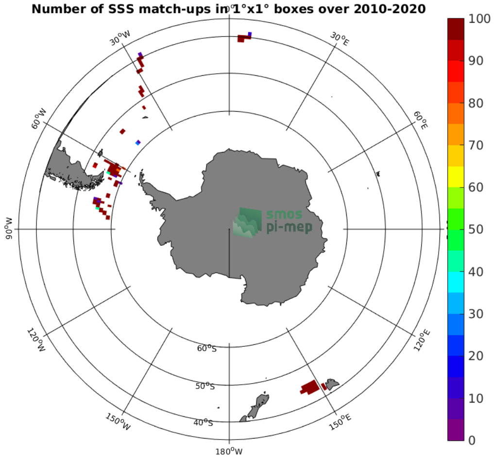
Figure 4: Number of SSS match-ups between TSG (SAMOS) SSS and the SMOS SSS L2 v662 (ESA) SSS product for the Roaring Forties and Furious Fifties Pi-MEP region over 1°x1° boxes and for the full satellite product period.
