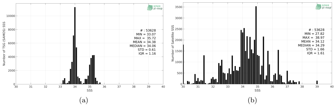
Figure 2: Histograms of SSS from TSG (SAMOS) (a) and SMOS SSS L2 v662 (ESA) (b) considering all match-up pairs per bins of 0.1 over the Roaring Forties and Furious Fifties Pi-MEP region and for the full satellite product period.
