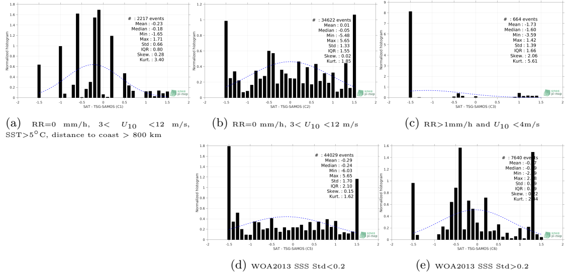
Figure 13: Normalized histogram of \Delta SSS (SMOS L2 v662 (ESA) - TSG-SAMOS) for 5 different subdatasets corresponding to: RR=0 mm/h, 3 < U_{10} < 12 m/s, SST > 5°C, distance to coast > 800 km (a), RR=0 mm/h, 3 < U_{10} < 12 m/s (b), RR > 1mm/h and U_{10} < 4 m/s (c), WOA2013 SSS Std < 0.2 (d), WOA2013 SSS Std > 0.2 (e).
