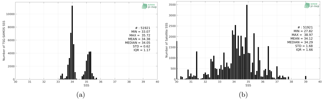
Figure 2: Histograms of SSS from TSG-SAMOS (a) and SMOS L2 v662 (ESA) (b) considering all match-up pairs per bins of 0.1 over the Roaring Forties and Furious Fifties Pi-MEP region and for the full satellite product period.
