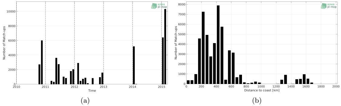
Figure 1: Number of match-ups between TSG-SAMOS and SMOS L2 v662 (ESA) SSS as a function of time (a) and as function of the distance to coast (b) over the Roaring Forties and Furious Fifties Pi-MEP region and for the full satellite product period.
