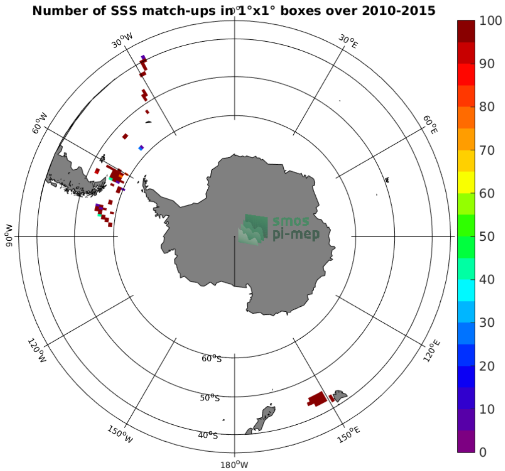
Figure 4: Number of SSS match-ups between TSG-SAMOS SSS and the SMOS L2 v662 (ESA) SSS product for the Roaring Forties and Furious Fifties Pi-MEP region over 1°x1° boxes and for the full satellite product period.
