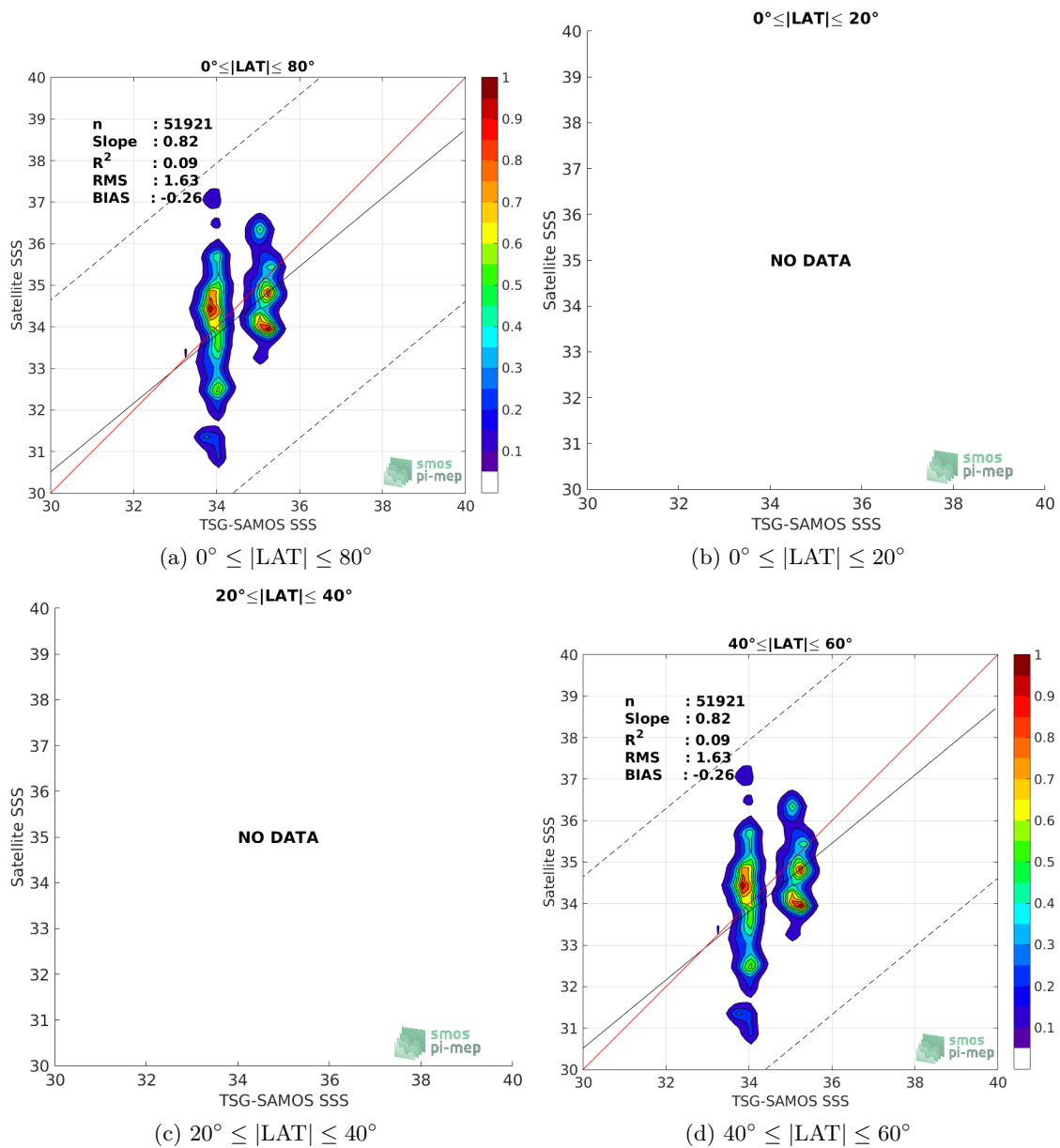
Figure 9: Contour maps of the concentration of SMOS L2 v662 (ESA) SSS (y-axis) versus TSG-SAMOS SSS (x-axis) at match-up pairs for different latitude bands. For each plot, the red line shows x=y . The black thin and dashed lines indicate a linear fit through the data cloud and the \pm 95\% confidence levels, respectively. The number match-up pairs n , the slope and R^2 coefficient of the linear fit, the root mean square (RMS) and the mean bias between satellite and in situ data are indicated for each latitude band in each plots.
