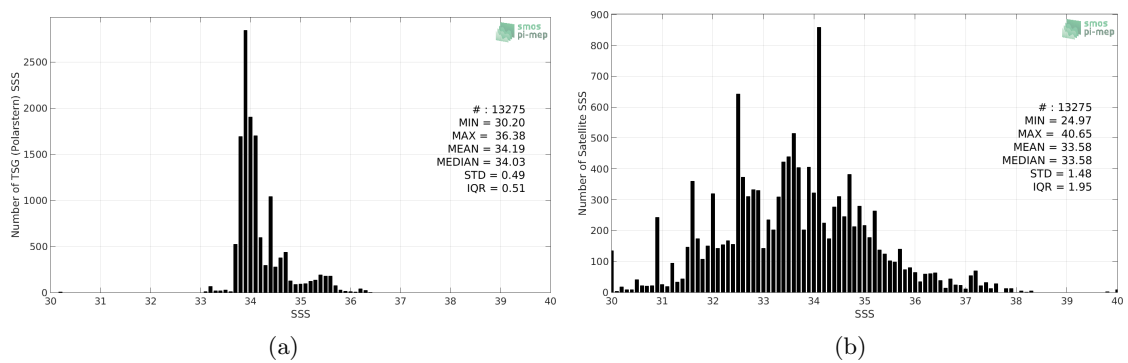
Figure 2: Histograms of SSS from TSG (Polarstern) (a) and SMOS SSS L2 v662 (ESA) (b) considering all match-up pairs per bins of 0.1 over the Roaring Forties and Furious Fifties Pi-MEP region and for the full satellite product period.
