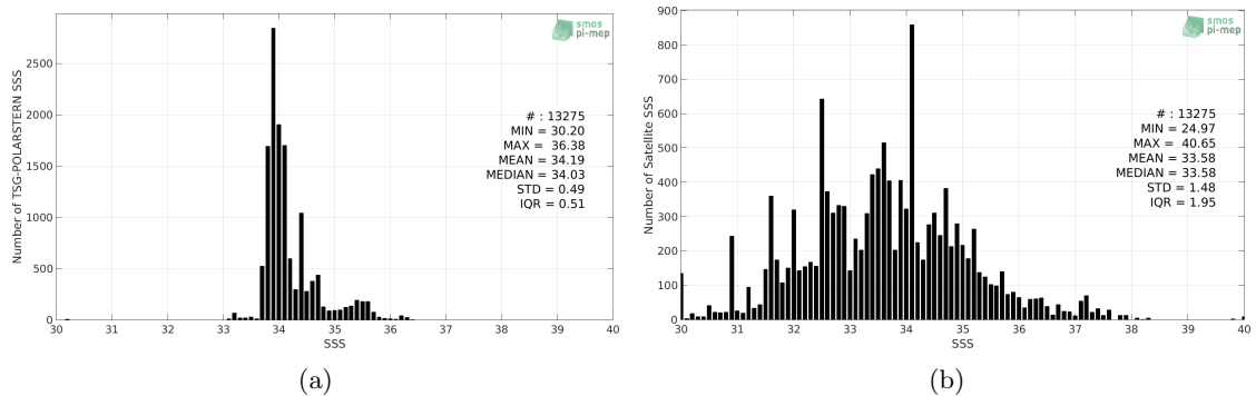
Figure 2: Histograms of SSS from TSG-POLARSTERN (a) and SMOS L2 v662 (ESA) (b) considering all match-up pairs per bins of 0.1 over the Roaring Forties and Furious Fifties Pi-MEP region and for the full satellite product period.
