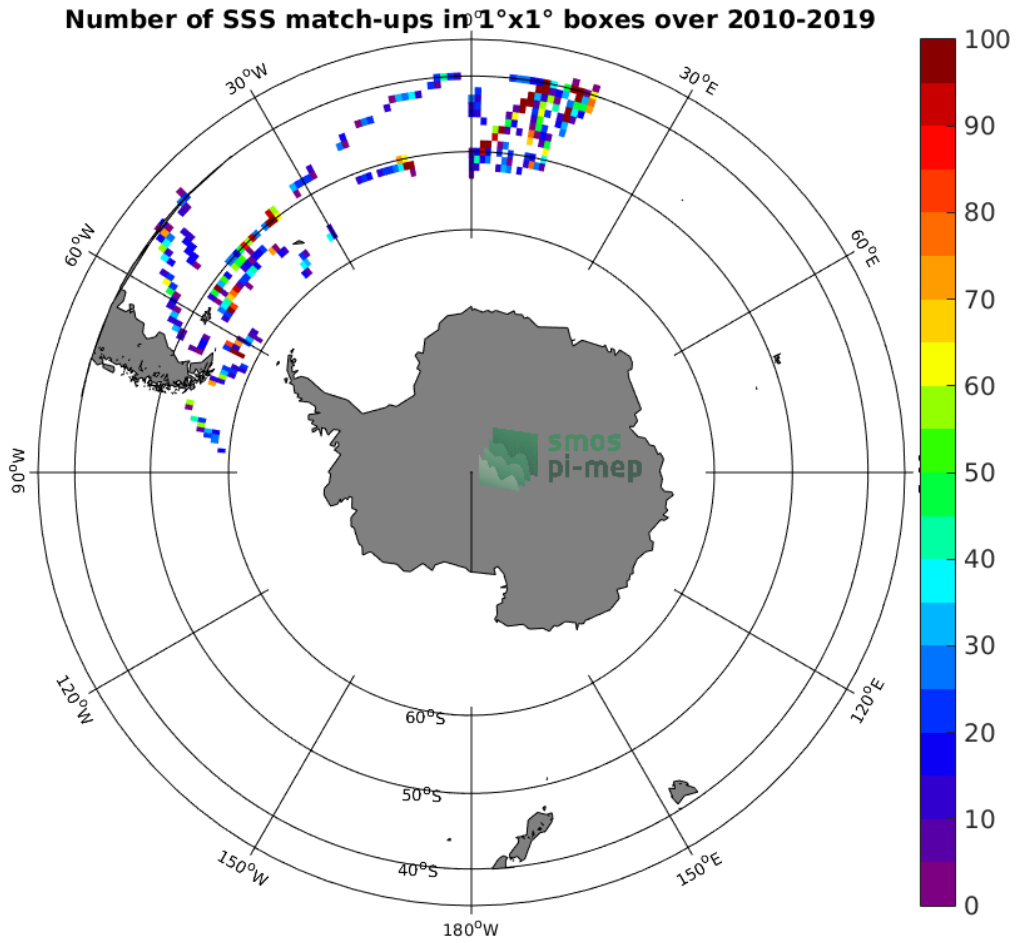
Figure 4: Number of SSS match-ups between TSG-POLARSTERN SSS and the SMOS L2 v662 (ESA) SSS product for the Roaring Forties and Furious Fifties Pi-MEP region over 1°x1° boxes and for the full satellite product period.
