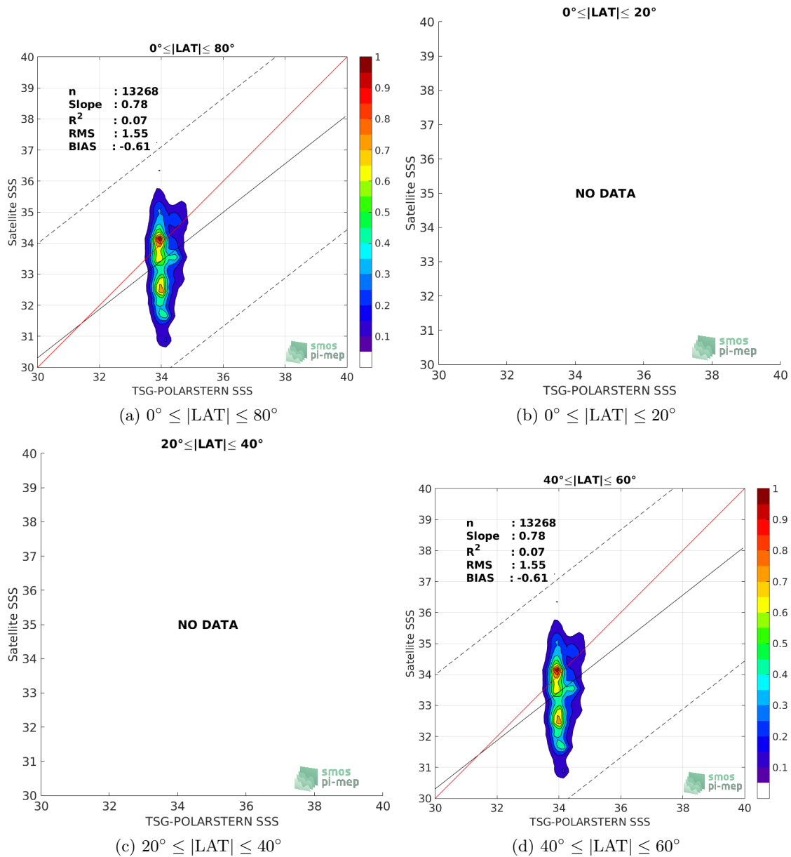
Figure 9: Contour maps of the concentration of SMOS L2 v662 (ESA) SSS (y-axis) versus TSG-POLARSTERN SSS (x-axis) at match-up pairs for different latitude bands. For each plot, the red line shows x=y . The black thin and dashed lines indicate a linear fit through the data cloud and the \pm 95\% confidence levels, respectively. The number match-up pairs n , the slope and R^2 coefficient of the linear fit, the root mean square (RMS) and the mean bias between satellite and in situ data are indicated for each latitude band in each plots.
