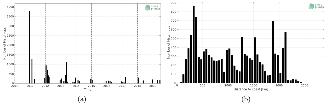
Figure 1: Number of match-ups between TSG-POLARSTERN and SMOS L2 v662 (ESA) SSS as a function of time (a) and as function of the distance to coast (b) over the Roaring Forties and Furious Fifties Pi-MEP region and for the full satellite product period.
