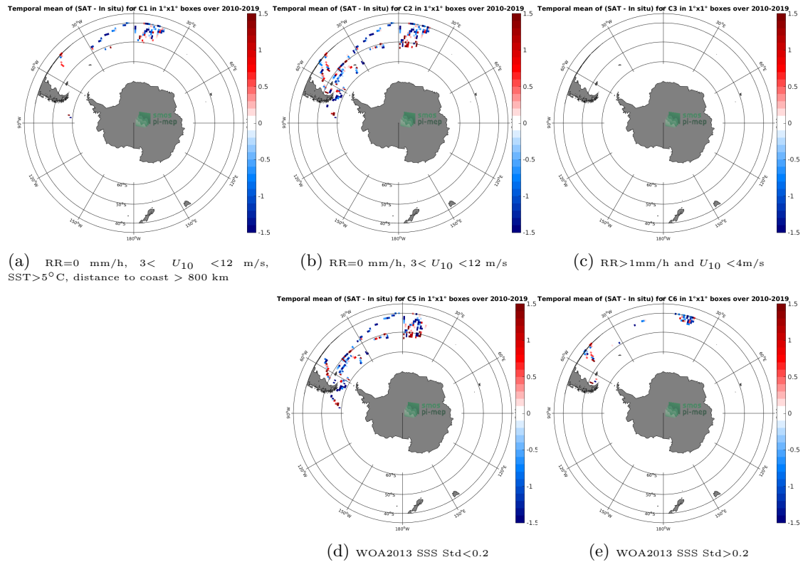
Figure 12: Temporal mean gridded over spatial boxes of size 1^{\circ}\times 1^{\circ} of \Delta\text{SSS} (SMOS L2 v662 (ESA) - TSG-POLARSTERN) for 5 different subdatasets corresponding to:RR=0 mm/h, 3 < U_{10} < 12 m/s, SST >5^{\circ}\text{C} , distance to coast > 800 km (a), RR=0 mm/h, 3 < U_{10} < 12 m/s (b), RR >1 mm/h and U_{10} < 4 m/s (c), WOA2013 SSS Std <0.2 (d), WOA2013 SSS Std >0.2 (e).
