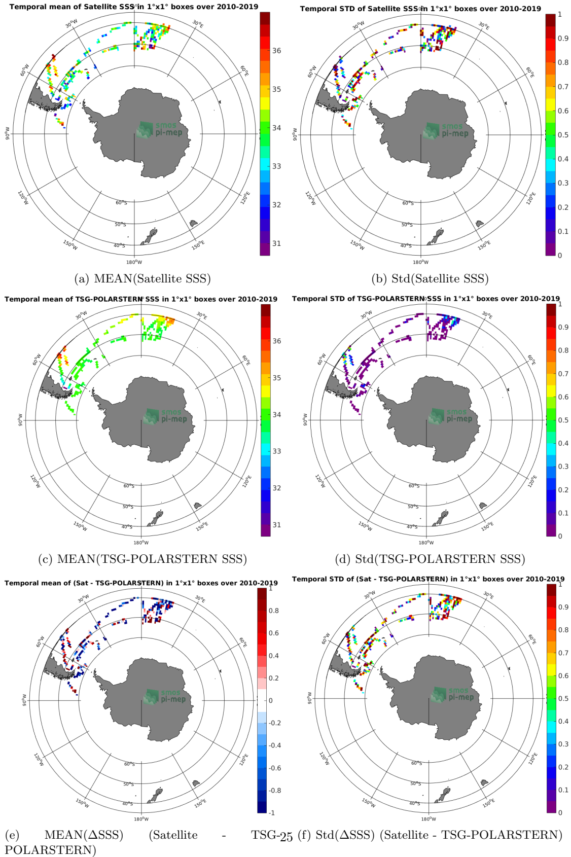
Figure 6: Temporal mean (left) and Std (right) of SSS from SMOS L2 v662 (ESA) (top), TSG-POLARSTERN (middle), and of \Delta SSS (Satellite - TSG-POLARSTERN). Only match-up pairs are used to generate these maps.
