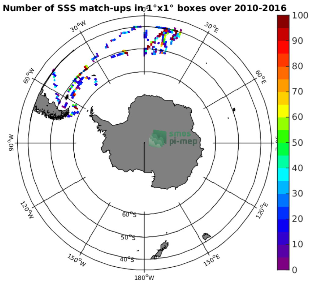
Figure 4: Number of SSS match-ups between TSG-POLARSTERN SSS and the SMOS-L2-DPGS-v662 SSS product for the Roaring Forties and Furious Fifties Pi-MEP region over 1°x1° boxes and for the full satellite product period.
