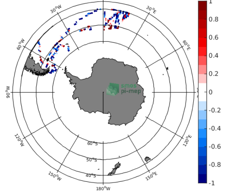
(e) MEAN( \Delta SSS) (Satellite - TSG-POLARSTERN)
