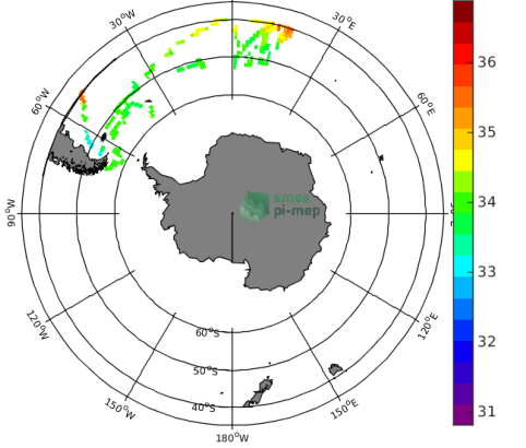
(c) MEAN(TSG-POLARSTERN SSS)
