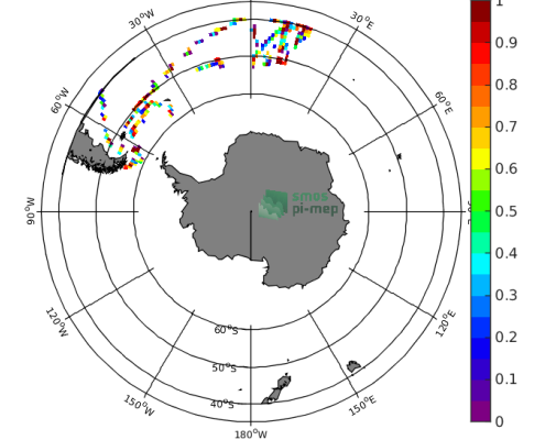
(f) Std( \Delta SSS) (Satellite - TSG-POLARSTERN)
