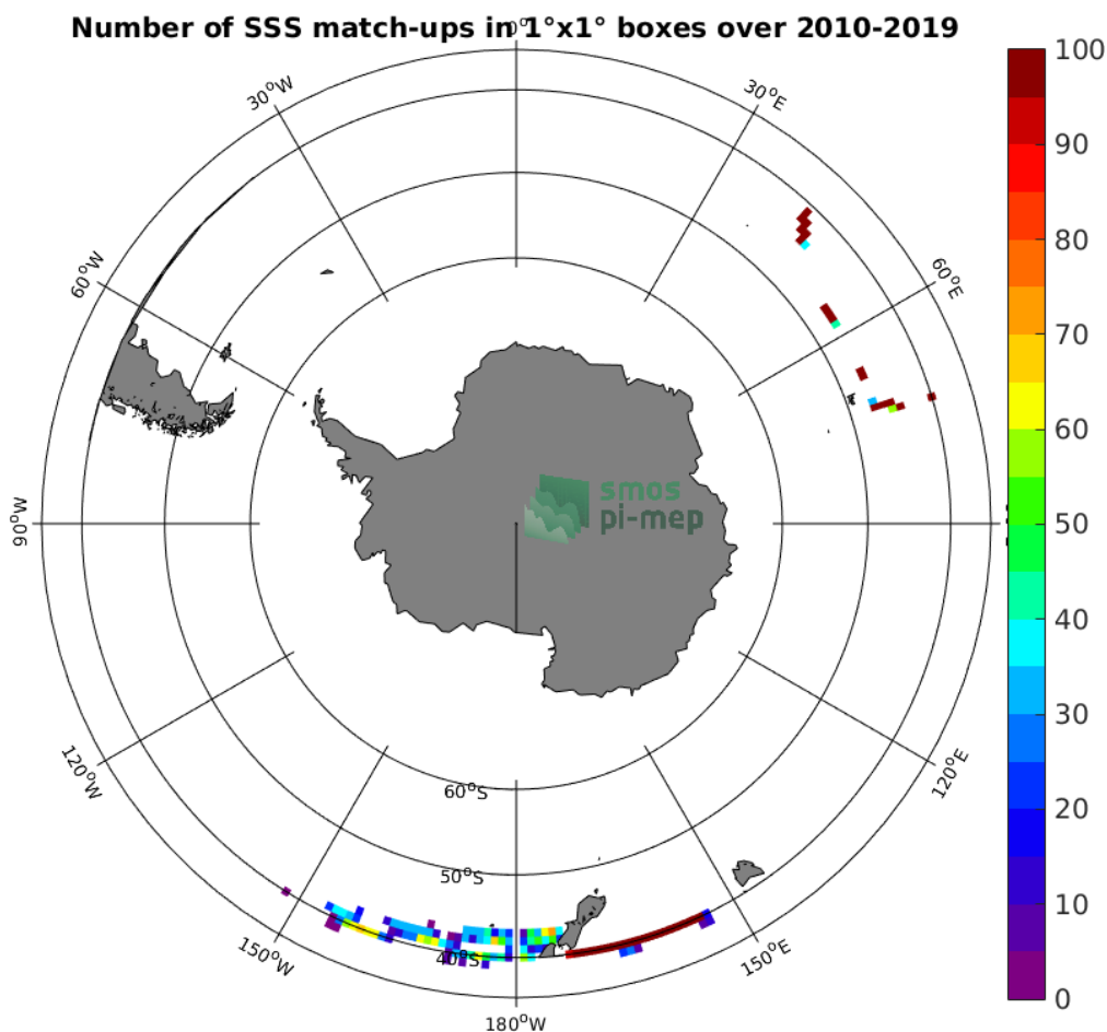
Figure 4: Number of SSS match-ups between TSG (LEGOS-DM) SSS and the SMOS SSS L2 v662 (ESA) SSS product for the Roaring Forties and Furious Fifties Pi-MEP region over 1°x1° boxes and for the full satellite product period.
