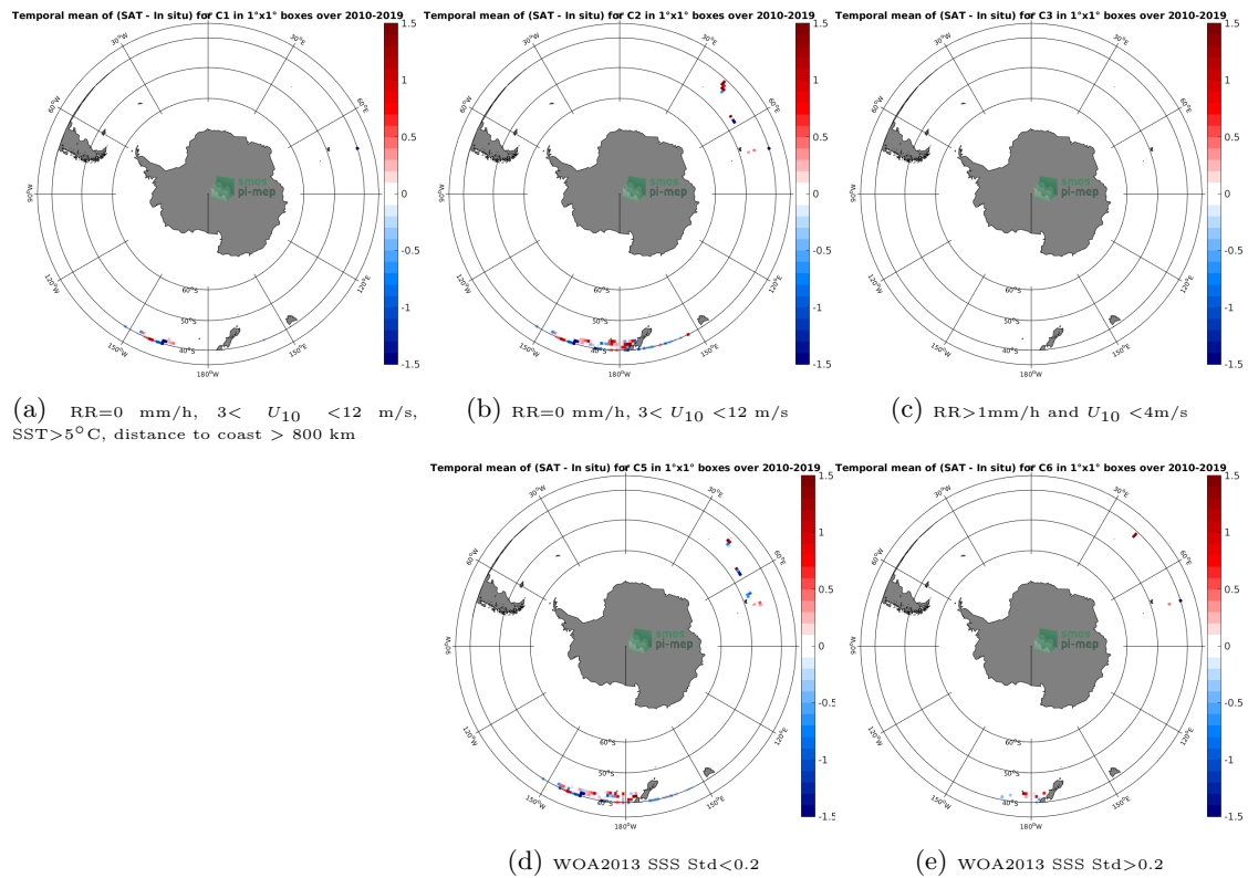
Figure 12: Temporal mean gridded over spatial boxes of size 1^{\circ}\times 1^{\circ} of \Delta\text{SSS} (SMOS L2 v662 (ESA) - TSG-LEGOS-DM) for 5 different subdatasets corresponding to:RR=0 mm/h, 3 < U_{10} < 12 m/s, SST >5^{\circ}\text{C} , distance to coast > 800 km (a), RR=0 mm/h, 3 < U_{10} < 12 m/s (b), RR >1 mm/h and U_{10} < 4 m/s (c), WOA2013 SSS Std <0.2 (d), WOA2013 SSS Std >0.2 (e).
