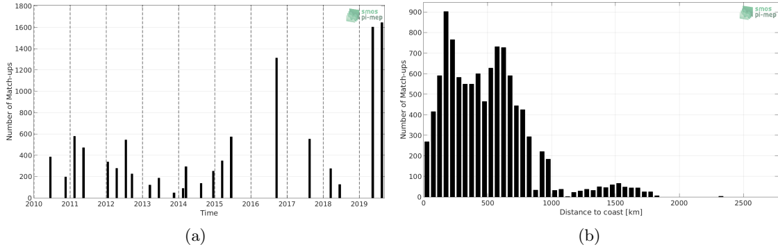
Figure 1: Number of match-ups between TSG-LEGOS-DM and SMOS L2 v662 (ESA) SSS as a function of time (a) and as function of the distance to coast (b) over the Roaring Forties and Furious Fifties Pi-MEP region and for the full satellite product period.
