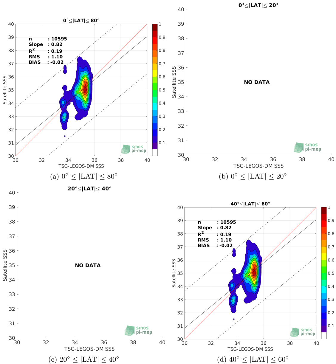
Figure 9: Contour maps of the concentration of SMOS L2 v662 (ESA) SSS (y-axis) versus TSG-LEGOS-DM SSS (x-axis) at match-up pairs for different latitude bands. For each plot, the red line shows x=y . The black thin and dashed lines indicate a linear fit through the data cloud and the \pm 95\% confidence levels, respectively. The number match-up pairs n , the slope and R^2 coefficient of the linear fit, the root mean square (RMS) and the mean bias between satellite and in situ data are indicated for each latitude band in each plots.
