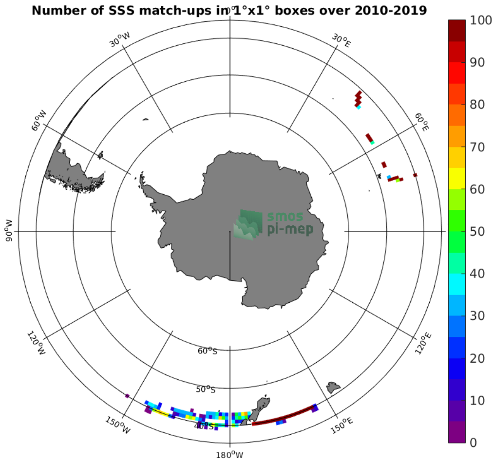
Figure 4: Number of SSS match-ups between TSG-LEGOS-DM SSS and the SMOS L2 v662 (ESA) SSS product for the Roaring Forties and Furious Fifties Pi-MEP region over 1°x1° boxes and for the full satellite product period.
