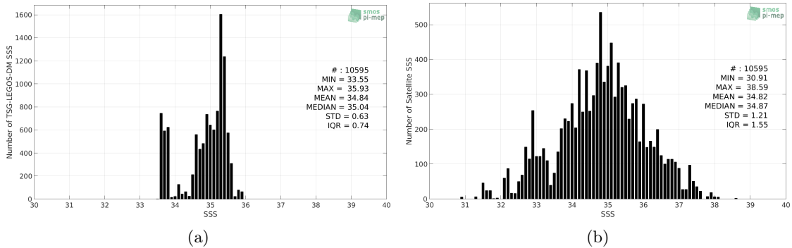
Figure 2: Histograms of SSS from TSG-LEGOS-DM (a) and SMOS L2 v662 (ESA) (b) considering all match-up pairs per bins of 0.1 over the Roaring Forties and Furious Fifties Pi-MEP region and for the full satellite product period.
