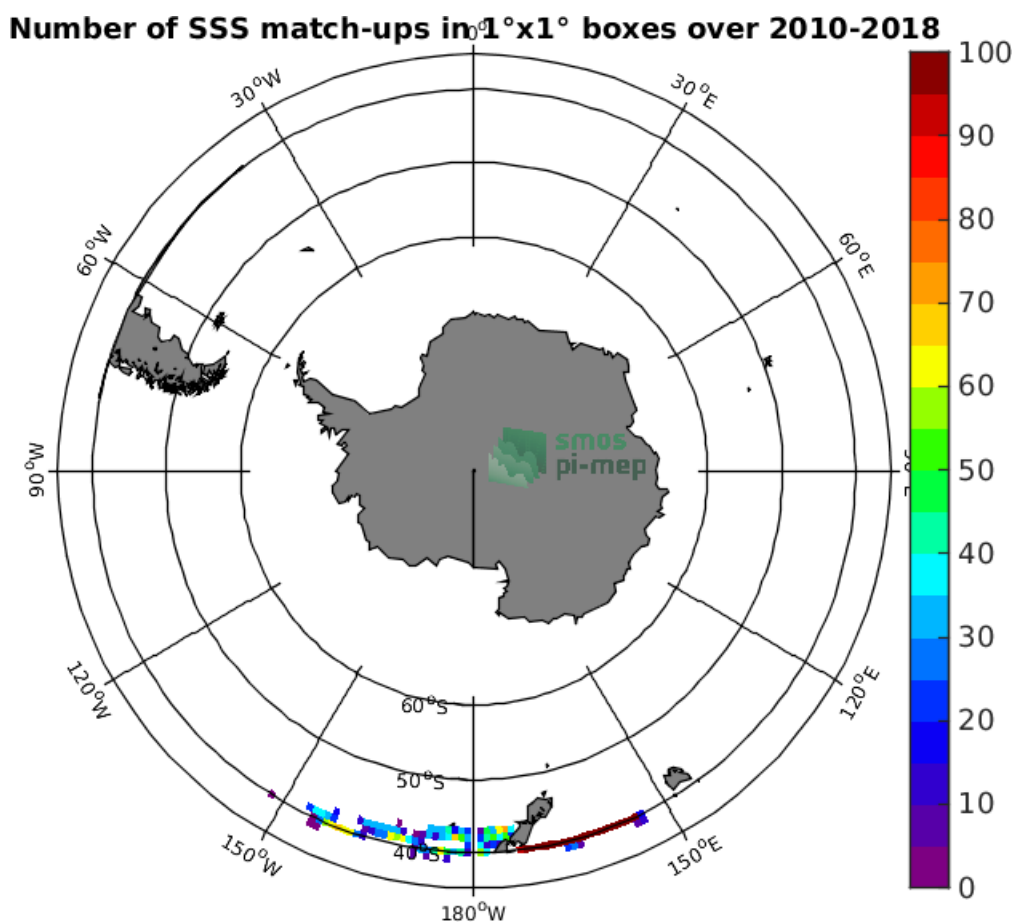
Figure 4: Number of SSS match-ups between TSG-LEGOS-DM SSS and the SMOS-L2-DPGS-v662 SSS product for the Roaring Forties and Furious Fifties Pi-MEP region over 1^\circ \times 1^\circ boxes and for the full satellite product period.
