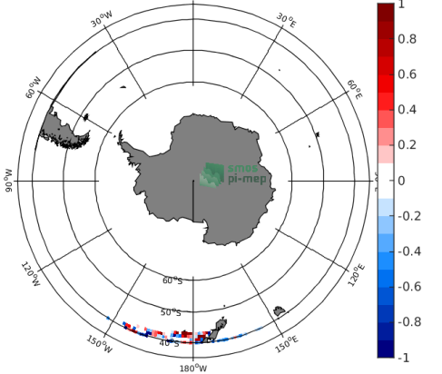
(e) MEAN( \Delta SSS) (Satellite - TSG-LEGOS-DM)
