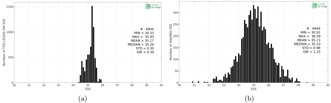
Figure 2: Histograms of SSS from TSG-LEGOS-DM (a) and SMOS-L2-DPGS-v662 (b) considering all match-up pairs per bins of 0.1 over the Roaring Forties and Furious Fifties Pi-MEP region and for the full satellite product period.
