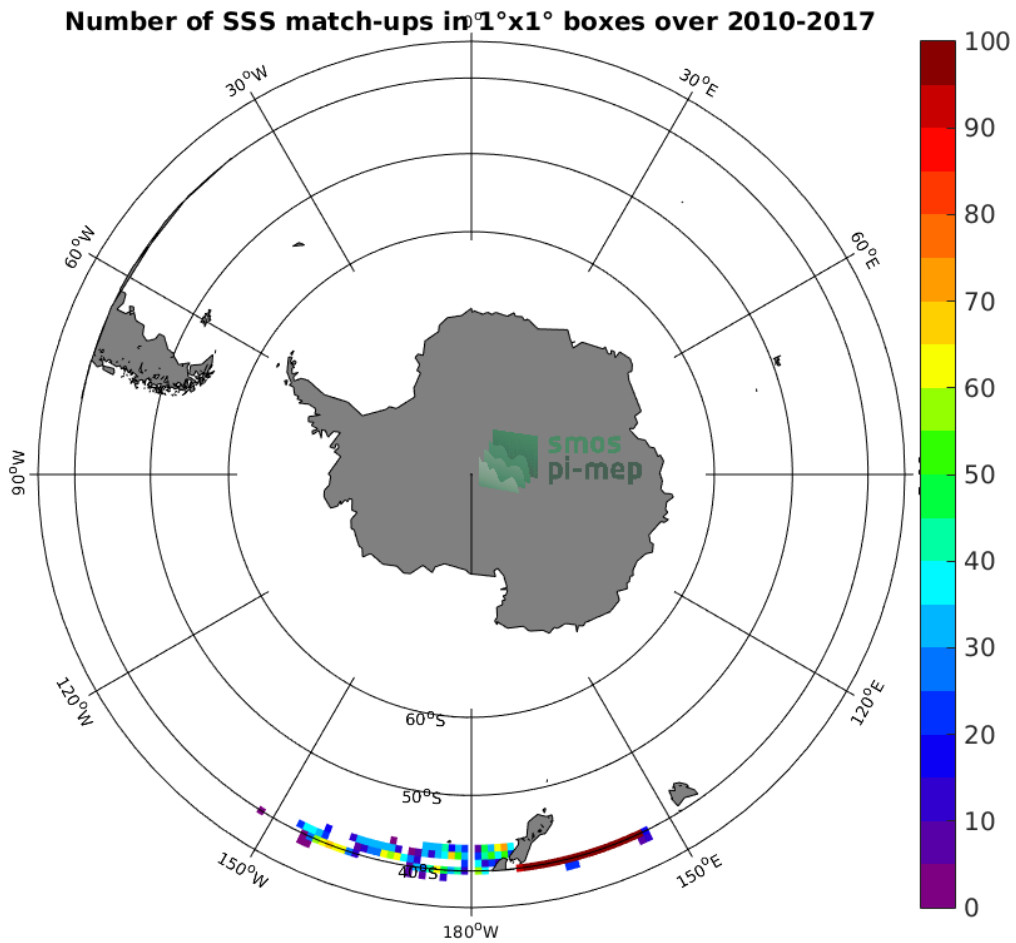
Figure 4: Number of SSS match-ups between TSG-LEGOS-DM SSS and the SMOS-L2-DPGS-v662 SSS product for the Roaring Forties and Furious Fifties Pi-MEP region over 1°x1° boxes and for the full satellite product period.
