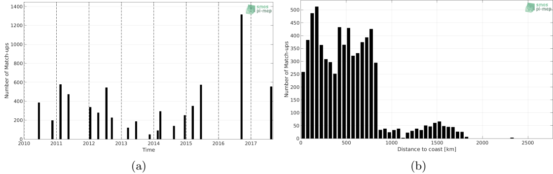
Figure 1: Number of match-ups between TSG-LEGOS-DM and SMOS-L2-DPGS-v662 SSS as a function of time (a) and as function of the distance to coast (b) over the Roaring Forties and Furious Fifties Pi-MEP region and for the full satellite product period.
