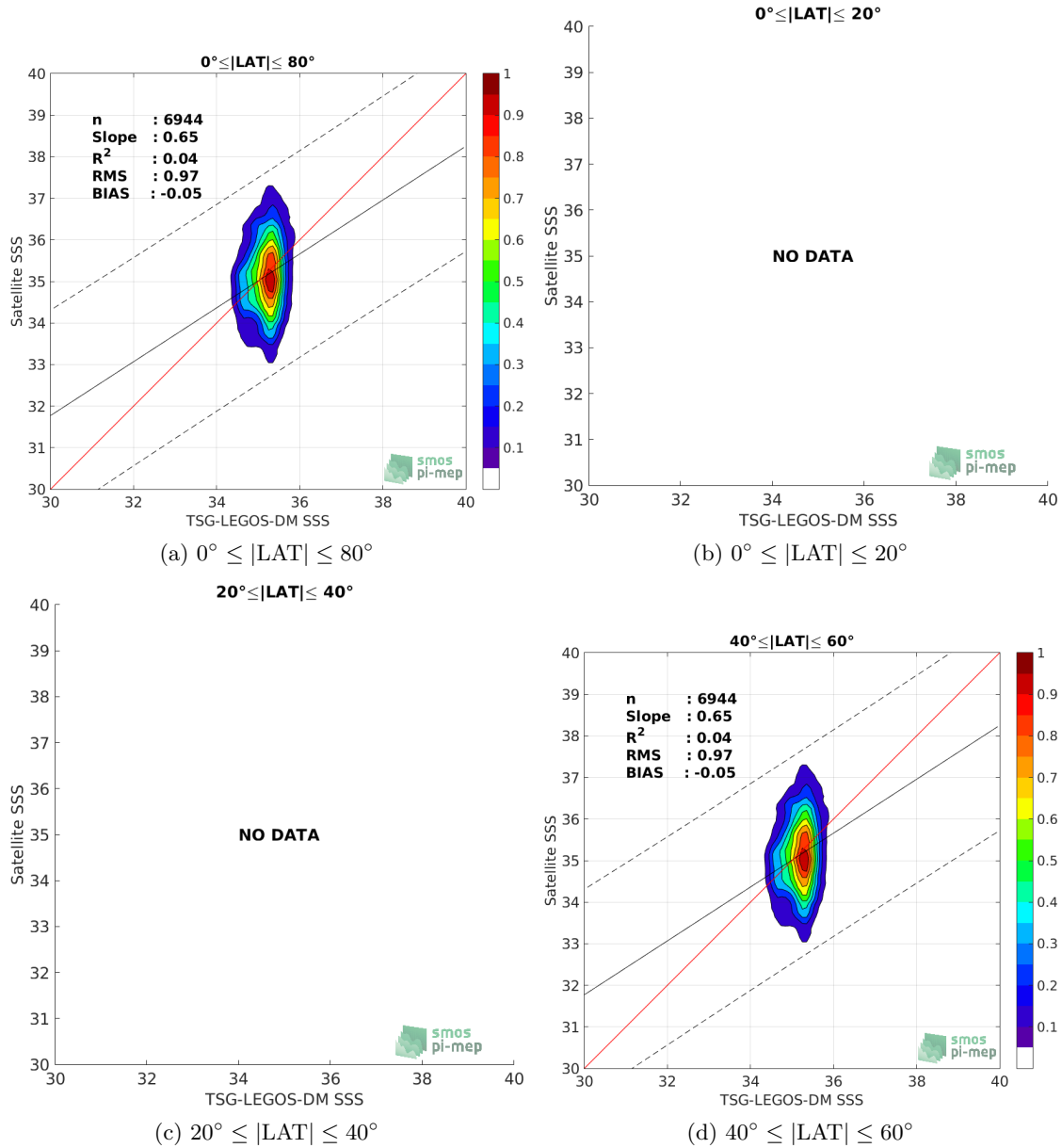
Figure 9: Contour maps of the concentration of SMOS-L2-DPGS-v662 SSS (y-axis) versus TSG-LEGOS-DM SSS (x-axis) at match-up pairs for different latitude bands. For each plot, the red line shows x=y . The black thin and dashed lines indicate a linear fit through the data cloud and the \pm 95\% confidence levels, respectively. The number match-up pairs n , the slope and R^2 coefficient of the linear fit, the root mean square (RMS) and the mean bias between satellite and in situ data are indicated for each latitude band in each plots.
