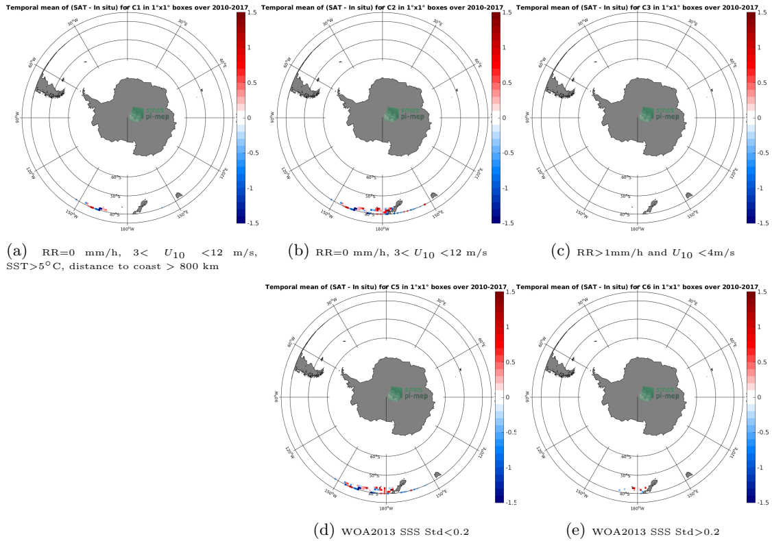
Figure 12: Temporal mean gridded over spatial boxes of size 1^\circ \times 1^\circ of \Delta SSS (SMOS-L2-DPGS-v662 - TSG-LEGOS-DM) for 5 different subdatasets corresponding to:RR=0 mm/h, 3 < U_{10} < 12 m/s, SST >5^\circ C, distance to coast > 800 km (a), RR=0 mm/h, 3 < U_{10} < 12 m/s (b), RR >1 mm/h and U_{10} < 4 m/s (c), WOA2013 SSS Std <0.2 (d), WOA2013 SSS Std >0.2 (e).
