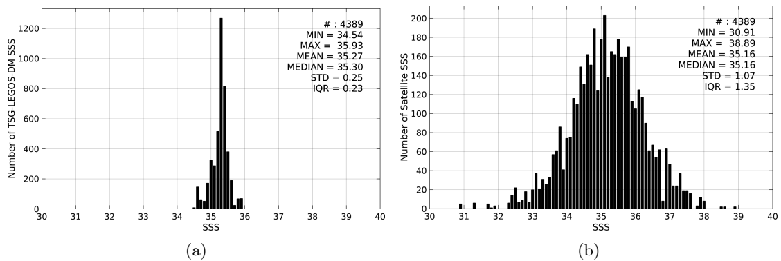
Figure 2: Histograms of SSS from TSG-LEGOS-DM (a) and SMOS-L2-DPGS-v662 (b) considering all match-up pairs per bins of 0.1 over the Roaring Forties and Furious Fifties Pi-MEP region and for the full satellite product period.
