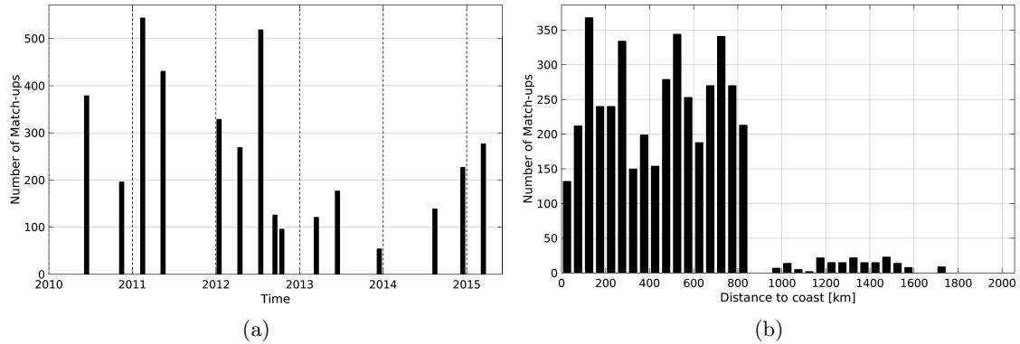
Figure 1: Number of match-ups between TSG-LEGOS-DM and SMOS-L2-DPGS-v662 SSS as a function of time (a) and as function of the distance to coast (b) over the Roaring Forties and Furious Fifties Pi-MEP region and for the full satellite product period.
