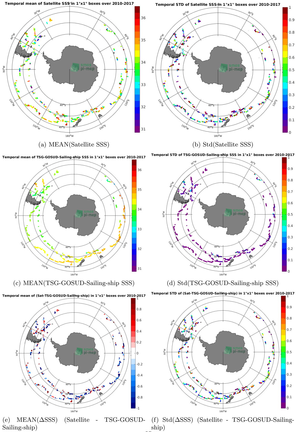
Figure 6: Temporal mean (left) and Std (right) of SSS from SMOS-L2-DPGS-v662 (top), TSG-GOSUD-Sailing-ship (middle), and of \Delta SSS (Satellite - TSG-GOSUD-Sailing-ship). Only match-up pairs are used to generate these maps.
