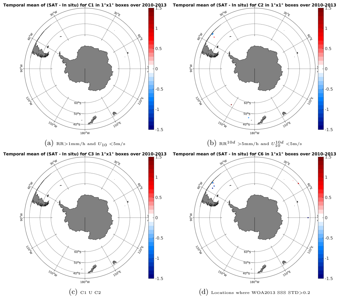
Figure 12: Temporal mean gridded over spatial boxes of size 1^\circ \times 1^\circ of \Delta SSS (SMOS-L2-DPGS-v662 - TSG-GOSUD-Sailing-ship) for 4 different subdatasets corresponding to:RR >1 mm/h and U_{10} < 5 m/s (a), RR 10d > 5 mm/h and U_{10}^{10d} < 5 m/s (b), C1 U C2 (c),Locations where WOA2013 SSS STD >0.2 (d).
