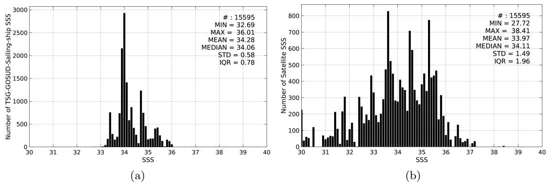
Figure 2: Histograms of SSS from TSG-GOSUD-Sailing-ship (a) and SMOS-L2-DPGS-v662 (b) considering all match-up pairs per bins of 0.1 over the Roaring Forties and Furious Fifties Pi-MEP region and for the full satellite product period.
