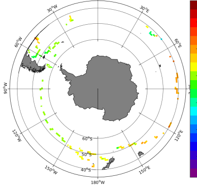
(c) MEAN(TSG-GOSUD-Sailing-ship SSS)
