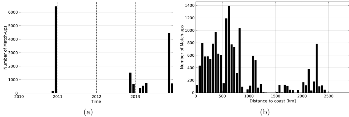
Figure 1: Number of match-ups between TSG-GOSUD-Sailing-ship and SMOS-L2-DPGS-v662 SSS as a function of time (a) and as function of the distance to coast (b) over the Roaring Forties and Furious Fifties Pi-MEP region and for the full satellite product period.
