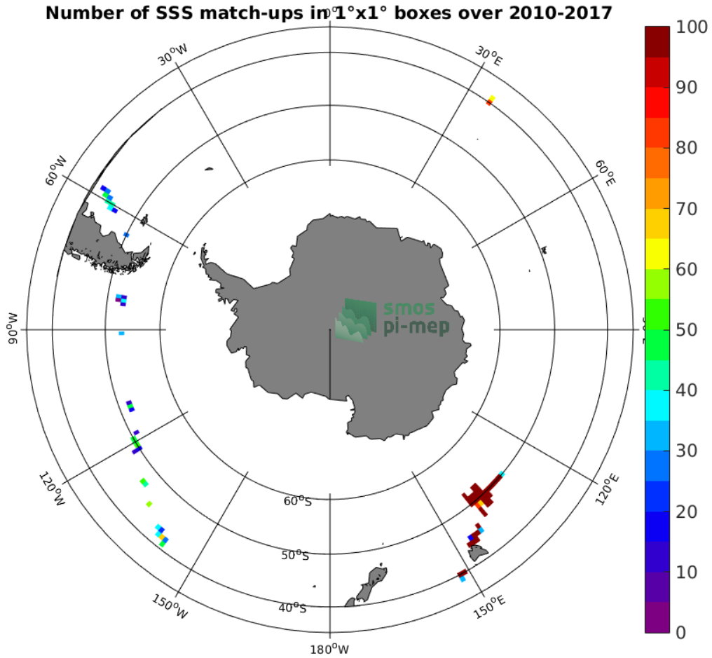
Figure 4: Number of SSS match-ups between TSG (GOSUD-Research-vessel) SSS and the SMOS SSS L2 v662 (ESA) SSS product for the Roaring Forties and Furious Fifties Pi-MEP region over 1°x1° boxes and for the full satellite product period.
