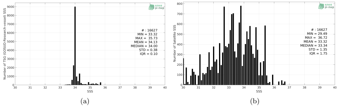
Figure 2: Histograms of SSS from TSG (GOSUD-Research-vessel) (a) and SMOS SSS L2 v662 (ESA) (b) considering all match-up pairs per bins of 0.1 over the Roaring Forties and Furious Fifties Pi-MEP region and for the full satellite product period.
