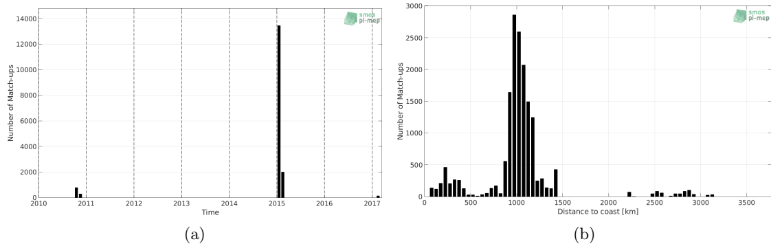
Figure 1: Number of match-ups between TSG (GOSUD-Research-vessel) and SMOS SSS L2 v662 (ESA) SSS as a function of time (a) and as function of the distance to coast (b) over the Roaring Forties and Furious Fifties Pi-MEP region and for the full satellite product period.
