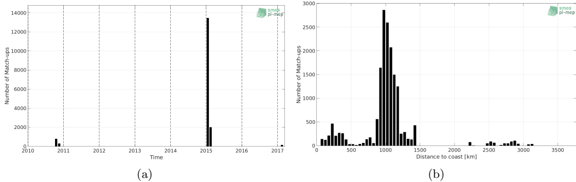
Figure 1: Number of match-ups between TSG-GOSUD-Research-vessel and SMOS L2 v662 (ESA) SSS as a function of time (a) and as function of the distance to coast (b) over the Roaring Forties and Furious Fifties Pi-MEP region and for the full satellite product period.
