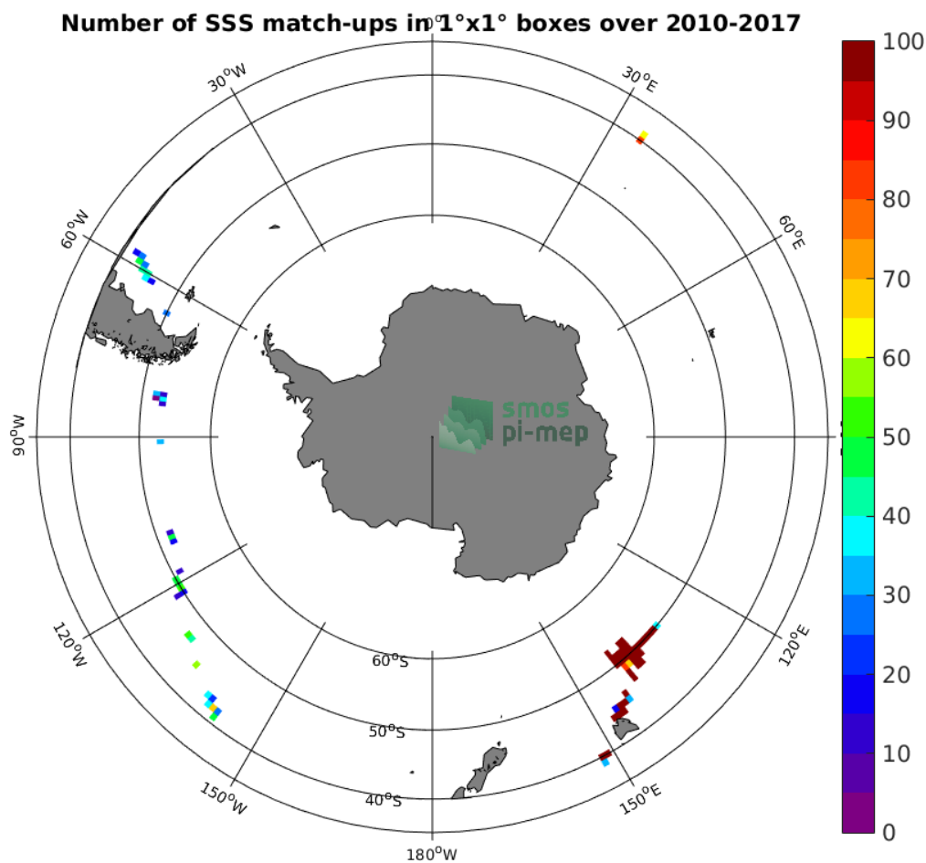
Figure 4: Number of SSS match-ups between TSG-GOSUD-Research-vessel SSS and the SMOS L2 v662 (ESA) SSS product for the Roaring Forties and Furious Fifties Pi-MEP region over 1°x1° boxes and for the full satellite product period.
