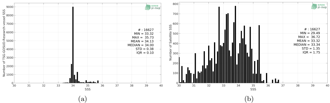
Figure 2: Histograms of SSS from TSG-GOSUD-Research-vessel (a) and SMOS L2 v662 (ESA) (b) considering all match-up pairs per bins of 0.1 over the Roaring Forties and Furious Fifties Pi-MEP region and for the full satellite product period.
