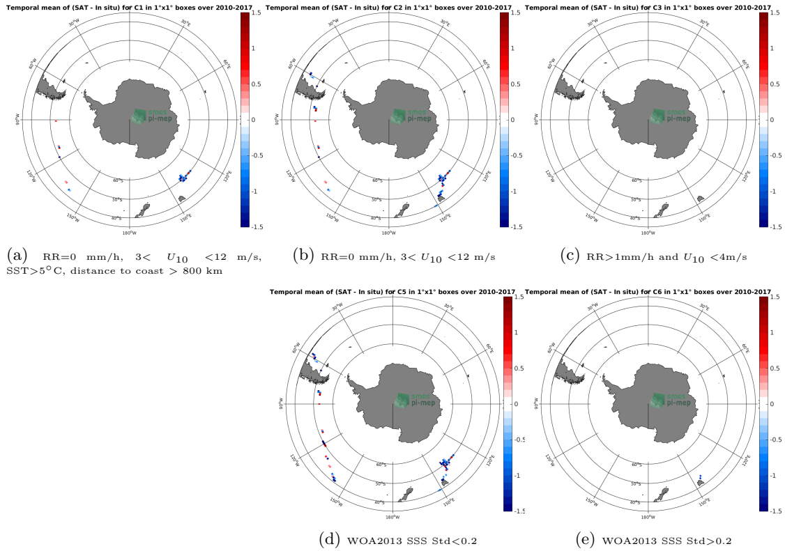
Figure 12: Temporal mean gridded over spatial boxes of size 1°x1° of \Delta SSS (SMOS L2 v662 (ESA) - TSG-GOSUD-Research-vessel) for 5 different subdatasets corresponding to:RR=0 mm/h, 3 < U_{10} < 12 m/s, SST>5°C, distance to coast > 800 km (a), RR=0 mm/h, 3 < U_{10} < 12 m/s (b), RR>1mm/h and U_{10} < 4 m/s (c), WOA2013 SSS Std<0.2 (d), WOA2013 SSS Std>0.2 (e).
