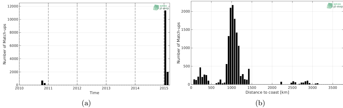
Figure 1: Number of match-ups between TSG-GOSUD-Research-vessel and SMOS-L2-DPGS-v662 SSS as a function of time (a) and as function of the distance to coast (b) over the Roaring Forties and Furious Fifties Pi-MEP region and for the full satellite product period.
