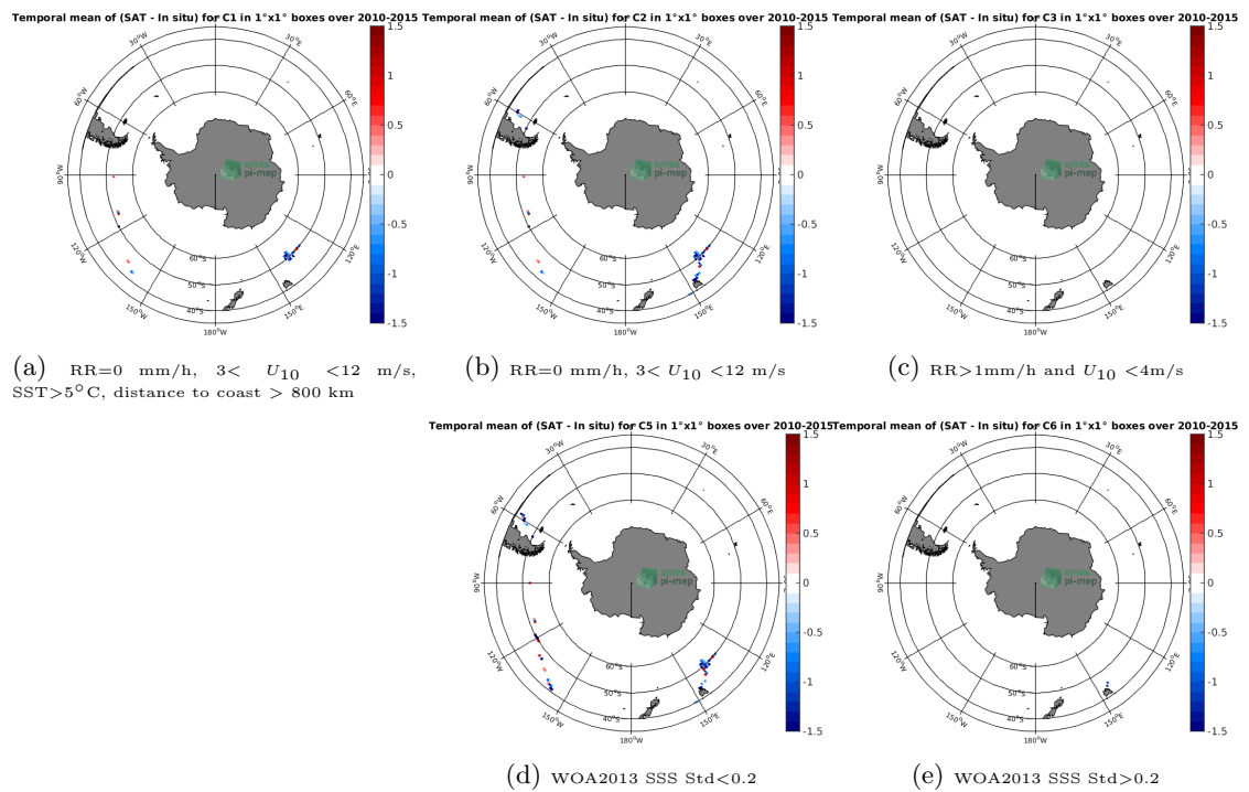
Figure 12: Temporal mean gridded over spatial boxes of size 1^\circ \times 1^\circ of \Delta SSS (SMOS-L2-DPGS-v662 - TSG-GOSUD-Research-vessel) for 5 different subdatasets corresponding to:RR=0 mm/h, 3 < U_{10} < 12 m/s, SST>5°C, distance to coast > 800 km (a), RR=0 mm/h, 3 < U_{10} < 12 m/s (b), RR>1mm/h and U_{10} < 4 m/s (c), WOA2013 SSS Std<0.2 (d), WOA2013 SSS Std>0.2 (e).
