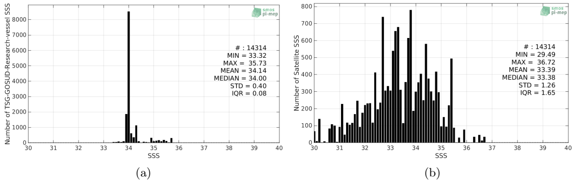
Figure 2: Histograms of SSS from TSG-GOSUD-Research-vessel (a) and SMOS-L2-DPGS-v662 (b) considering all match-up pairs per bins of 0.1 over the Roaring Forties and Furious Fifties Pi-MEP region and for the full satellite product period.
