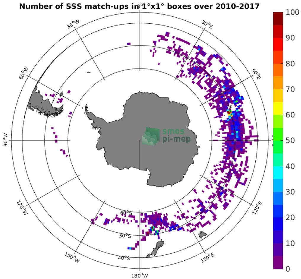
Figure 4: Number of SSS match-ups between Sea mammals SSS and the SMOS SSS L2 v662 (ESA) SSS product for the Roaring Forties and Furious Fifties Pi-MEP region over 1^\circ \times 1^\circ boxes and for the full satellite product period.
