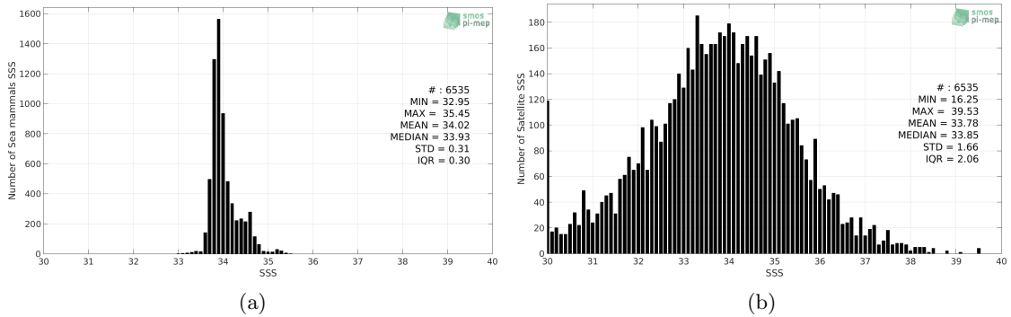
Figure 2: Histograms of SSS from Sea mammals (a) and SMOS SSS L2 v662 (ESA) (b) considering all match-up pairs per bins of 0.1 over the Roaring Forties and Furious Fifties Pi-MEP region and for the full satellite product period.
