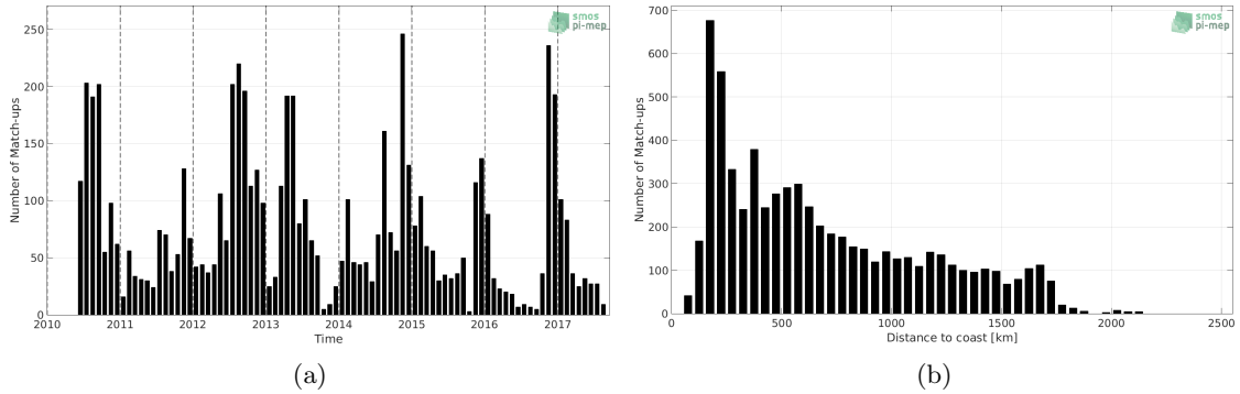
Figure 1: Number of match-ups between Sea mammals and SMOS SSS L2 v662 (ESA) SSS as a function of time (a) and as function of the distance to coast (b) over the Roaring Forties and Furious Fifties Pi-MEP region and for the full satellite product period.
