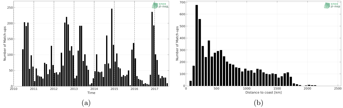
Figure 1: Number of match-ups between Sea mammals and SMOS L2 v662 (ESA) SSS as a function of time (a) and as function of the distance to coast (b) over the Roaring Forties and Furious Fifties Pi-MEP region and for the full satellite product period.
