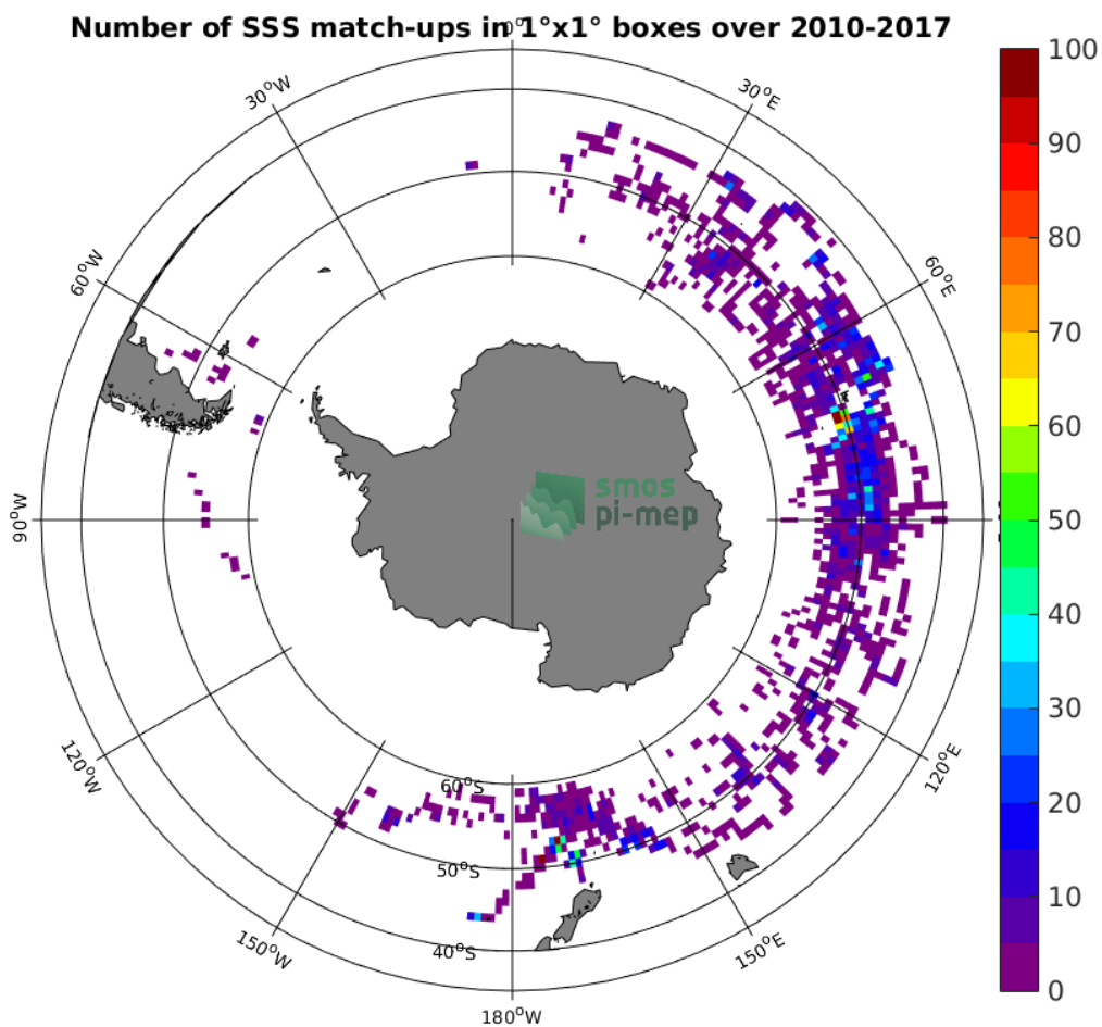
Figure 4: Number of SSS match-ups between Sea mammals SSS and the SMOS L2 v662 (ESA) SSS product for the Roaring Forties and Furious Fifties Pi-MEP region over 1^\circ \times 1^\circ boxes and for the full satellite product period.
