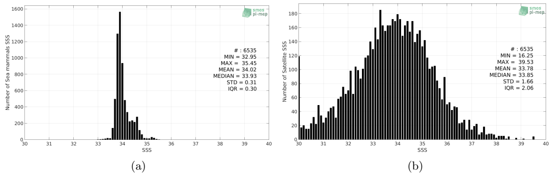
Figure 2: Histograms of SSS from Sea mammals (a) and SMOS L2 v662 (ESA) (b) considering all match-up pairs per bins of 0.1 over the Roaring Forties and Furious Fifties Pi-MEP region and for the full satellite product period.
