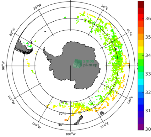
(c) MEAN(Sea mammals SSS)
