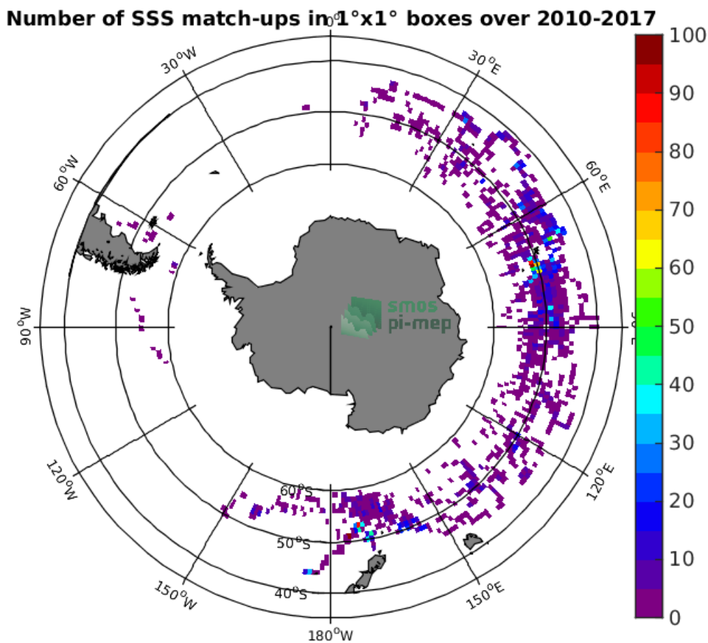
Figure 4: Number of SSS match-ups between Sea mammals SSS and the SMOS-L2-DPGS-v662 SSS product for the Roaring Forties and Furious Fifties Pi-MEP region over 1°x1° boxes and for the full satellite product period.
