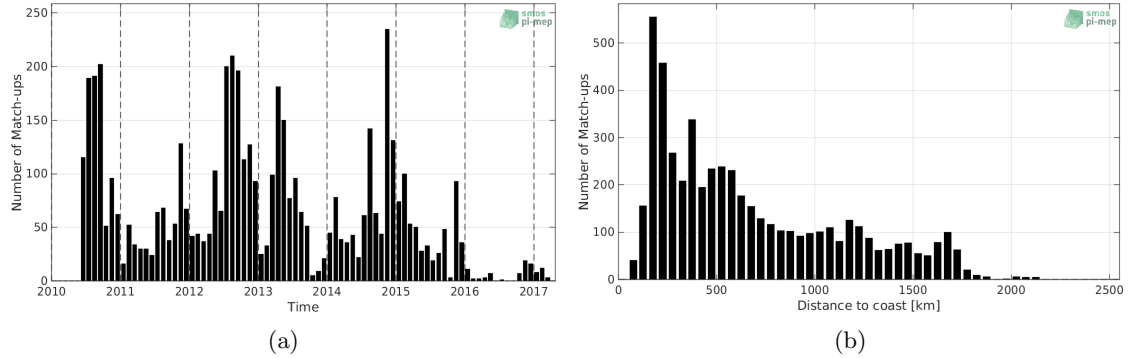
Figure 1: Number of match-ups between Sea mammals and SMOS-L2-DPGS-v662 SSS as a function of time (a) and as function of the distance to coast (b) over the Roaring Forties and Furious Fifties Pi-MEP region and for the full satellite product period.
