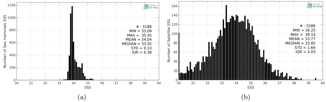
Figure 2: Histograms of SSS from Sea mammals (a) and SMOS-L2-DPGS-v662 (b) considering all match-up pairs per bins of 0.1 over the Roaring Forties and Furious Fifties Pi-MEP region and for the full satellite product period.
