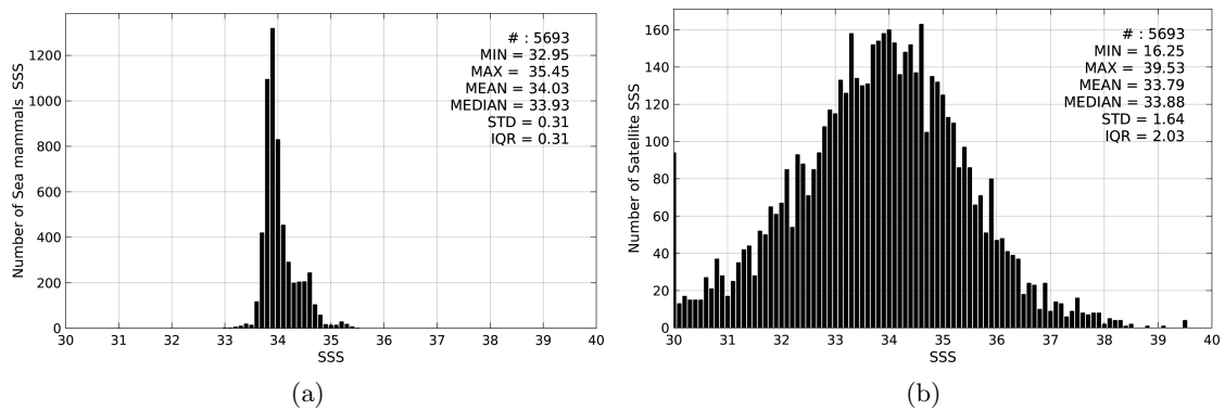
Figure 2: Histograms of SSS from Sea mammals (a) and SMOS-L2-DPGS-v662 (b) considering all match-up pairs per bins of 0.1 over the Roaring Forties and Furious Fifties Pi-MEP region and for the full satellite product period.
