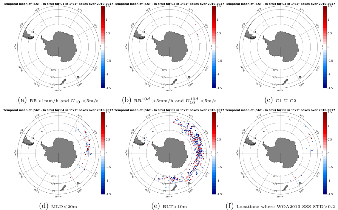
Figure 12: Temporal mean gridded over spatial boxes of size 1^\circ \times 1^\circ of \Delta SSS (SMOS-L2-DPGS-v662 - Sea mammals) for 6 different subdatasets corresponding to: RR > 1\text{mm/h} and U_{10} < 5\text{m/s} (a), RR^{10d} > 5\text{mm/h} and U_{10}^{10d} < 5\text{m/s} (b), C1 U C2 (c), MLD < 20\text{m} (d), BLT > 10\text{m} (e), Locations where WOA2013 SSS STD > 0.2 (f).
