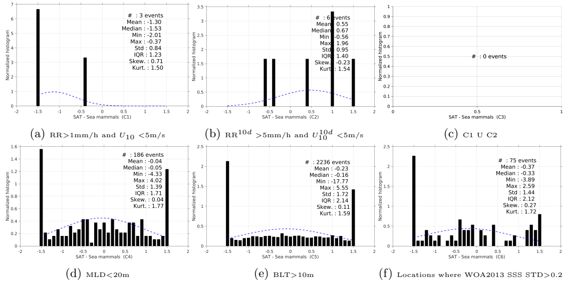
Figure 13: Normalized histogram of \Delta SSS (SMOS-L2-DPGS-v662 - Sea mammals) for 6 different subdatasets corresponding to: RR > 1mm/h and U_{10} < 5 m/s (a), RR^{10d} > 5 mm/h and U_{10}^{10d} < 5 m/s (b), C1 U C2 (c), MLD < 20m (d), BLT > 10m (e), Locations where WOA2013 SSS STD > 0.2 (f).
