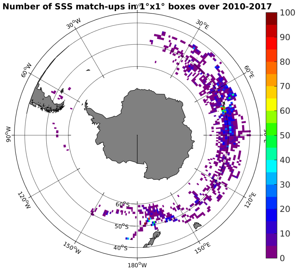
Figure 4: Number of SSS match-ups between Sea mammals SSS and the SMOS-L2-DPGS-v662 SSS product for the Roaring Forties and Furious Fifties Pi-MEP region over 1^\circ \times 1^\circ boxes and for the full satellite product period.
