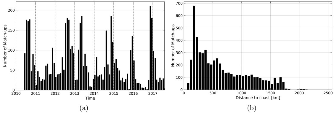
Figure 1: Number of match-ups between Sea mammals and SMOS-L2-DPGS-v662 SSS as a function of time (a) and as function of the distance to coast (b) over the Roaring Forties and Furious Fifties Pi-MEP region and for the full satellite product period.
