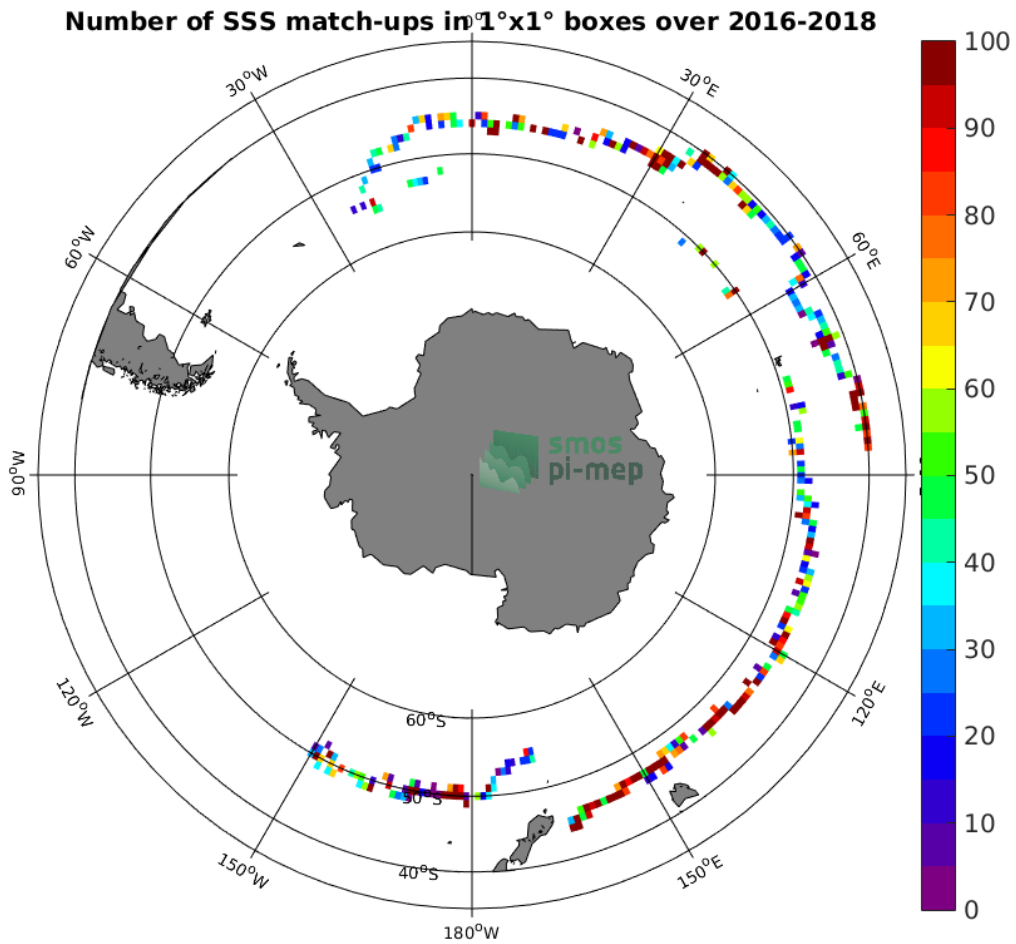
Figure 3: Number of SSS match-ups between Surface drifters SSS and the SMOS SSS L2 v662 (ESA) SSS product for the Roaring Forties and Furious Fifties Pi-MEP region over 1°x1° boxes and for the full satellite product period.
