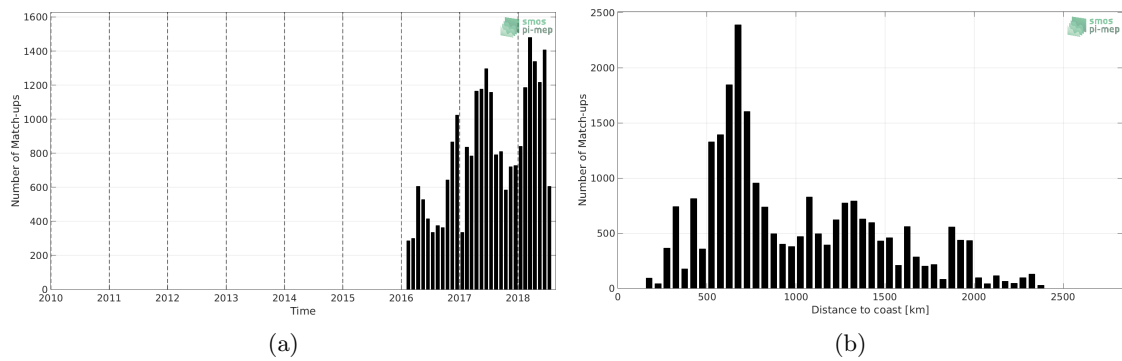
Figure 1: Number of match-ups between Surface drifters and SMOS SSS L2 v662 (ESA) SSS as a function of time (a) and as function of the distance to coast (b) over the Roaring Forties and Furious Fifties Pi-MEP region and for the full satellite product period.
