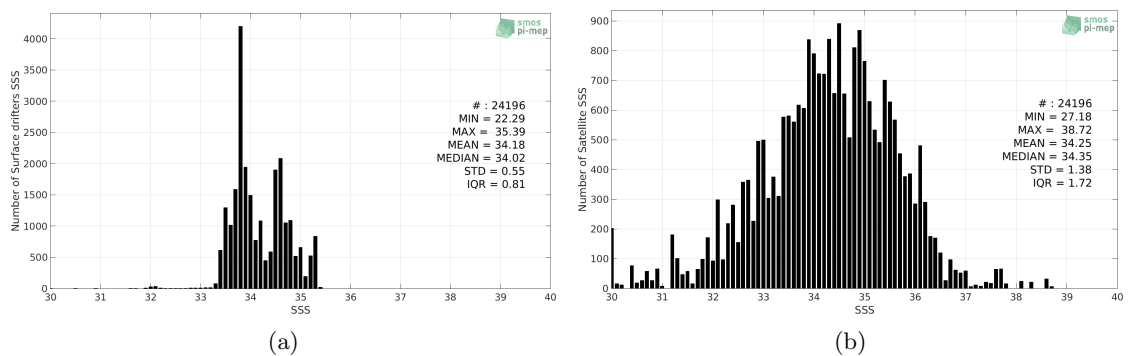
Figure 2: Histograms of SSS from Surface drifters (a) and SMOS SSS L2 v662 (ESA) (b) considering all match-up pairs per bins of 0.1 over the Roaring Forties and Furious Fifties Pi-MEP region and for the full satellite product period.
