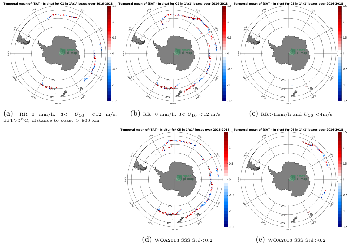
Figure 11: Temporal mean gridded over spatial boxes of size 1^{\circ}\times 1^{\circ} of \Delta\text{SSS} (SMOS L2 v662 (ESA) - Surface drifters) for 5 different subdatasets corresponding to:RR=0 mm/h, 3 < U_{10} < 12 m/s, SST > 5^{\circ}\text{C} , distance to coast > 800 km (a), RR=0 mm/h, 3 < U_{10} < 12 m/s (b), RR > 1 mm/h and U_{10} < 4 m/s (c), WOA2013 SSS Std < 0.2 (d), WOA2013 SSS Std > 0.2 (e).
