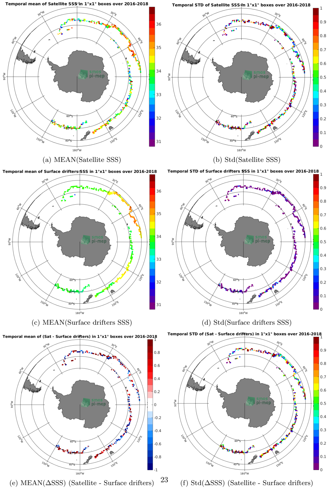
Figure 5: Temporal mean (left) and Std (right) of SSS from SMOS L2 v662 (ESA) (top), Surface drifters (middle), and of \Delta SSS (Satellite - Surface drifters). Only match-up pairs are used to generate these maps.
