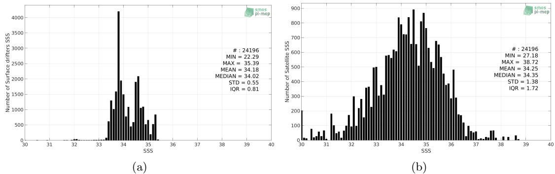
Figure 2: Histograms of SSS from Surface drifters (a) and SMOS L2 v662 (ESA) (b) considering all match-up pairs per bins of 0.1 over the Roaring Forties and Furious Fifties Pi-MEP region and for the full satellite product period.
