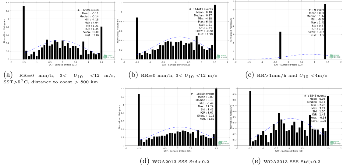
Figure 12: Normalized histogram of \Delta SSS (SMOS L2 v662 (ESA) - Surface drifters) for 5 different subdatasets corresponding to: RR=0 mm/h, 3 < U_{10} < 12 m/s, SST>5°C, distance to coast > 800 km (a), RR=0 mm/h, 3 < U_{10} < 12 m/s (b), RR>1mm/h and U_{10} < 4 m/s (c), WOA2013 SSS Std<0.2 (d), WOA2013 SSS Std>0.2 (e).
