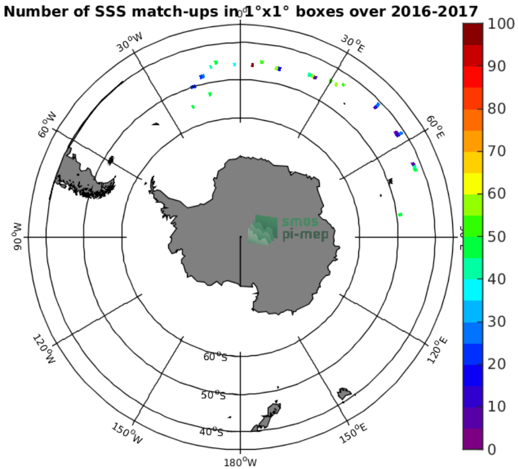
Figure 3: Number of SSS match-ups between Surface drifters SSS and the SMOS-L2-DPGS-v662 SSS product for the Roaring Forties and Furious Fifties Pi-MEP region over 1^\circ \times 1^\circ boxes and for the full satellite product period.
