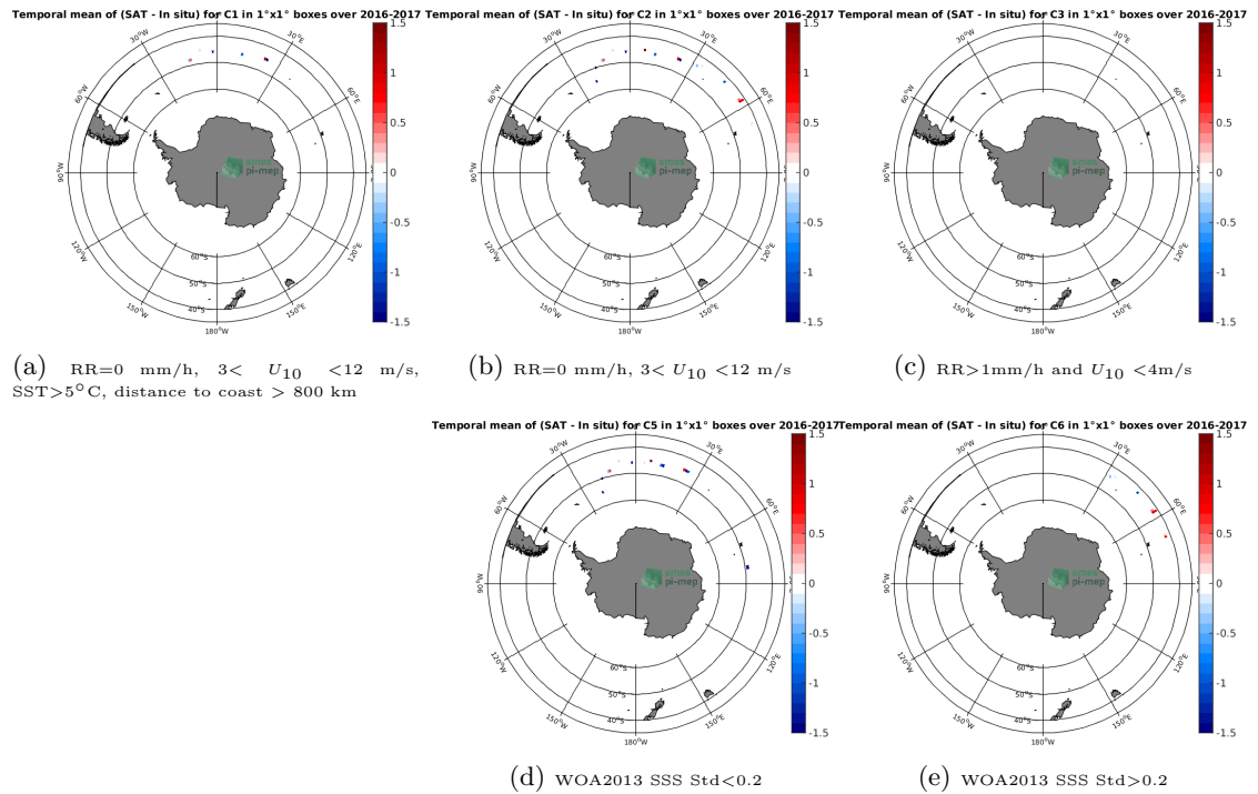
Figure 11: Temporal mean gridded over spatial boxes of size 1^\circ \times 1^\circ of \Delta SSS (SMOS-L2-DPGS-v662 - Surface drifters) for 5 different subdatasets corresponding to: RR=0 mm/h, 3 < U_{10} < 12 m/s, SST > 5^\circ\text{C} , distance to coast > 800 km (a), RR=0 mm/h, 3 < U_{10} < 12 m/s (b), RR > 1 mm/h and U_{10} < 4 m/s (c), WOA2013 SSS Std < 0.2 (d), WOA2013 SSS Std > 0.2 (e).
