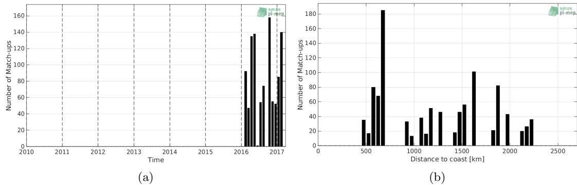
Figure 1: Number of match-ups between Surface drifters and SMOS-L2-DPGS-v662 SSS as a function of time (a) and as function of the distance to coast (b) over the Roaring Forties and Furious Fifties Pi-MEP region and for the full satellite product period.
