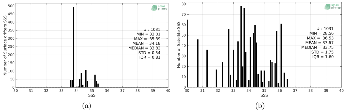
Figure 2: Histograms of SSS from Surface drifters (a) and SMOS-L2-DPGS-v662 (b) considering all match-up pairs per bins of 0.1 over the Roaring Forties and Furious Fifties Pi-MEP region and for the full satellite product period.
