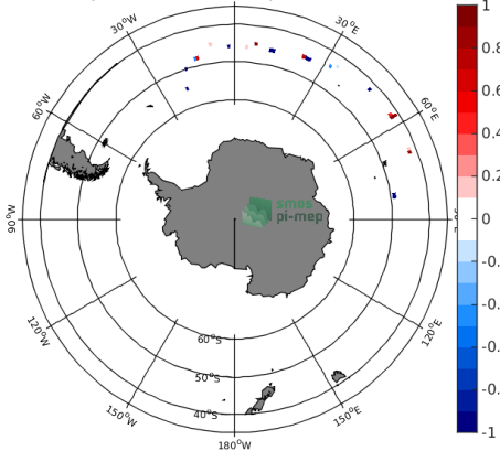
(e) MEAN( \Delta SSS) (Satellite - Surface drifters)
