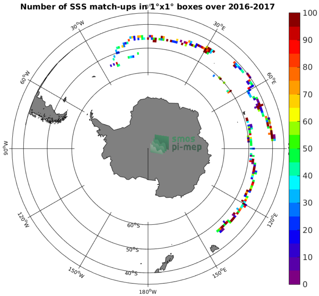
Figure 3: Number of SSS match-ups between Surface drifters SSS and the SMOS-L2-DPGS-v662 SSS product for the Roaring Forties and Furious Fifties Pi-MEP region over 1^\circ \times 1^\circ boxes and for the full satellite product period.
