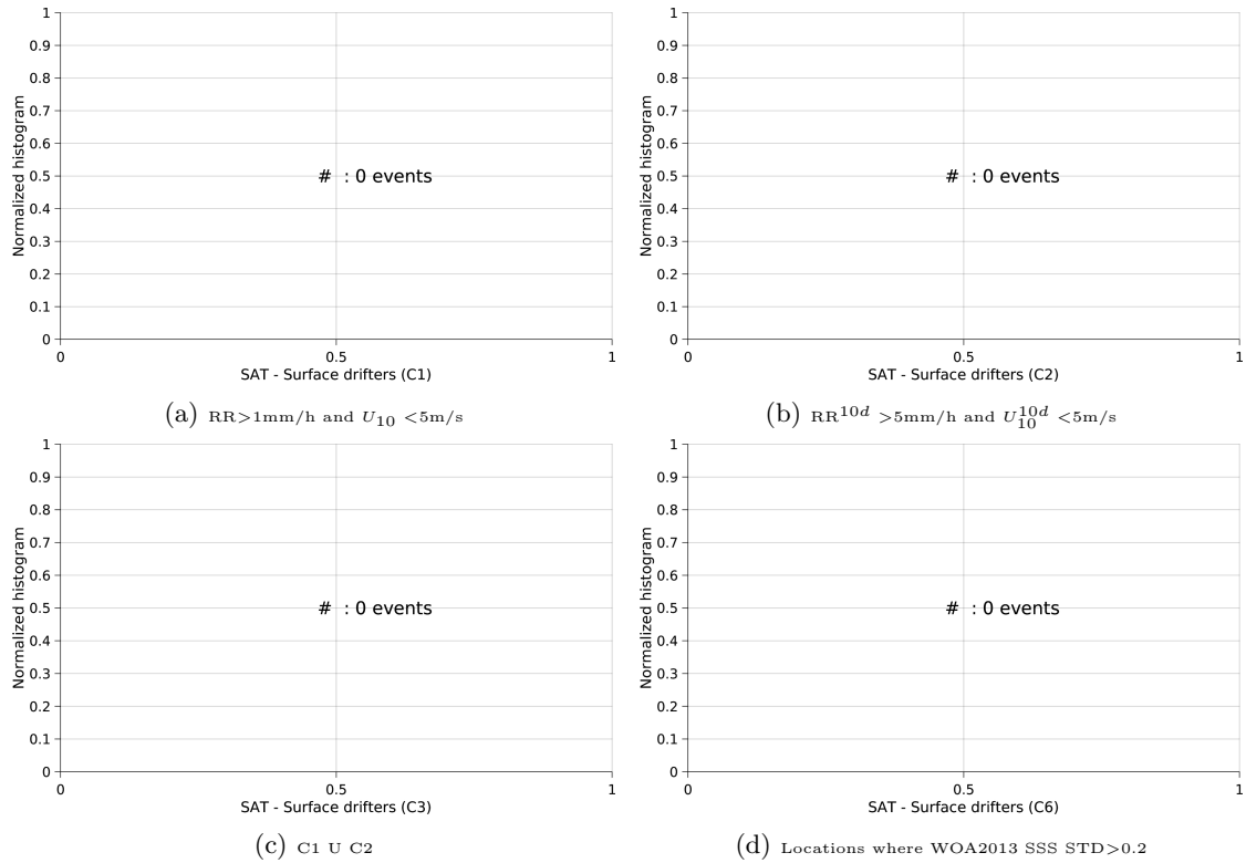
Figure 12: Normalized histogram of \Delta\text{SSS} (SMOS-L2-DPGS-v662 - Surface drifters) for 6 different subdatasets corresponding to: RR > 1\text{mm/h} and U_{10} < 5\text{m/s} (a), RR^{10d} > 5\text{mm/h} and U_{10}^{10d} < 5\text{m/s} (b), C1 \cup C2 (c), Locations where WOA2013 SSS STD > 0.2 (d).
