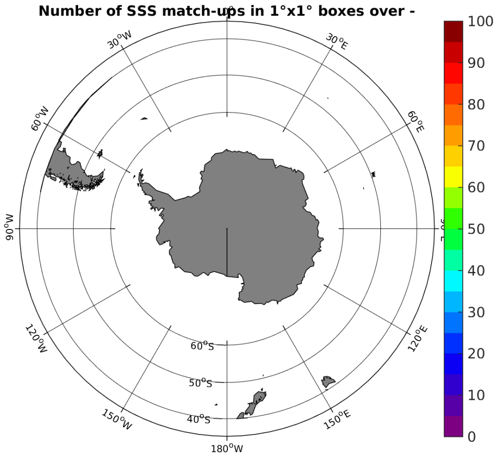
Figure 3: Number of SSS match-ups between Surface drifters SSS and the SMOS-L2-DPGS-v662 SSS product for the Roaring Forties and Furious Fifties Pi-MEP region over 1°x1° boxes and for the full satellite product period.
