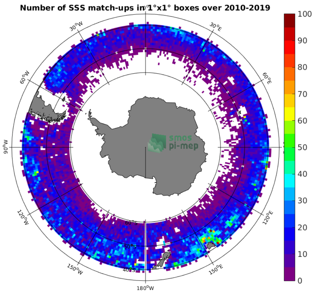
Figure 4: Number of SSS match-ups between Argo SSS and the SMOS-L2-DPGS-v662 SSS product for the Roaring Forties and Furious Fifties Pi-MEP region over 1^\circ \times 1^\circ boxes and for the full satellite product period.
