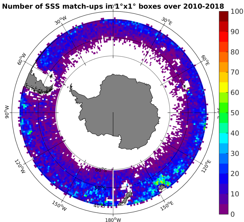
Figure 4: Number of SSS match-ups between Argo SSS and the SMOS-L2-DPGS-v662 SSS product for the Roaring Forties and Furious Fifties Pi-MEP region over 1^\circ \times 1^\circ boxes and for the full satellite product period.
