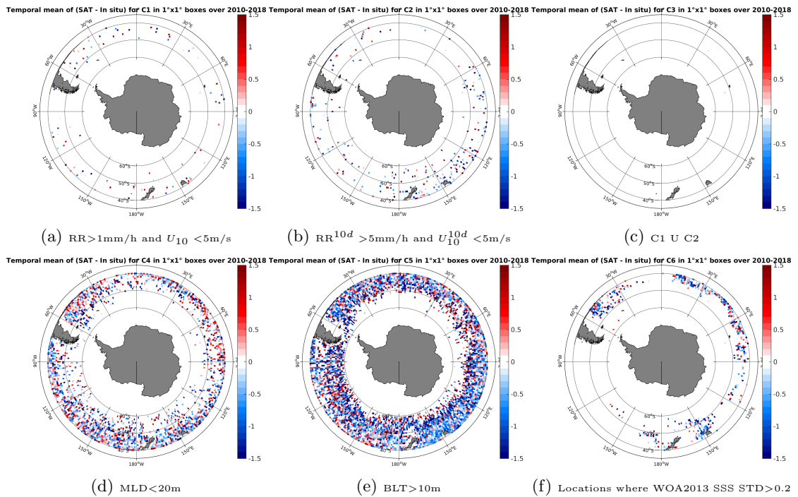
Figure 12: Temporal mean gridded over spatial boxes of size 1^\circ \times 1^\circ of \Delta SSS (SMOS-L2-DPGS-v662 - Argo) for 6 different subdatasets corresponding to: RR > 1\text{mm/h} and U_{10} < 5\text{m/s} (a), RR^{10d} > 5\text{mm/h} and U_{10}^{10d} < 5\text{m/s} (b), C1 U C2 (c), MLD < 20\text{m} (d), BLT > 10\text{m} (e), Locations where WOA2013 SSS STD > 0.2 (f).
