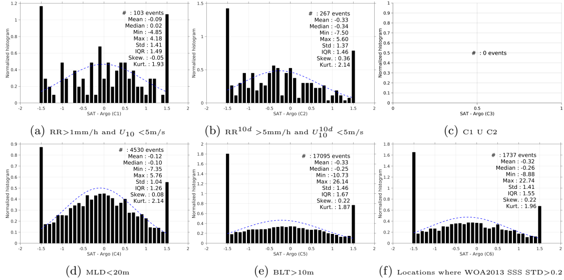
Figure 13: Normalized histogram of \Delta SSS (SMOS-L2-DPGS-v662 - Argo) for 6 different sub-datasets corresponding to: RR>1mm/h and U_{10} < 5\text{m/s} (a), RR^{10d} > 5\text{mm/h} and U_{10}^{10d} < 5\text{m/s} (b), C1 U C2 (c),MLD<20m (d),BLT>10m (e),Locations where WOA2013 SSS STD>0.2 (f).
