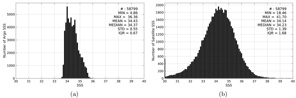
Figure 2: Histograms of SSS from Argo (a) and SMOS-L2-DPGS-v662 (b) considering all match-up pairs per bins of 0.1 over the Roaring Forties and Furious Fifties Pi-MEP region and for the full satellite product period.
