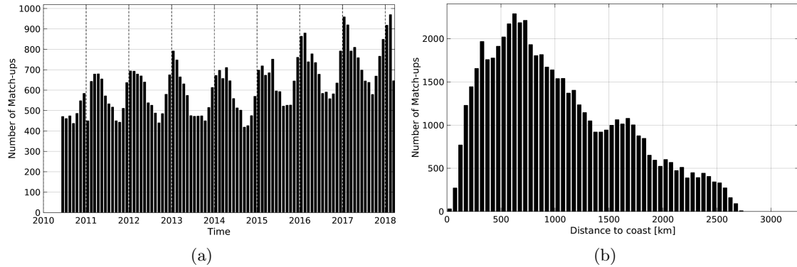
Figure 1: Number of match-ups between Argo and SMOS-L2-DPGS-v662 SSS as a function of time (a) and as function of the distance to coast (b) over the Roaring Forties and Furious Fifties Pi-MEP region and for the full satellite product period.
