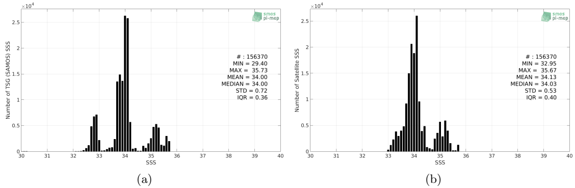
Figure 2: Histograms of SSS from TSG (SAMOS) (a) and SMAP SSS L4 OI v1 - 7day (IPRC) (b) considering all match-up pairs per bins of 0.1 over the Roaring Forties and Furious Fifties Pi-MEP region and for the full satellite product period.
