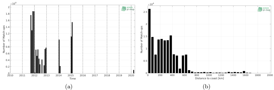
Figure 1: Number of match-ups between TSG (SAMOS) and SMAP SSS L4 OI v1 - 7day (IPRC) SSS as a function of time (a) and as function of the distance to coast (b) over the Roaring Forties and Furious Fifties Pi-MEP region and for the full satellite product period.
