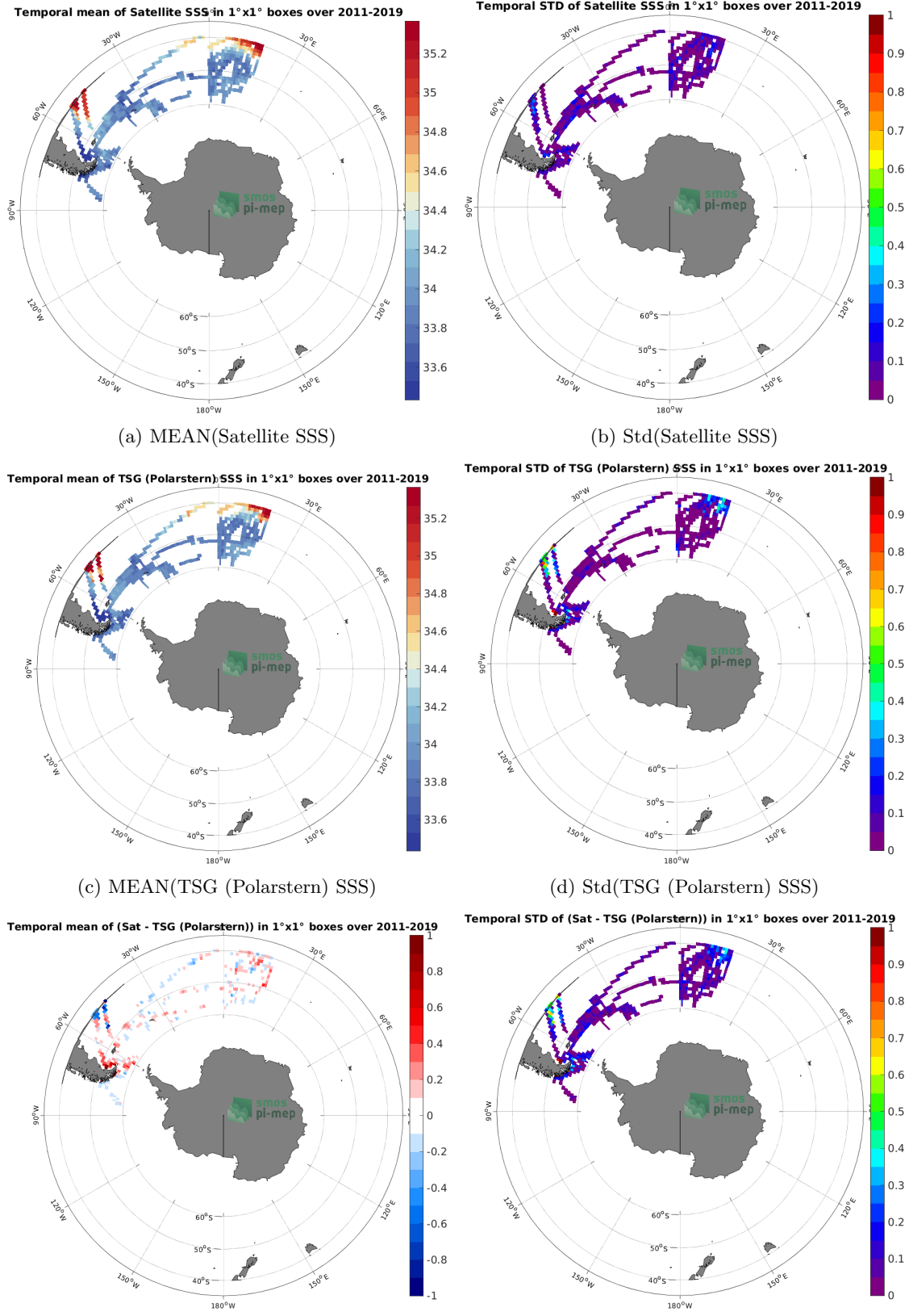
Figure 6: Temporal mean (left) and Std (right) of SSS from SMAP SSS L4 OI v1 - 7 Days (IPRC) (top), TSG (Polarstern) (middle), and of \Delta SSS (Satellite - TSG (Polarstern)). Only match-up pairs are used to generate these maps.
