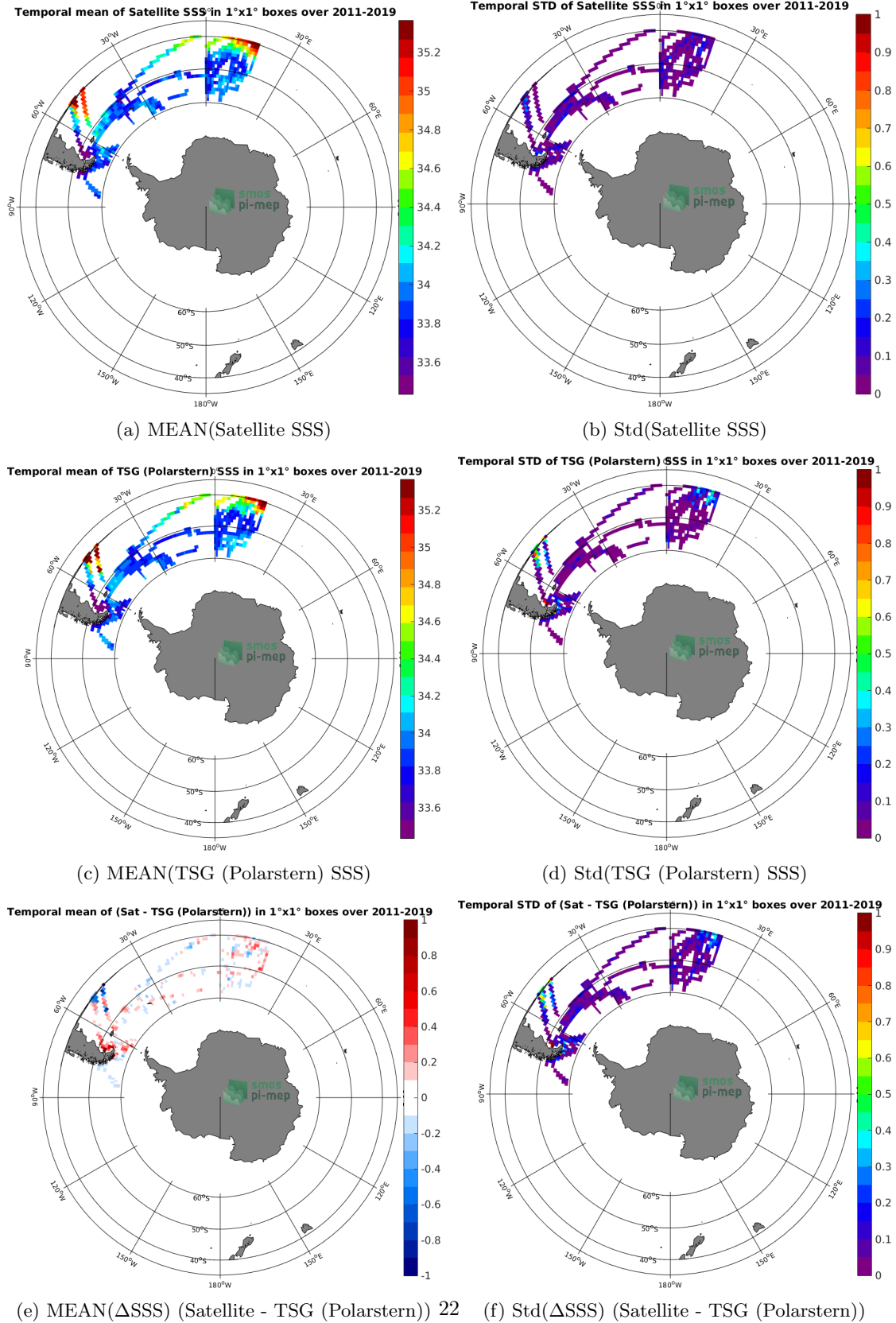
Figure 6: Temporal mean (left) and Std (right) of SSS from SMAP SSS L4 OI v1 - 7day (IPRC) (top), TSG (Polarstern) (middle), and of \Delta SSS (Satellite - TSG (Polarstern)). Only match-up pairs are used to generate these maps.
