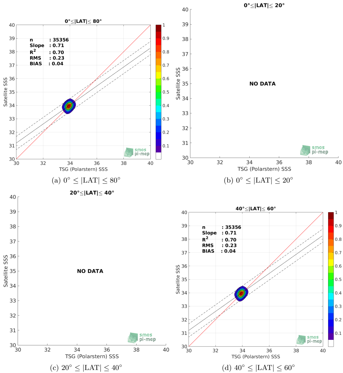
Figure 9: Contour maps of the concentration of SMAP SSS L4 OI v1 - 7day (IPRC) SSS (y-axis) versus TSG (Polarstern) SSS (x-axis) at match-up pairs for different latitude bands. For each plot, the red line shows x=y . The black thin and dashed lines indicate a linear fit through the data cloud and the \pm 95\% confidence levels, respectively. The number match-up pairs n , the slope and R^2 coefficient of the linear fit, the root mean square (RMS) and the mean bias between satellite and in situ data are indicated for each latitude band in each plots.
