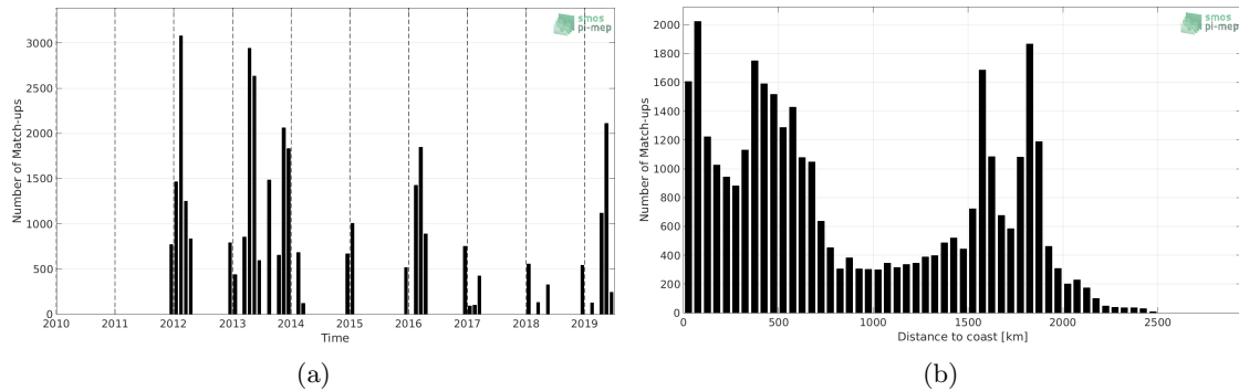
Figure 1: Number of match-ups between TSG (Polarstern) and SMAP SSS L4 OI v1 - 7day (IPRC) SSS as a function of time (a) and as function of the distance to coast (b) over the Roaring Forties and Furious Fifties Pi-MEP region and for the full satellite product period.
