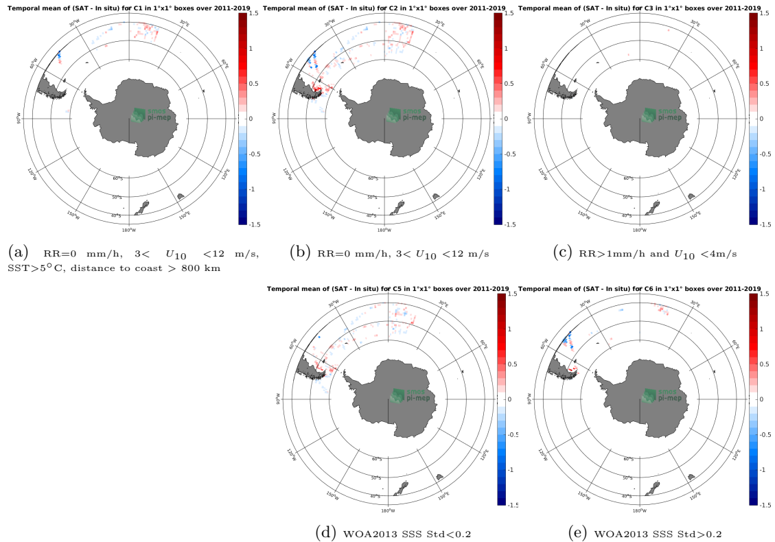
Figure 12: Temporal mean gridded over spatial boxes of size 1^{\circ}\times 1^{\circ} of \Delta\text{SSS} (SMAP SSS L4 OI v1 - 7day (IPRC) - TSG (Polarstern)) for 5 different subdatasets corresponding to:RR=0 mm/h, 3 < U_{10} < 12 m/s, SST >5^{\circ}\text{C} , distance to coast > 800 km (a), RR=0 mm/h, 3 < U_{10} < 12 m/s (b), RR >1 mm/h and U_{10} < 4 m/s (c), WOA2013 SSS Std <0.2 (d), WOA2013 SSS Std >0.2 (e).
