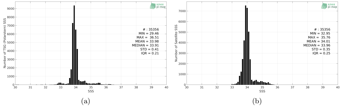
Figure 2: Histograms of SSS from TSG (Polarstern) (a) and SMAP SSS L4 OI v1 - 7day (IPRC) (b) considering all match-up pairs per bins of 0.1 over the Roaring Forties and Furious Fifties Pi-MEP region and for the full satellite product period.
