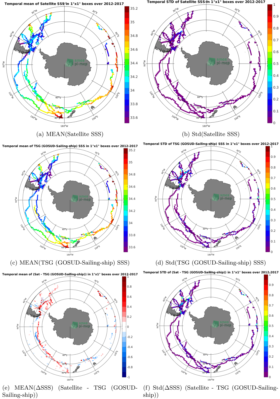
Figure 6: Temporal mean (left) and Std (right), of SSS from SMAP SSS L4 OI v1 - 7day (IPRC) (top), TSG (GOSUD-Sailing-ship) (middle), and of \Delta SSS (Satellite - TSG (GOSUD-Sailing-ship)). Only match-up pairs are used to generate these maps.
