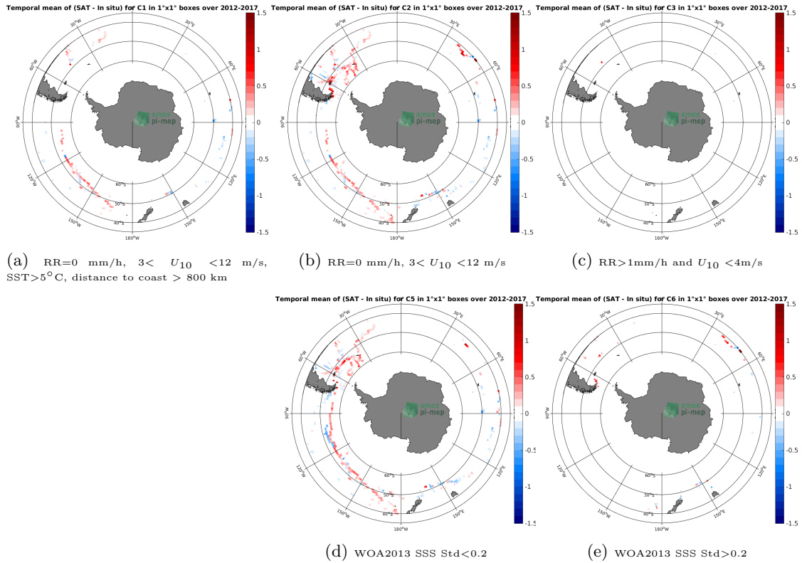
Figure 12: Temporal mean gridded over spatial boxes of size 1°x1° of \Delta SSS (SMAP SSS L4 OI v1 - 7day (IPRC) - TSG (GOSUD-Sailing-ship)) for 5 different subdatasets corresponding to: RR=0 mm/h, 3 < U_{10} < 12 m/s, SST>5°C, distance to coast > 800 km (a), RR=0 mm/h, 3 < U_{10} < 12 m/s (b), RR>1mm/h and U_{10} < 4 m/s (c), WOA2013 SSS Std<0.2 (d), WOA2013 SSS Std>0.2 (e).
