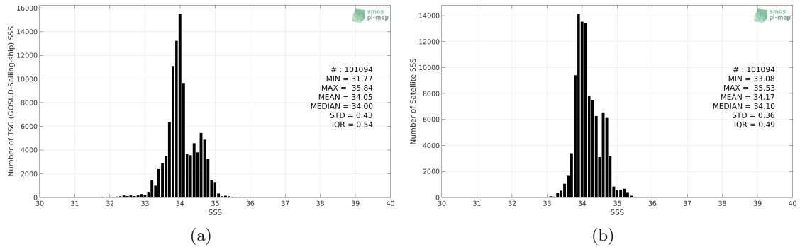
Figure 2: Histograms of SSS from TSG (GOSUD-Sailing-ship) (a) and SMAP SSS L4 OI v1 - 7day (IPRC) (b) considering all match-up pairs per bins of 0.1 over the Roaring Forties and Furious Fifties Pi-MEP region and for the full satellite product period.
