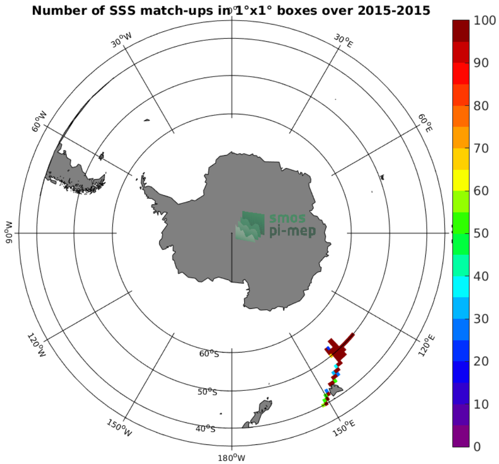
Figure 4: Number of SSS match-ups between TSG (GOSUD-Research-vessel) SSS and the SMAP SSS L4 OI v1 - 7day (IPRC) SSS product for the Roaring Forties and Furious Fifties Pi-MEP region over 1^\circ \times 1^\circ boxes and for the full satellite product period.
