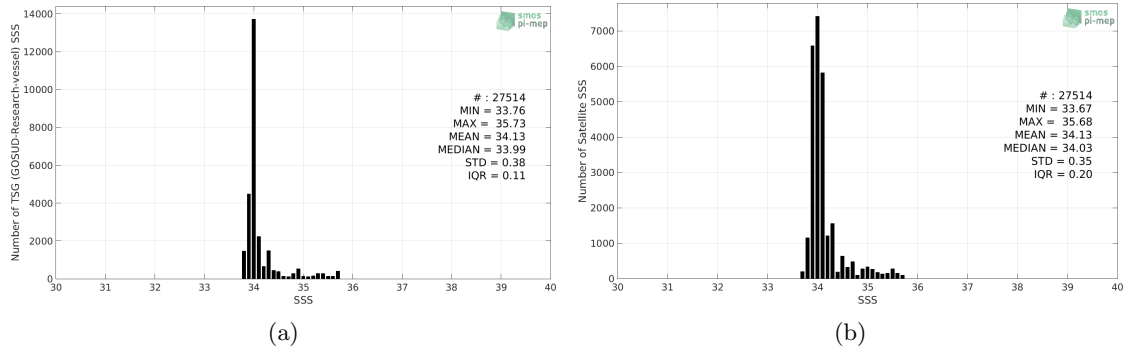
Figure 2: Histograms of SSS from TSG (GOSUD-Research-vessel) (a) and SMAP SSS L4 OI v1 - 7day (IPRC) (b) considering all match-up pairs per bins of 0.1 over the Roaring Forties and Furious Fifties Pi-MEP region and for the full satellite product period.
