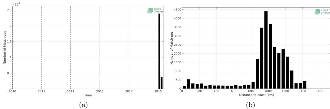
Figure 1: Number of match-ups between TSG (GOSUD-Research-vessel) and SMAP SSS L4 OI v1 - 7day (IPRC) SSS as a function of time (a) and as function of the distance to coast (b) over the Roaring Forties and Furious Fifties Pi-MEP region and for the full satellite product period.
