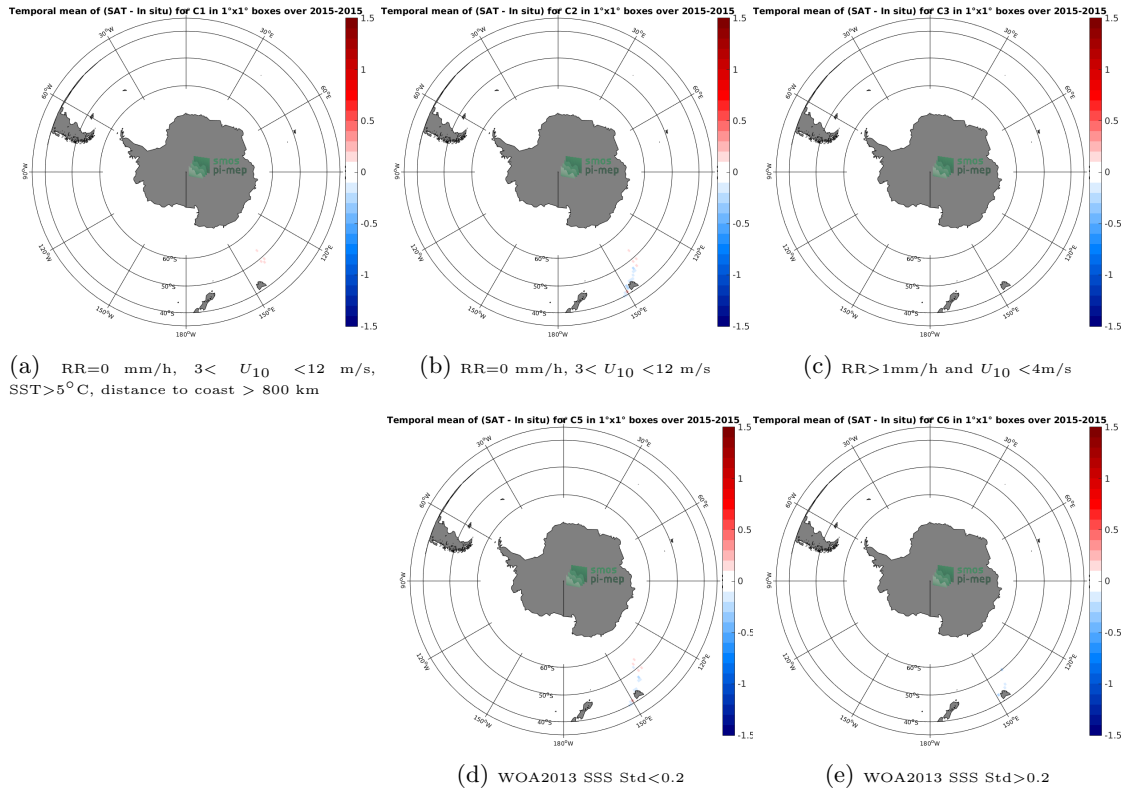
Figure 12: Temporal mean gridded over spatial boxes of size 1°x1° of \Delta SSS (SMAP SSS L4 OI v1 - 7day (IPRC) - TSG (GOSUD-Research-vessel)) for 5 different subdatasets corresponding to:RR=0 mm/h, 3 < U_{10} < 12 m/s, SST>5°C, distance to coast > 800 km (a), RR=0 mm/h, 3 < U_{10} < 12 m/s (b), RR>1mm/h and U_{10} < 4 m/s (c), WOA2013 SSS Std<0.2 (d), WOA2013 SSS Std>0.2 (e).
