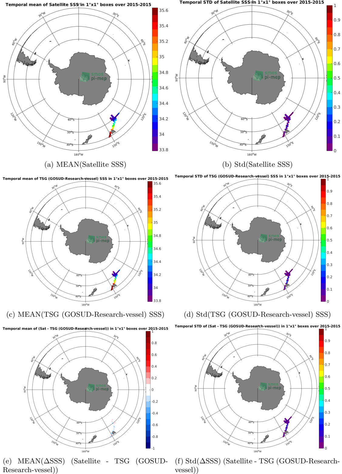
Figure 6: Temporal mean (left) and Std (right) of SSS from SMAP SSS L4 OI v1 - 7day (IPRC) (top), TSG (GOSUD-Research-vessel) (middle), and of \Delta SSS (Satellite - TSG (GOSUD-Research-vessel)). Only match-up pairs are used to generate these maps.
