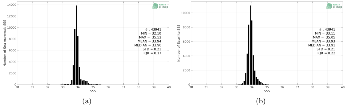
Figure 2: Histograms of SSS from Marine mammals (a) and SMAP SSS L4 OI v1 - 7 Days (IPRC) (b) considering all match-up pairs per bins of 0.1 over the Roaring Forties and Furious Fifties Pi-MEP region and for the full satellite product period.
