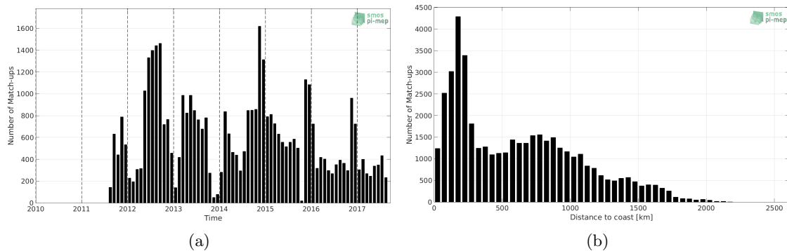
Figure 1: Number of match-ups between Marine mammals and SMAP SSS L4 OI v1 - 7 Days (IPRC) SSS as a function of time (a) and as function of the distance to coast (b) over the Roaring Forties and Furious Fifties Pi-MEP region and for the full satellite product period.
