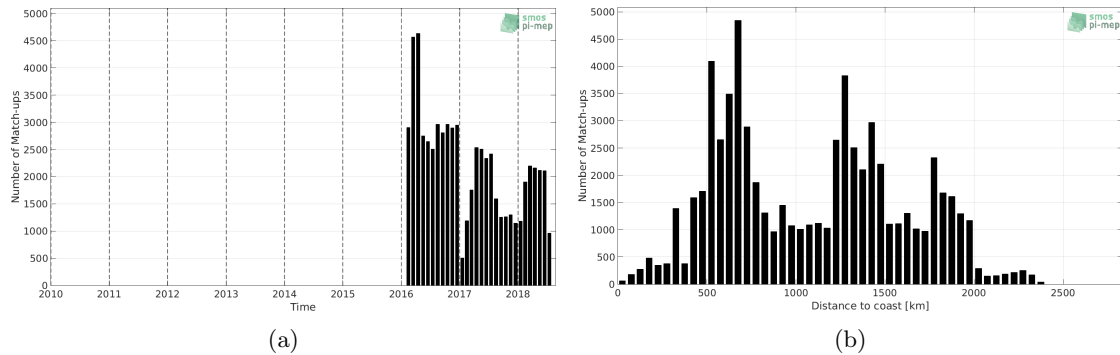
Figure 1: Number of match-ups between Surface drifters and SMAP SSS L4 OI v1 - 7day (IPRC) SSS as a function of time (a) and as function of the distance to coast (b) over the Roaring Forties and Furious Fifties Pi-MEP region and for the full satellite product period.
