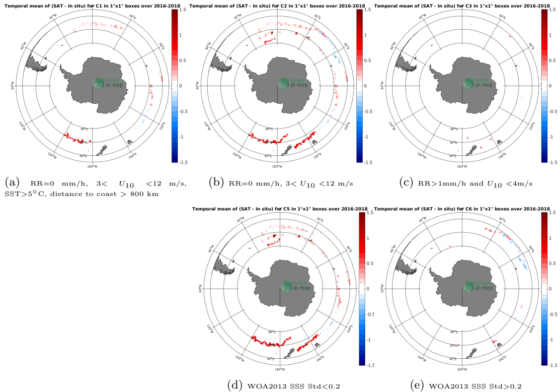
Figure 11: Temporal mean gridded over spatial boxes of size 1^{\circ}\times 1^{\circ} of \Delta\text{SSS} (SMAP SSS L4 OI v1 - 7day (IPRC) - Surface drifters) for 5 different subdatasets corresponding to:RR=0 mm/h, 3 < U_{10} < 12 m/s, SST >5^{\circ}\text{C} , distance to coast > 800 km (a), RR=0 mm/h, 3 < U_{10} < 12 m/s (b), RR >1 mm/h and U_{10} < 4 m/s (c), WOA2013 SSS Std <0.2 (d), WOA2013 SSS Std >0.2 (e).
