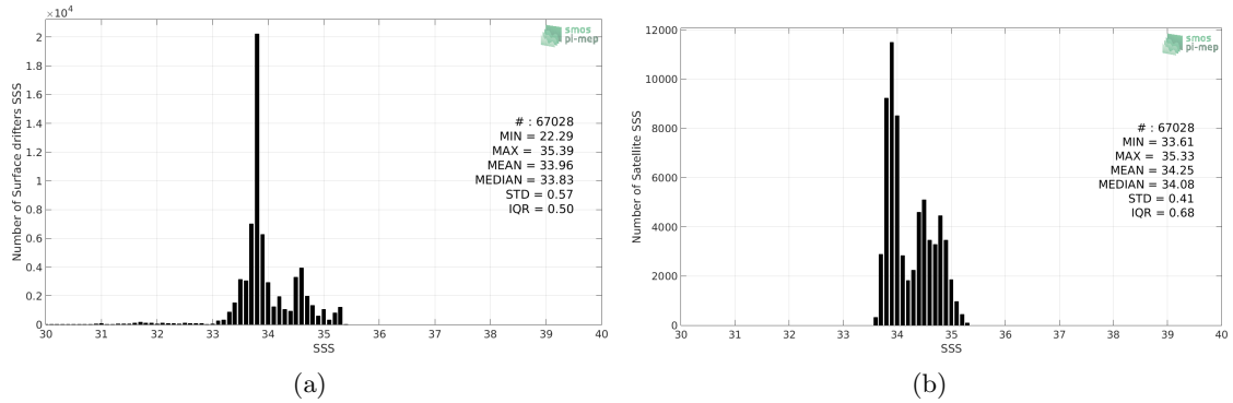
Figure 2: Histograms of SSS from Surface drifters (a) and SMAP SSS L4 OI v1 - 7day (IPRC) (b) considering all match-up pairs per bins of 0.1 over the Roaring Forties and Furious Fifties Pi-MEP region and for the full satellite product period.
