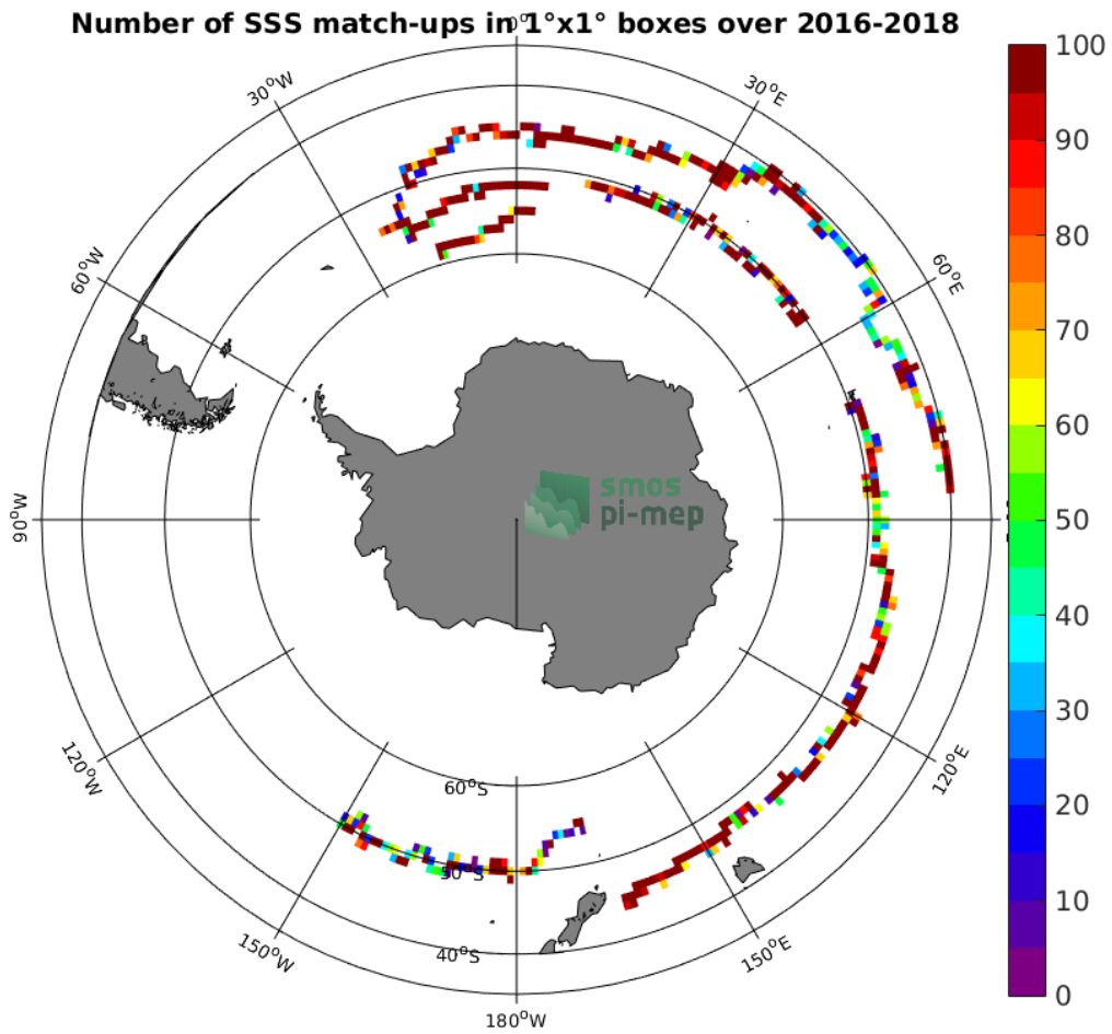
Figure 3: Number of SSS match-ups between Surface drifters SSS and the SMAP SSS L4 OI v1 - 7day (IPRC) SSS product for the Roaring Forties and Furious Fifties Pi-MEP region over 1^\circ \times 1^\circ boxes and for the full satellite product period.
