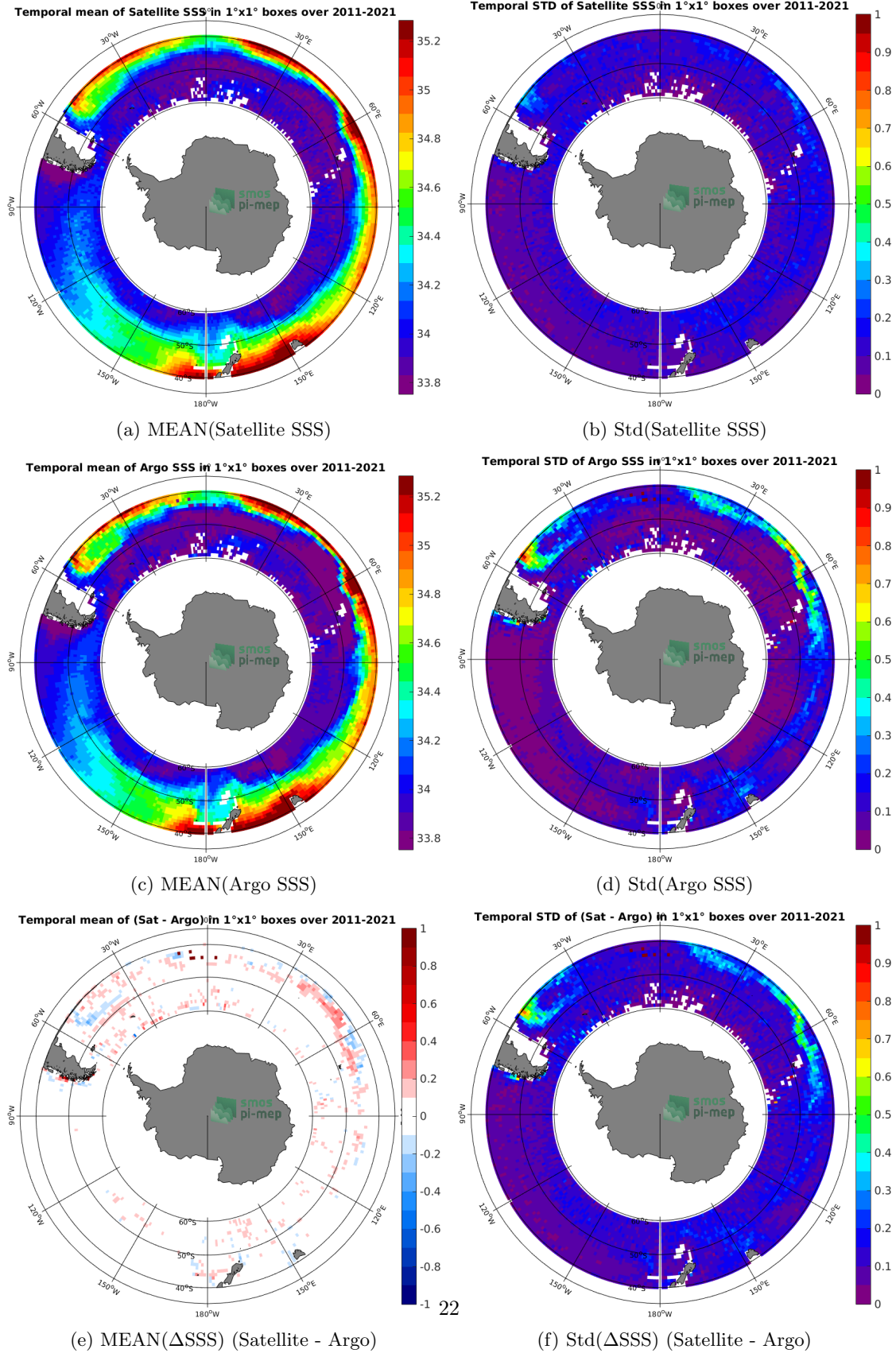
Figure 6: Temporal mean (left) and Std (right) of SSS from SMAP SSS L4 OI v1 - 7 Days (IPRC) (top), Argo (middle), and of \Delta SSS (Satellite - Argo). Only match-up pairs are used to generate these maps.
