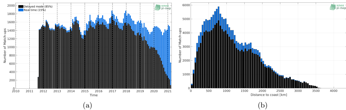
Figure 1: Number of match-ups between Argo and SMAP SSS L4 OI v1 - 7 Days (IPRC) SSS as a function of time (a) and as function of the distance to coast (b) over the Roaring Forties and Furious Fifties Pi-MEP region and for the full satellite product period.
