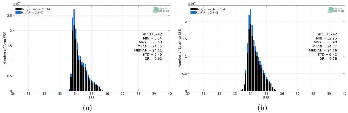
Figure 2: Histograms of SSS from Argo (a) and SMAP SSS L4 OI v1 - 7 Days (IPRC) (b) considering all match-up pairs per bins of 0.1 over the Roaring Forties and Furious Fifties Pi-MEP region and for the full satellite product period.
