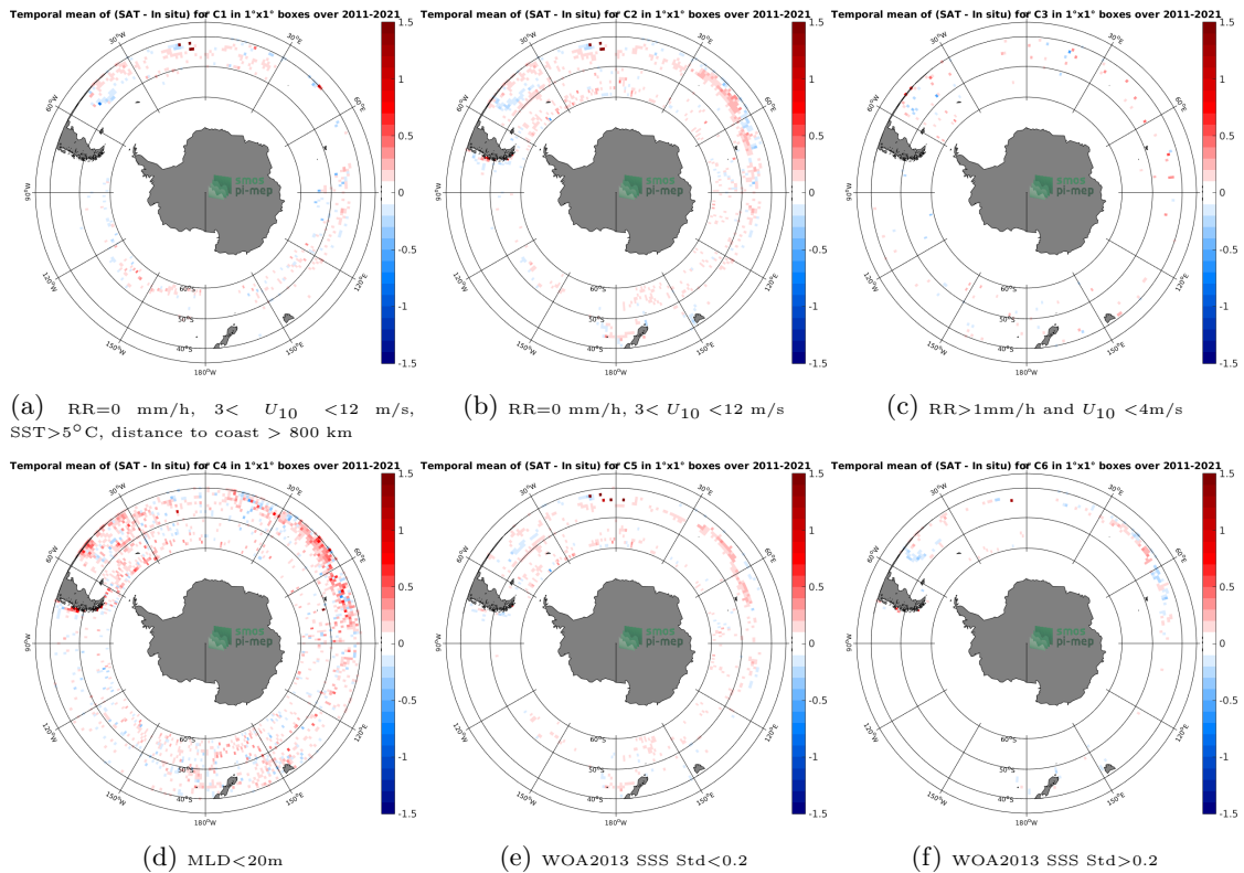
Figure 12: Temporal mean gridded over spatial boxes of size 1^{\circ}\times 1^{\circ} of \Delta\text{SSS} (SMAP SSS L4 OI v1 - 7 Days (IPRC) - Argo) for 6 different subdatasets corresponding to:RR=0 mm/h, 3 < U_{10} < 12 m/s, SST >5^{\circ}\text{C} , distance to coast > 800 km (a), RR=0 mm/h, 3 < U_{10} < 12 m/s (b), RR >1 mm/h and U_{10} < 4 m/s (c),MLD <20 m (d),WOA2013 SSS Std <0.2 (e),WOA2013 SSS Std >0.2 (f).
