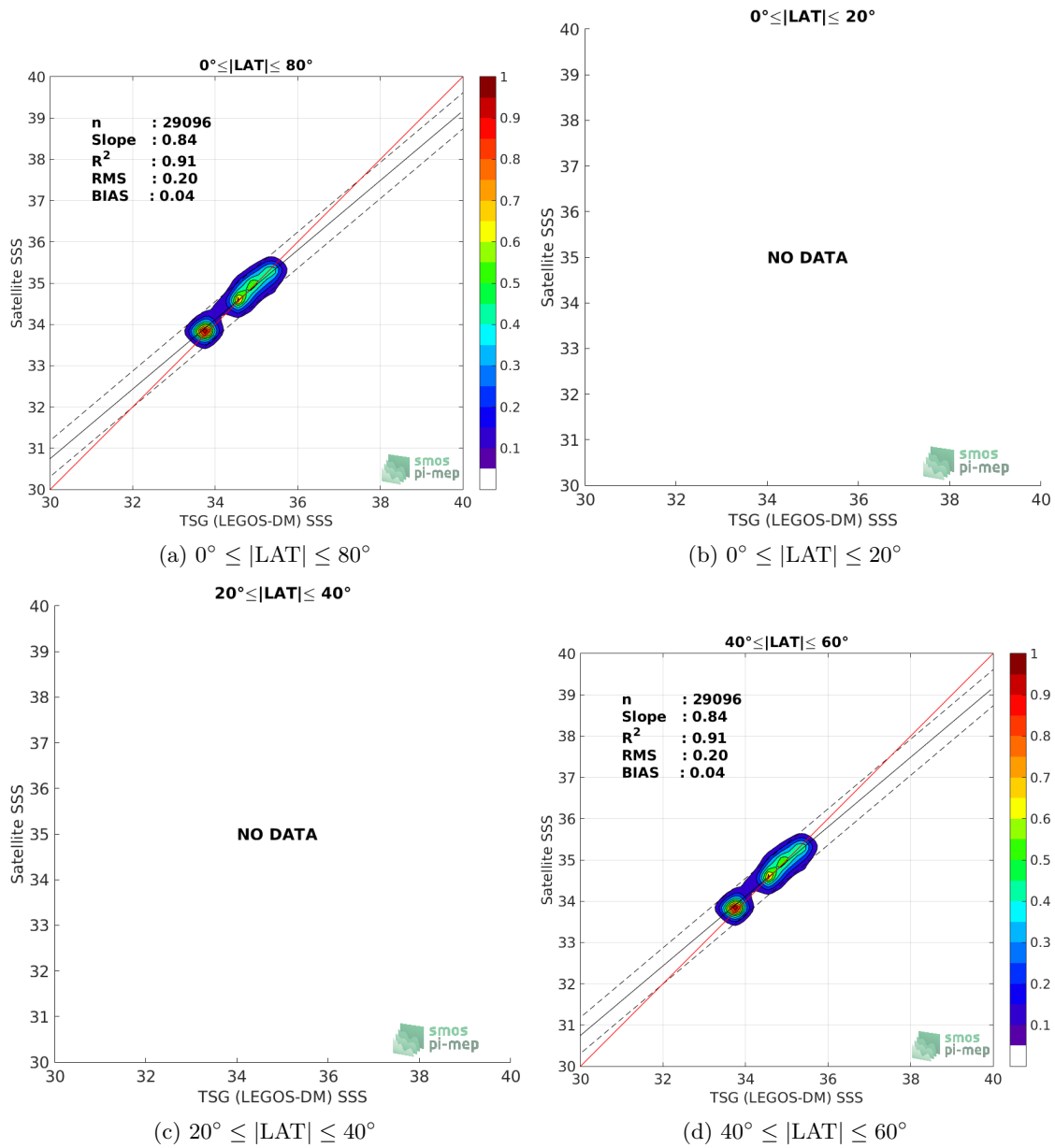
Figure 9: Contour maps of the concentration of SMAP SSS L4 OI v1 - Monthly (IPRC) SSS (y-axis) versus TSG (LEGOS-DM) SSS (x-axis) at match-up pairs for different latitude bands. For each plot, the red line shows x=y . The black thin and dashed lines indicate a linear fit through the data cloud and the \pm 95\% confidence levels, respectively. The number match-up pairs n , the slope and R^2 coefficient of the linear fit, the root mean square (RMS) and the mean bias between satellite and in situ data are indicated for each latitude band in each plots.
