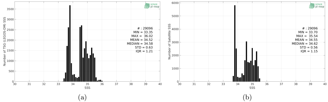
Figure 2: Histograms of SSS from TSG (LEGOS-DM) (a) and SMAP SSS L4 OI v1 - Monthly (IPRC) (b) considering all match-up pairs per bins of 0.1 over the Roaring Forties and Furious Fifties Pi-MEP region and for the full satellite product period.
