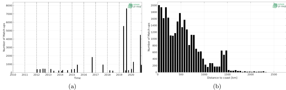
Figure 1: Number of match-ups between TSG (LEGOS-DM) and SMAP SSS L4 OI v1 - Monthly (IPRC) SSS as a function of time (a) and as function of the distance to coast (b) over the Roaring Forties and Furious Fifties Pi-MEP region and for the full satellite product period.
