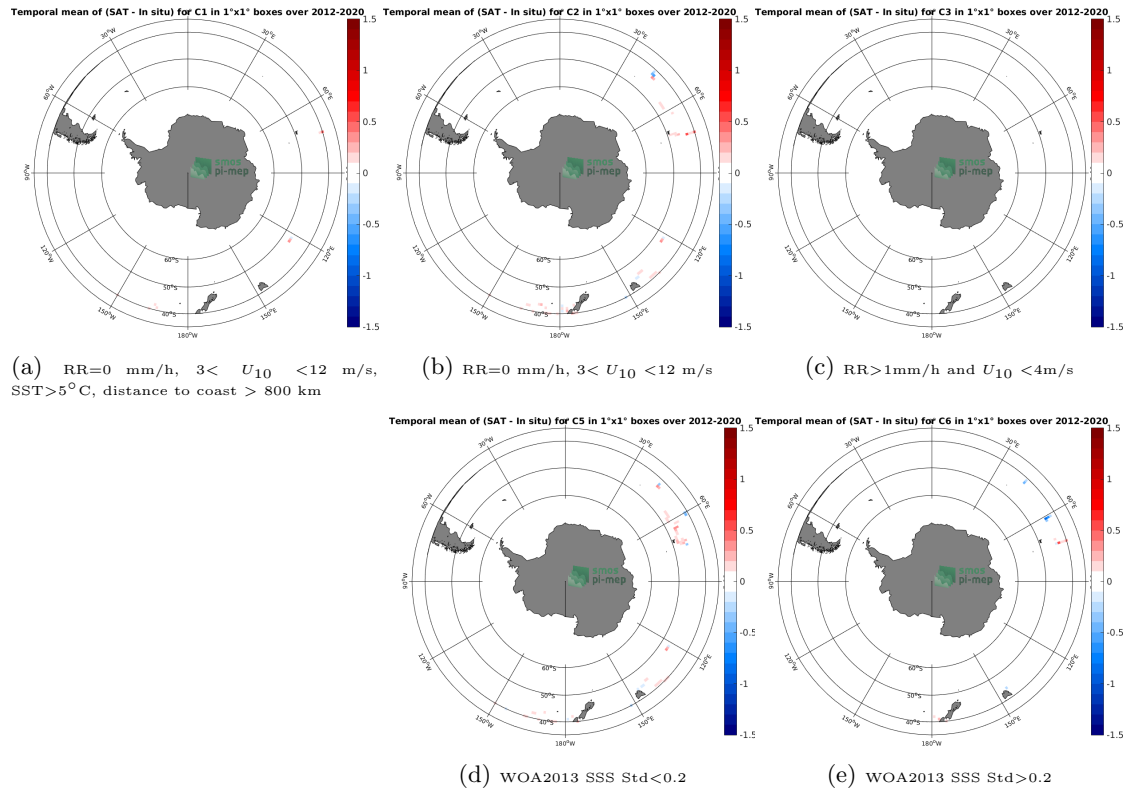
Figure 12: Temporal mean gridded over spatial boxes of size 1^{\circ}\times 1^{\circ} of \Delta\text{SSS} (SMAP SSS L4 OI v1 - Monthly (IPRC) - TSG (LEGOS-DM)) for 5 different subdatasets corresponding to: RR=0 mm/h, 3 < U_{10} < 12 m/s, SST > 5^{\circ}\text{C} , distance to coast > 800 km (a), RR=0 mm/h, 3 < U_{10} < 12 m/s (b), RR > 1 mm/h and U_{10} < 4 m/s (c), WOA2013 SSS Std < 0.2 (d), WOA2013 SSS Std > 0.2 (e).
