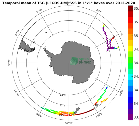
(c) MEAN(TSG (LEGOS-DM) SSS)
