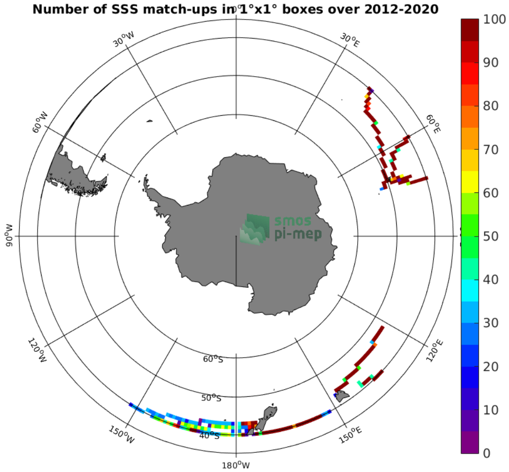
Figure 4: Number of SSS match-ups between TSG (LEGOS-DM) SSS and the SMAP SSS L4 OI v1 - Monthly (IPRC) SSS product for the Roaring Forties and Furious Fifties Pi-MEP region over 1^{\circ} \times 1^{\circ} boxes and for the full satellite product period.
